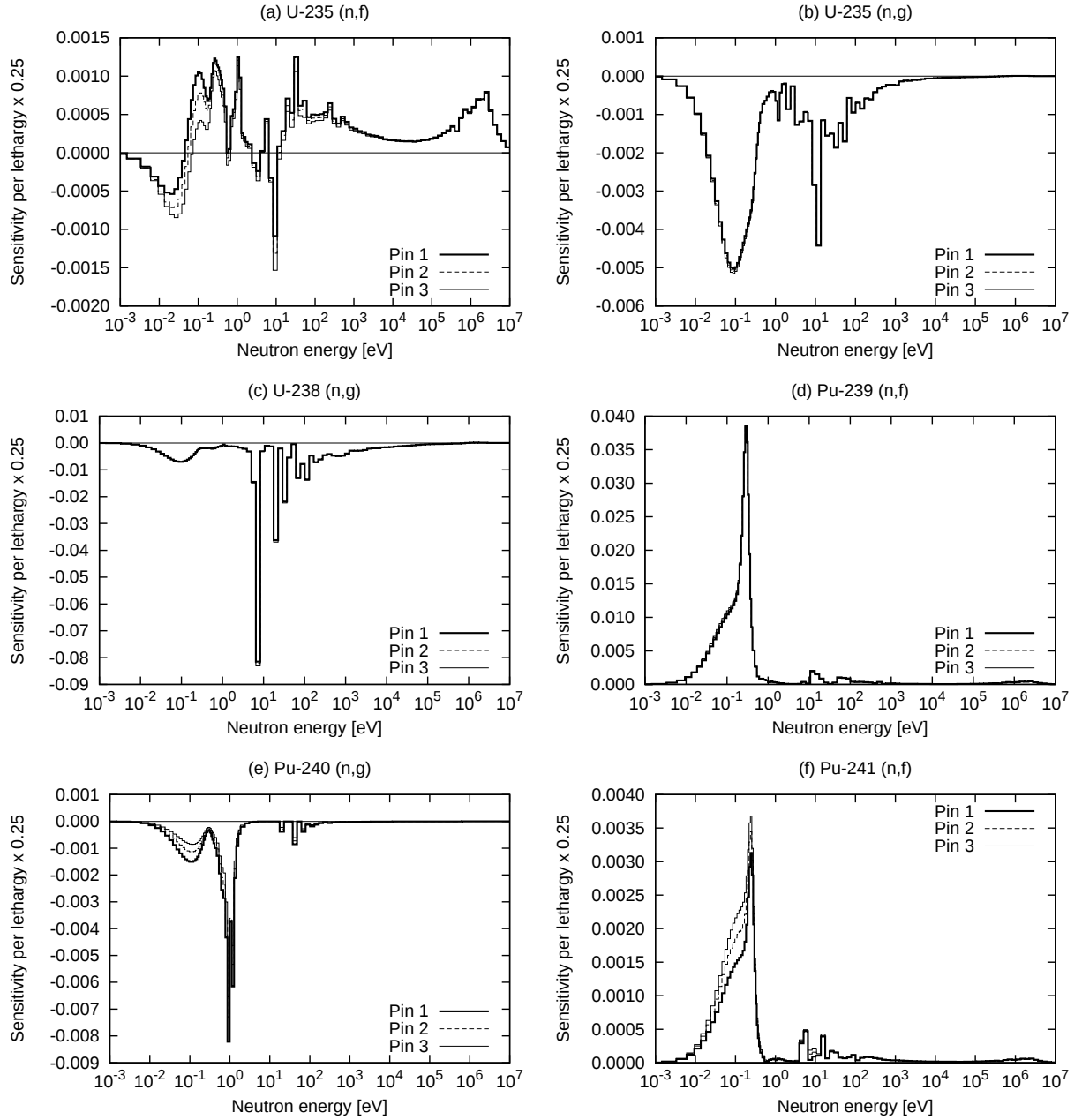
Figure 9: Sensitivities of gadolinium-156 number densities after fuel depletion to several cross sections in a 5 \times 5 multi-cell problem
