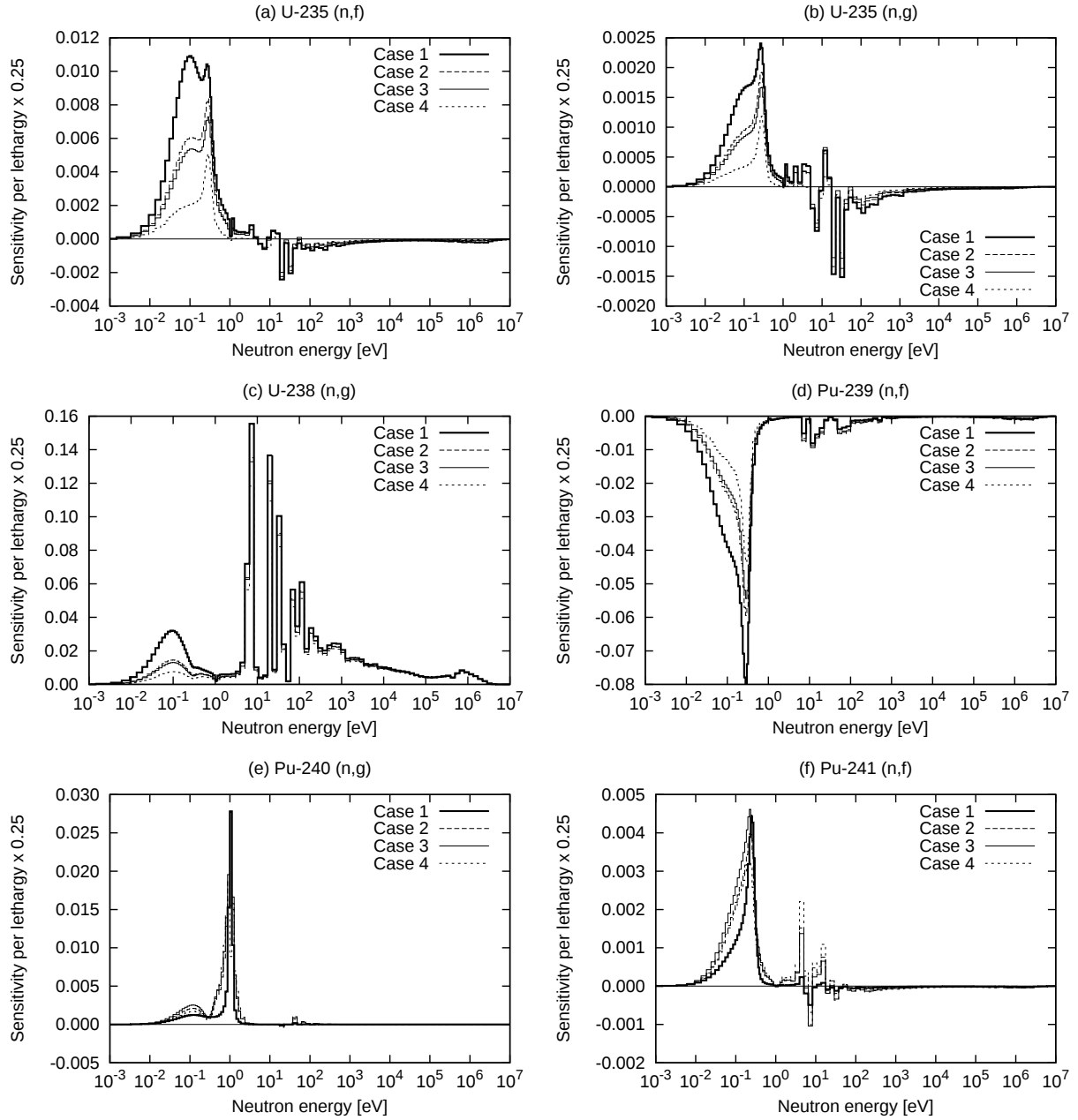
Figure 7: Sensitivities of plutonium-239 number densities after fuel depletion to several cross sections in a 3×3 multi-cell problem
