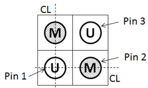
Figure 1: 3×3 multi-cell problem for verification calculations. “U” and “M” stand for UO 2 and MOX fuel cells, respectively.
