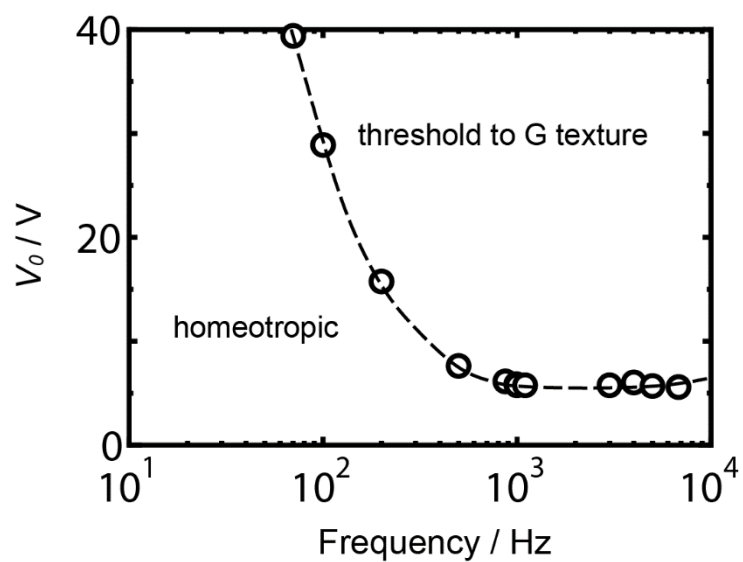
Figure 4. A dependence of the threshold voltage for a sample containing 0.1 wt% of RM257. The open symbols show the data showing the G pattern. The dashed curve is a guide to eyes. The cell thickness is 4.4 \mu\text{m} . The polymerization is made at V_0=26.2 V, 100 Hz.
