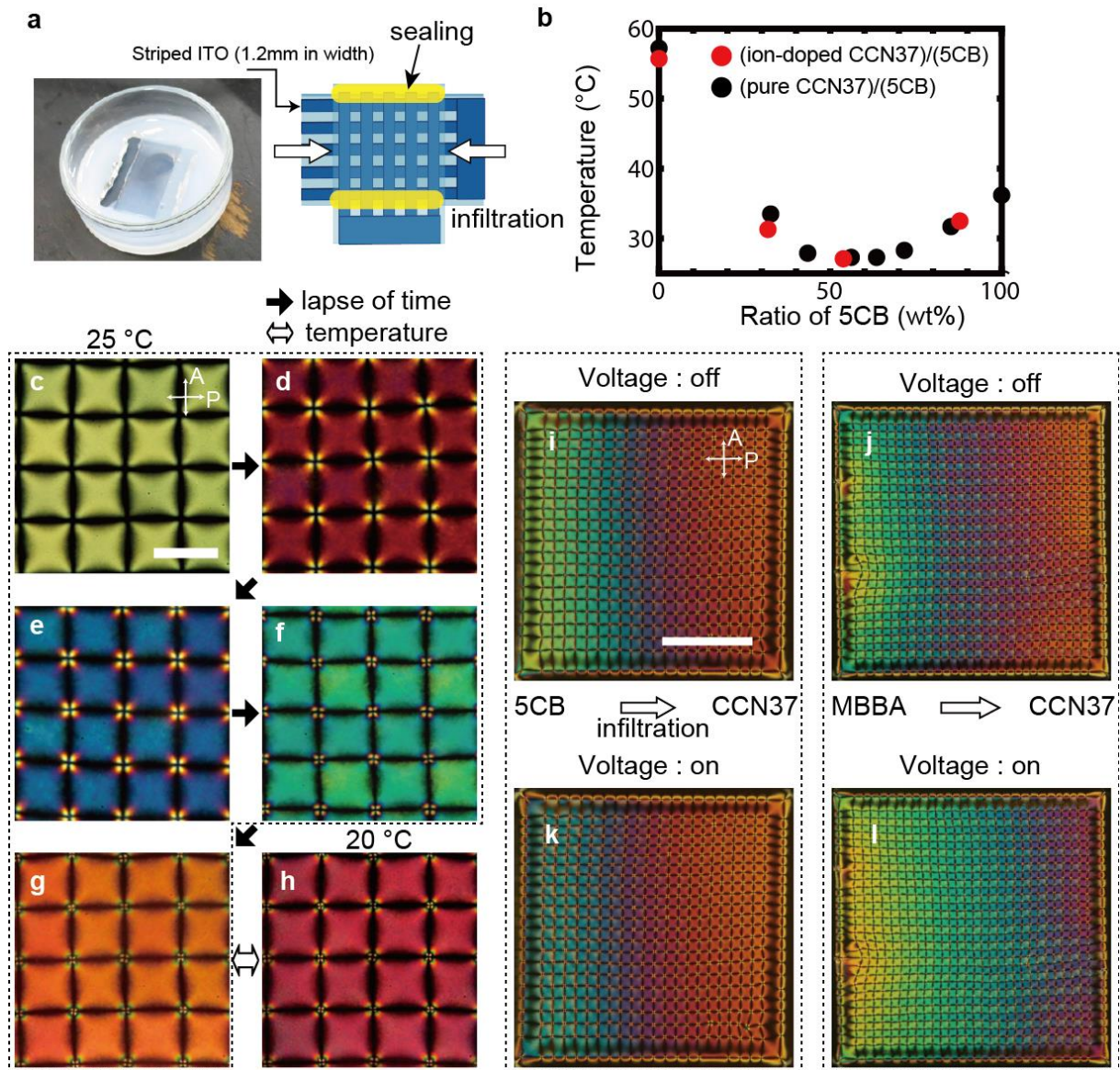
Figure 2. a) Schematic illustration of immersion experiment. b) Transition temperature to the isotropic phase of CCN-37/5CB mixtures. Black circles are for pure CCN-37. Red circles are for CCN-37 containing 1 wt% of TBABE. c)-g) Enlarged views of color alternation during time course as a result of immersion with 5CB. We note that the images c)-g) are taken at different locations of a cell because the process takes time (typically around a month). h) Enhanced retardation by decreasing temperature from g). i), j) POM images as a result of infiltration by 5CB and MBBA from left to right. RM257 concentration is 3.3 wt% for i) and 1.6 wt% for j). G-texture is polymerized at V_0=26.2 V. f is 50 Hz for i) and 90 Hz for j). k), l) POM images under the electric voltages of V_0=26.2 V, f=10 KHz.
