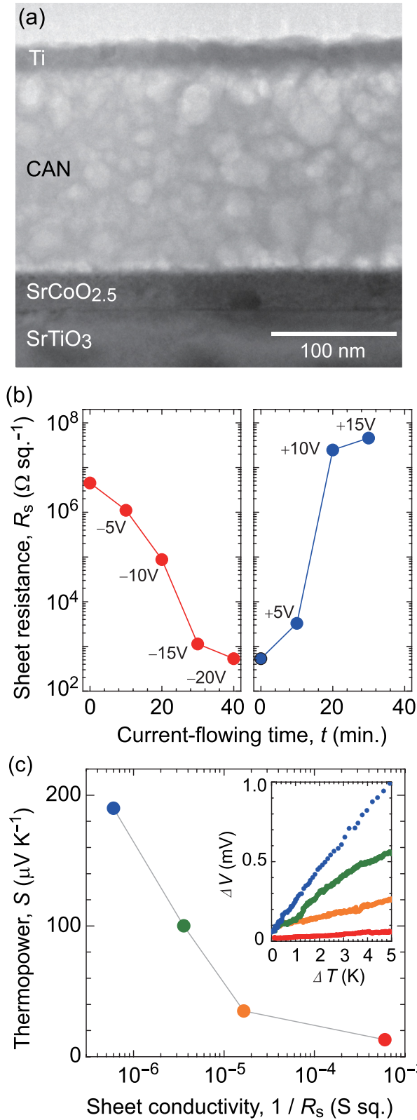
FIG. 2. (a) Cross-sectional TEM image of the SrCoO x TFT with leakage-free water. The trilayer structure composed of SrCoO 2.5 (30 nm), CAN (160 nm), and Ti (20 nm) layers is clearly seen. Many light spots in the CAN layer indicate nanopores, which are fully occupied with water. (b) R_s vs. current-flowing time ( t ) of applied V_g for the SrCoO x layer. The R_s was measured after the V_g application, where negative V_g up to -20 V was applied for oxidation (left panel) and positive V_g up to +15 V was applied for reduction (right panel) of the SrCoO x layer. The V_g application time was 10 min at each step. (c) S vs. 1/R_s at RT. \Delta V - \Delta T plots are shown in the inset.
