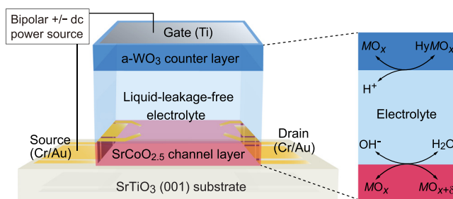
FIG. 1. A schematic of three-terminal TFT structure consisting of a \text{SrCoO}_{2.5} channel layer, a liquid-leakage-free electrolyte as a gate insulator, an \text{a-WO}_3 counter layer, and a Ti gate electrode on a \text{SrTiO}_3 (001) substrate. Cr/Au bilayer films were used for source-drain electrodes. The right figure illustrates the electrochemical reaction in the device during the gate voltage application.
