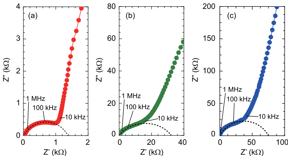
FIG. 4. Cole-Cole plots of 300-nm-thick \text{a-Na}_x\text{TaO}_3 films ( 950 \mu\text{m} \times 800 \mu\text{m} ) with x = 1.0 (a), 0.1 (b), and 0.01 (c), measured at RT in air. The dotted lines are fitting curves by using the equivalent circuit model composed of the constant phase element and ionic resistance in parallel.
