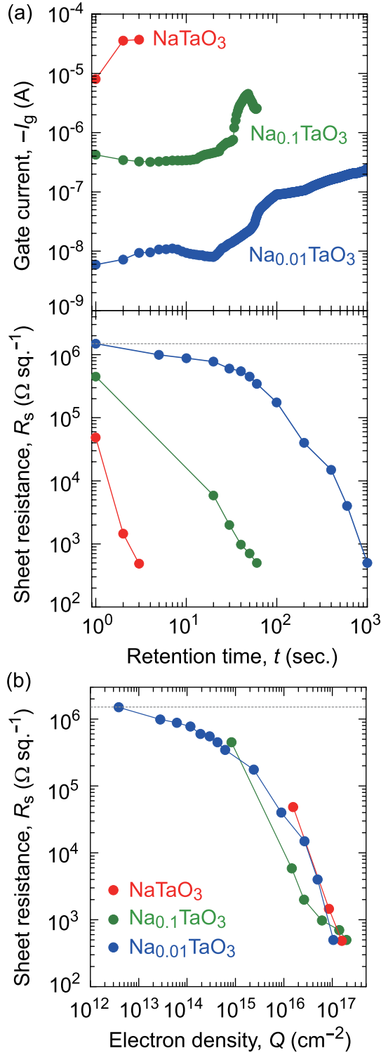
FIG. 5. (a) Current-flowing time ( t ) dependence of I_g (upper panel) and R_s (lower panel) for the \text{SrCoO}_x TFT with a \text{a-Na}_x\text{TaO}_3 ( x = 0.01, 0.1 , and 1.0 ) leakage-free electrolyte under the application of V_g = -3 V. The I_g and R_s were, respectively, measured during and after the V_g application. The dotted lines indicate the R_s of the virgin \text{SrCoO}_{2.5} layer. (b) Electron-density ( Q ) dependence of R_s under the V_g application. The Q was calculated as the integrated value of the I_g - t plots in (a).
