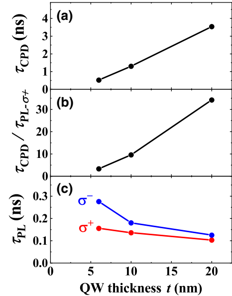
FIG. 3. Time constants (a) \tau_{\text{CPD}} , (b) \tau_{\text{CPD}}/\tau_{\text{PL-}\sigma^+} , and (c) \tau_{\text{PL-}\sigma^\pm} of the circularly polarized QD ES PL, where \tau_{\text{CPD}} is the CPD decay time and \tau_{\text{PL-}\sigma^\pm} are the PL decay times of the \sigma^\pm polarizations, as a function of the QW thickness t .
