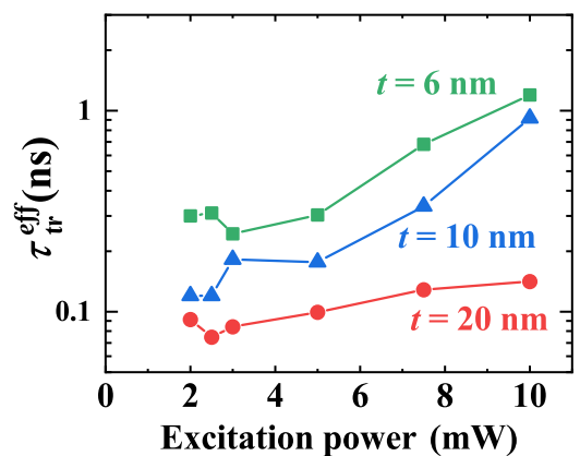
FIG. 6. Effective spin transfer time \tau_{tr}^{eff} as a function of the excitation power for various QW thicknesses t = 6 nm (green squares), 10 nm (blue triangles), and 20 nm (red circles).
