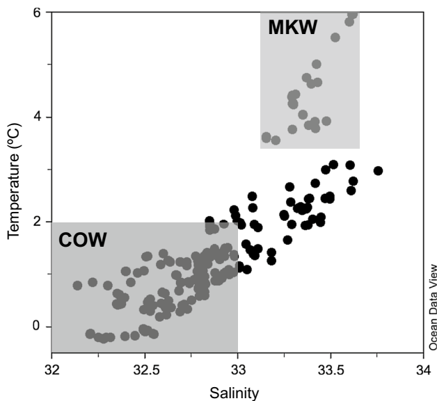
Fig. 4 Temperature–salinity ( T–S ) diagram for seawater samples collected from the upper 250 m at all stations included in this study. The shaded locations correspond to the Coastal Oyashio Water (COW) and the modified Kuroshio Water (MKW)
