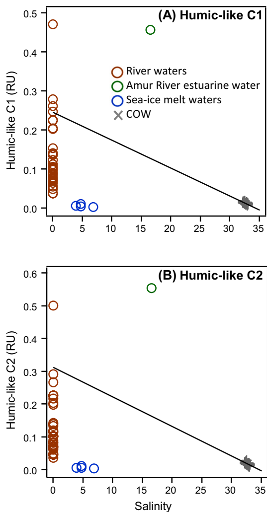
Fig. 8a–b Scatter plots of humic-like C1 ( a ) and humic-like C2 ( b ) against salinity for the Coastal Oyashio Water (COW) and its possible end-members (river water, the Amur River estuarine water, and sea-ice melt water). The line in each panel is the linear regression between the humic-like component and salinity determined using the COW samples
