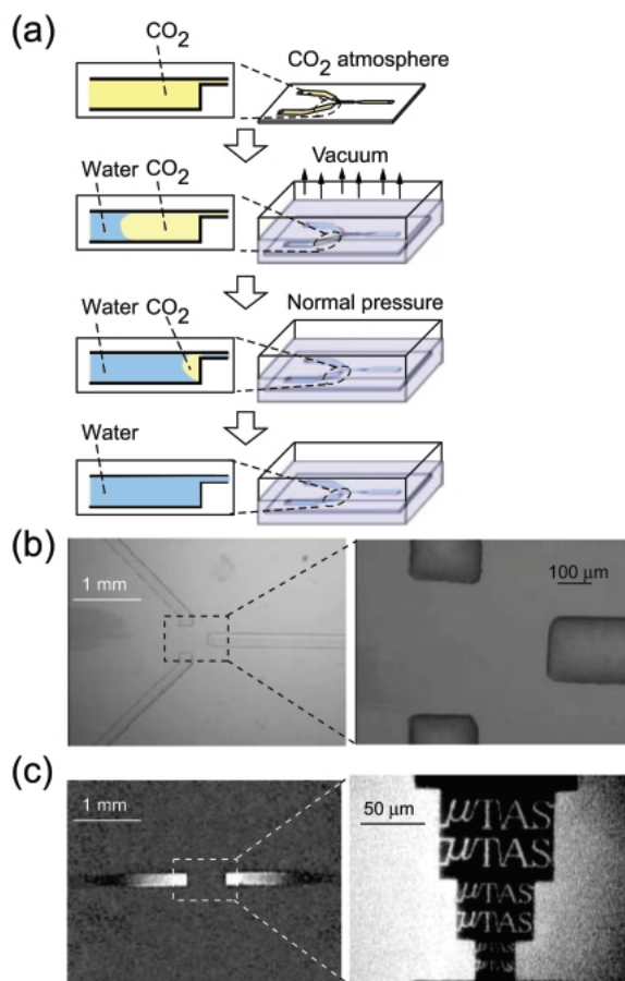
Fig. 5 (a) Schematic illustration of the liquid introduction method utilizing reduced pressure and high solubility of CO 2 . (b) Results of liquid introduction into the Y-shaped nano chemical reactor. Water filled the microchannels and the nanochannel. (c) Results of liquid introduction into the complicated nanochannels. The white areas correspond to fluorescent aqueous solution. All patterns were filled with the solution.
