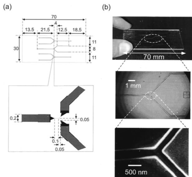
Fig. 1 (a) Layout of the nano chemical reactor. The depths of the gray pattern and black pattern were 40 \mu\text{m} and 400 nm, respectively. The numbers in this figure are “mm”. (b) The top two pictures are optical micrographs of the nano chemical reactor, and the bottom picture is an electron micrograph of it.
