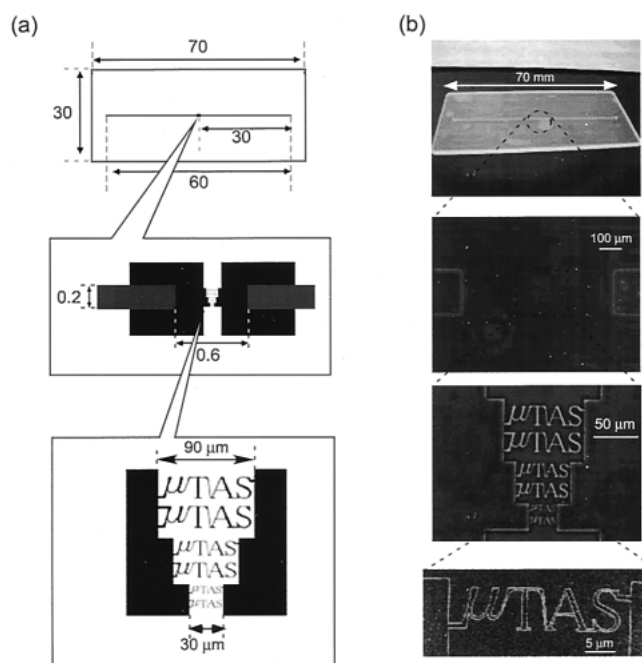
Fig. 2 (a) Layout of the complicated nano channels. The depths of the gray pattern and black pattern were 50 \mu\text{m} and 250 nm, respectively. (b) The top picture is a photograph of the chip. The middle two pictures are optical micrographs and the bottom picture is an SEM image of the complicated nanochannels connected to the microchannels for liquid introduction.
