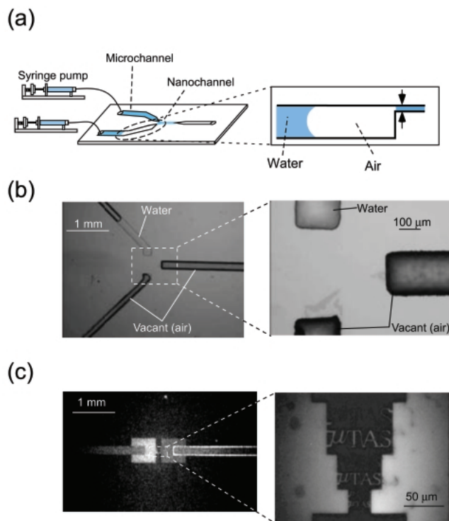
Fig. 3 (a) Illustration of liquid introduction by syringe pumps. (b) Results of liquid introduction into the Y-shaped nano chemical reactor. Water was introduced from the upper microchannel. Air remained in the nanochannel and microchannels. (c) Result of liquid introduction into the complicated nanochannels. The white area corresponds to fluorescent aqueous solution while the black area corresponds to an empty channel.
