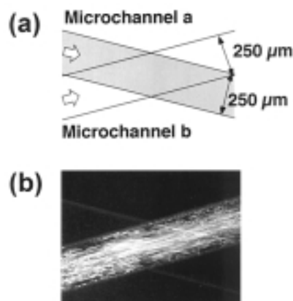
Fig. 6 (a) Illustration of the crossing region. (b) Fluorescent image of probe particles dispersed in the aqueous phase.
