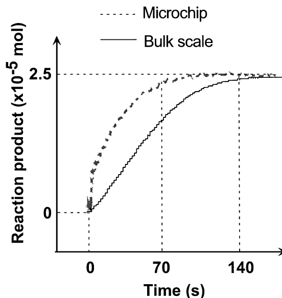
Fig. 1 Time courses of the reaction in the microchip and cuvette. The concentrations of HRP, TOOS, 4AA and \text{H}_2\text{O}_2 were 0.005 units/ml, 500 \mu M, 500 \mu M and 25 \mu M, respectively.
