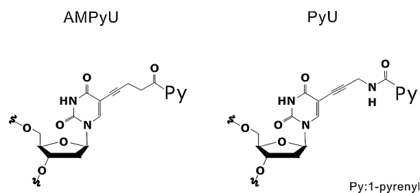
Figure 2. Structure of the BDF nucleosides, AMPyU and PyU.
