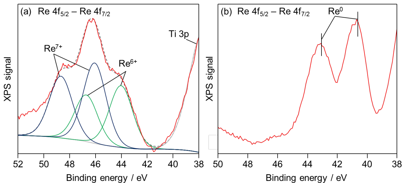
Figure 1. XPS spectra of the Re 4f region of \text{Re}/\text{TiO}_2 (a) before and (b) after the reduction with \text{H}_2 at T = 700^\circ\text{C} . Red line: raw spectra; dark gray line (dashed): total; pale gray line: Ti 3p; green line: \text{Re}^{6+} ; navy blue line: \text{Re}^{7+} .
