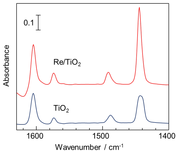
Figure 2. Ring-stretching region of the FT-IR spectra of pyridine adsorbed on \text{Re}/\text{TiO}_2 and \text{TiO}_2 after the \text{H}_2 reduction. Measurements were carried out at T = 100^\circ\text{C} under a He flow.
