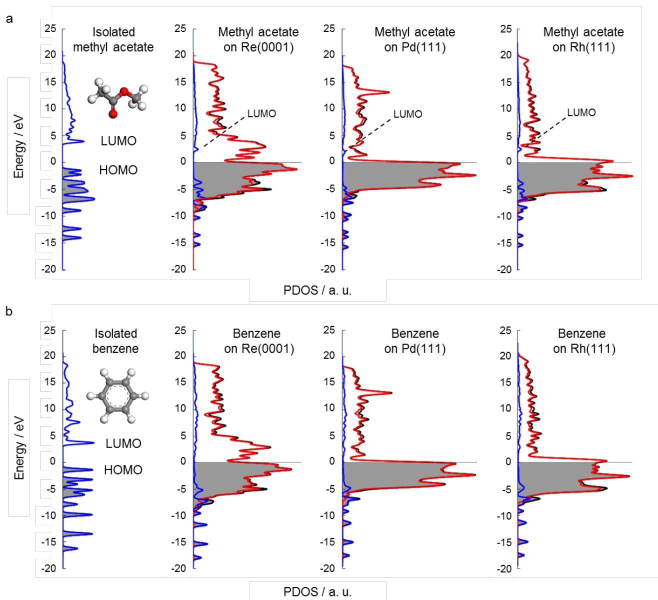
Figure 4. PDOSs of (a) isolated methyl acetate and methyl acetate adsorbed on the Re(0001), Pd(111), and Rh(111) surfaces; (b) isolated benzene and benzene adsorbed on the Re(0001), Pd(111), and Rh(111) surfaces; black line: total PDOS; blue line: PDOS of the adsorbates; red line: PDOS of the slabs; in all plots: E_F = 0 . The PDOS calculations for isolated methyl acetate and benzene were performed by placing the molecules at the center of the vacuum space on top of the Re(0001) slab.
