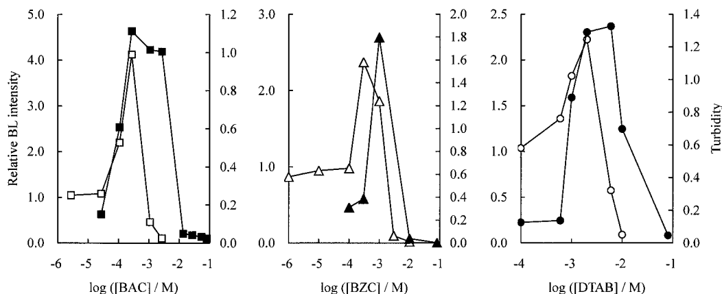
Fig. 5 Effect of cationic surfactant concentration on relative BL intensity (open) and turbidity (filled). Both PC and Chol concentrations are 1.25 \times 10^{-3} M.
