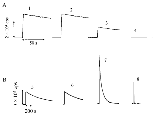
Fig. 2 Typical BL response curves in the presence of BAC (A) and of both BAC and VET 100 (B). In A, BAC concentrations are 0 (curve 1), 2.7 \times 10^{-6} (2), 2.7 \times 10^{-5} (3), and 2.7 \times 10^{-4} M (4). In B, BAC are 0 (curve 5), 2.7 \times 10^{-6} (6), 2.7 \times 10^{-4} (7), and 2.7 \times 10^{-3} M (8), all containing VET 100 at 1.25 \times 10^{-3} M PC and 1.25 \times 10^{-3} M Chol.
