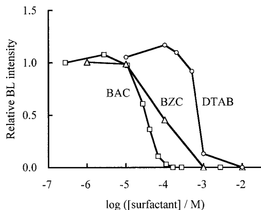
Fig. 3 Effect of cationic surfactant concentration on relative BL intensity.
