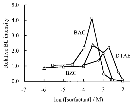
Fig. 4 Effect of cationic surfactant concentration on relative BL intensity in the presence of VET 100 . Both PC and Chol concentrations are 1.25 \times 10^{-3} M.
