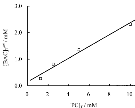
Fig. 6 Relationship between PC and saturating BAC concentrations.
