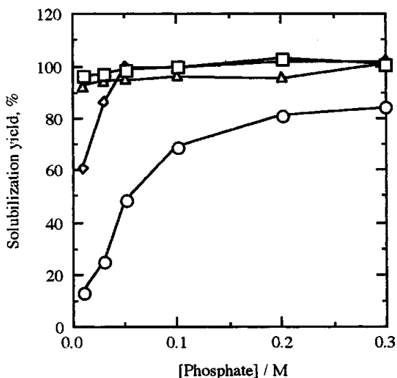
Fig. 4 Effect of the phosphate concentration on the solubilization of the microsomal electron-transfer proteins. (□), cytochrome b 5 ; (○), cytochrome P450; (◇), NADH-cytochrome b 5 reductase; (△), NADPH-cytochrome P450 reductase. The experiment was carried out at a protein concentration of 3.5 mg/ml and at 1.5%(w/v) OTG with 1 mM EDTA and 20%(v/v) glycerol.
