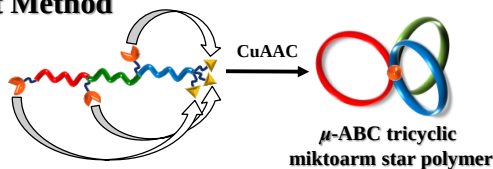
Scheme 1. (a) Previous and (b) present synthetic approaches for \mu -ABC tricyclic miktoarm star polymers.
