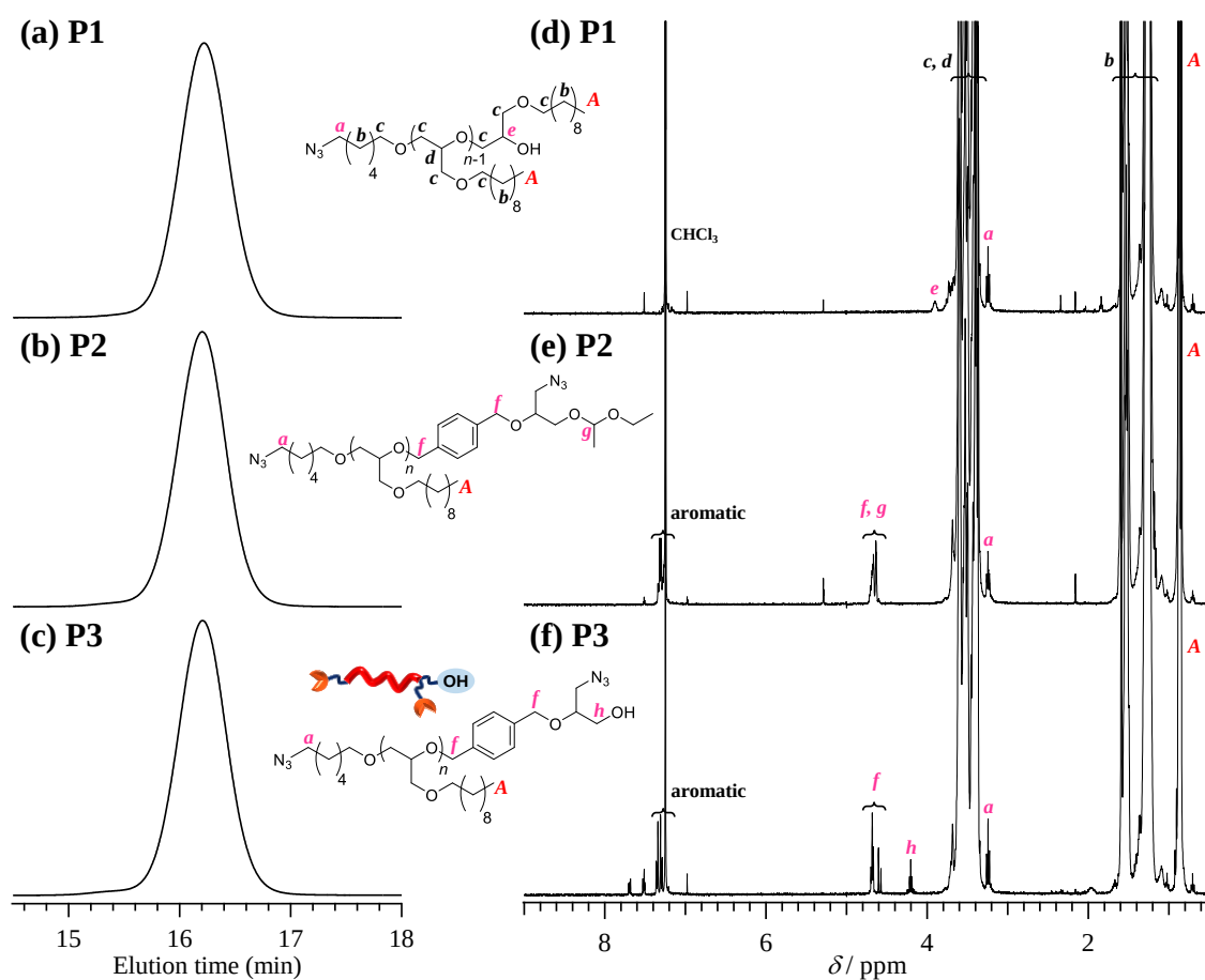
Figure 1. (a–c) Size exclusion chromatography (SEC) traces of P1 , P2 , and P3 . (d–f) ^1\text{H} NMR spectra of P1 , P2 , and P3 in \text{CDCl}_3 (400 MHz).
