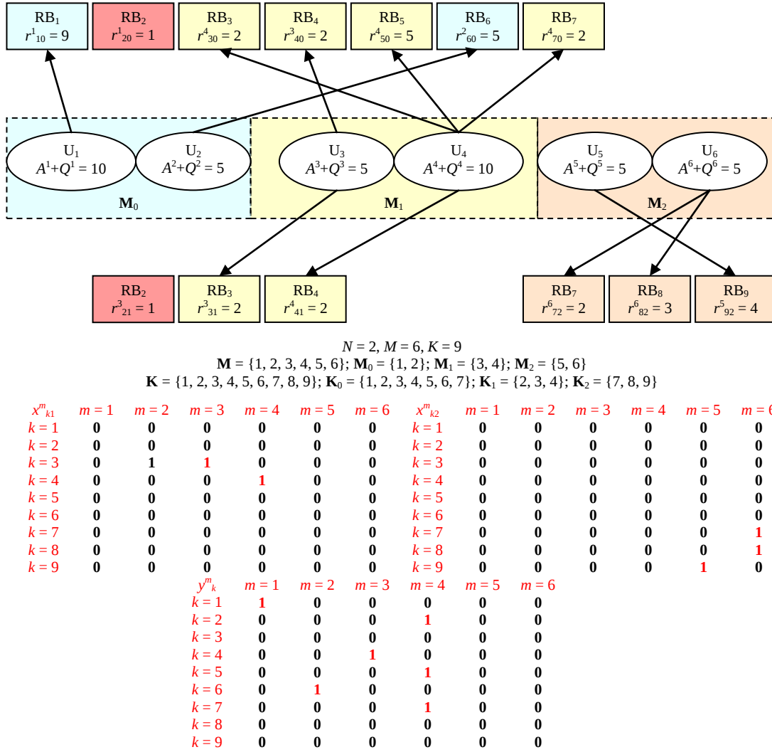
Figure 4. Result of RB allocation in the network with 2 pNBs and 6 users.
