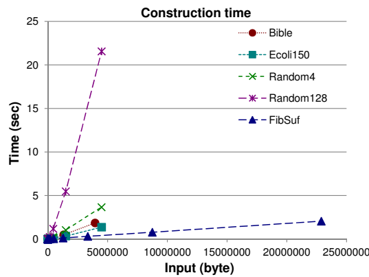
Figure 16: Exp 4. Computation time of Construct with increasing size of a data set.
