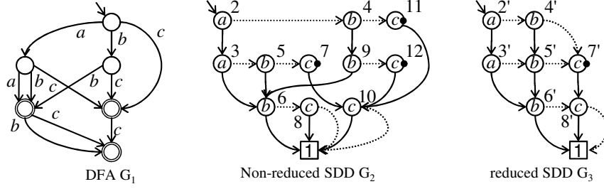
Figure 4: A minimal acyclic DFA G_1 (left), a non-reduced sequence BDD G_2 (middle), and a reduced sequence BDD G_3 (right) on \Sigma_1 = \{a, b, c\} for the same finite language L_1 in Example 1. The numbers at each node indicate vertex id. The 0-terminal \mathbf{0} is omitted, and all edges incoming to \mathbf{0} are indicated by a small black dot.
