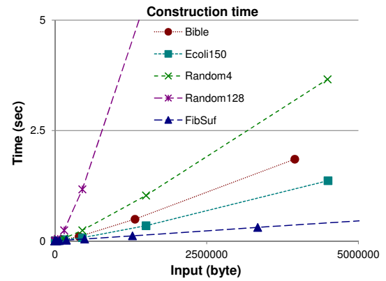
Figure 17: Exp 4. Computation time of Construct with increasing size of a data set (enlarged view).
