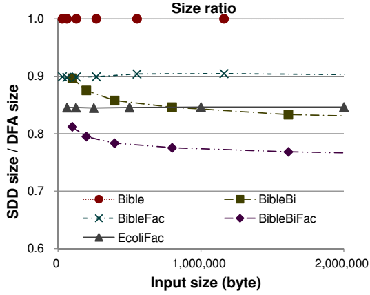
Figure 12: Exp 1. Ratio between the sizes of minimum sequence BDDs and ADFAs.
