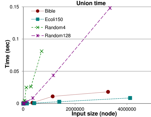
Figure 15: Exp 3. Computation time of Meld_{\cup} with increasing sum of input sequence BDD sizes.
