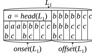
Figure 3: The binary decomposition of a finite language L_1 = \{aab, aac, aa, abb, abc, ab, acc, ac, bbb, bbc, bb, bcc, bc, cc, c\} in Example 1.
