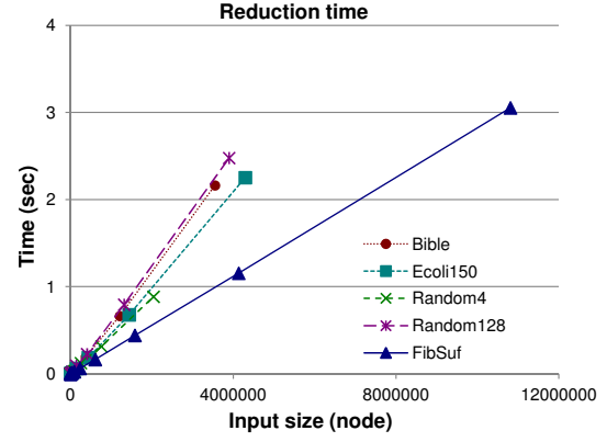
Figure 13: Exp 2. Computation time of Reduce with increasing sequence BDD size.
