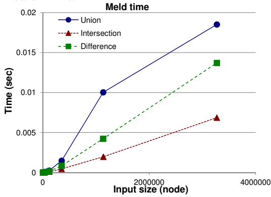
Figure 14: Exp 3. Computation time of Meld_{\diamond} for \diamond \in \{\cup, \cap, \setminus\} with increasing sum of input sequence BDD sizes.
