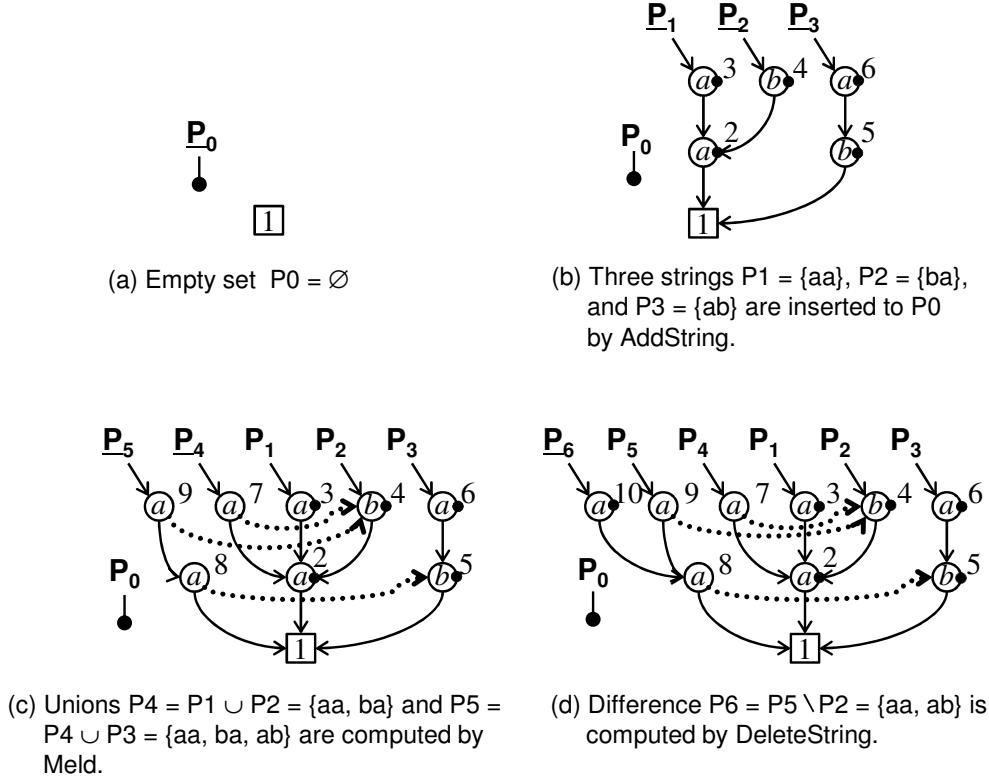
Figure 10: An execution example of \text{AddString} , \text{DeleteString} , and \text{Meld}_\cup in a shared sequence BDD environment \mathcal{E} , where the computation proceeds in write-only manner. In the figure, each circle stands for a vertex, and an associated symbol and a number indicate its vertex label and vertex id, respectively. The terminal 1 is indicated by a square with 1, and 0 is omitted. A small black dot indicates a pointer to 0 .
