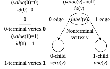
Figure 2: The 0-terminal, 1-terminal and nonterminal vertices.
