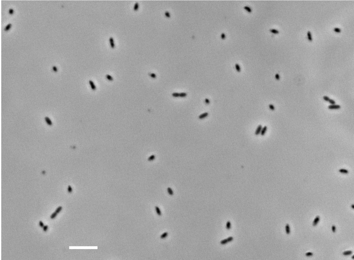
Fig S1. Fig. 1 Phase-contrast micrograph of strain Ok2G T . Bar, 5 \mu m.
