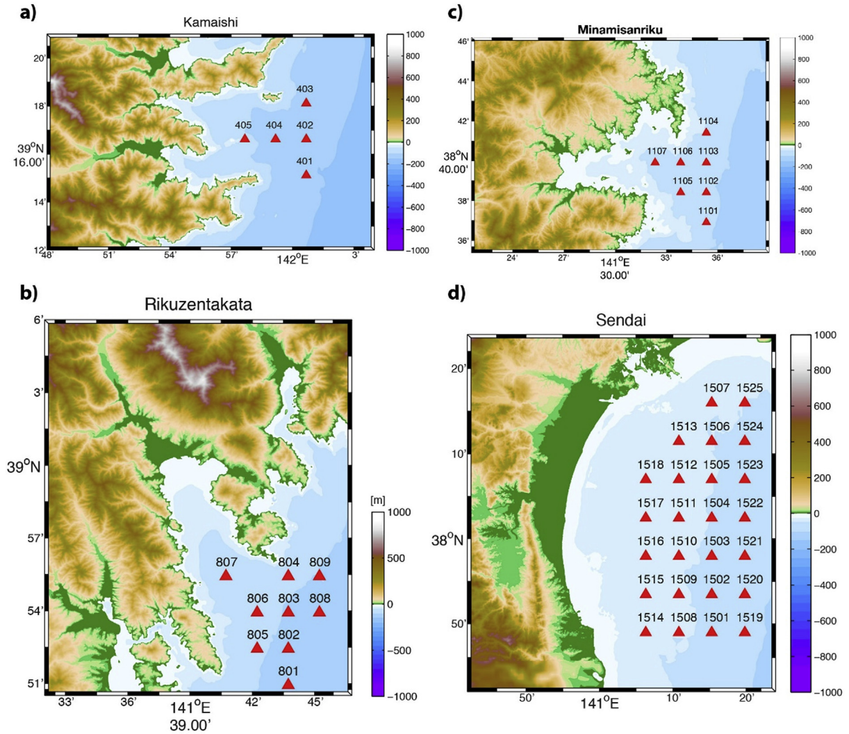
Fig. 4. Virtual observation points (red triangles) at four sites, (a) Kamaishi, (b) Rikuzentakata, (c) Minamisanriku, and (d) the Sendai Plain. Precomputed tsunami waveforms at those virtual observation points are stored in the database. (For interpretation of the references to color in this figure legend, the reader is referred to the web version of this article.)
