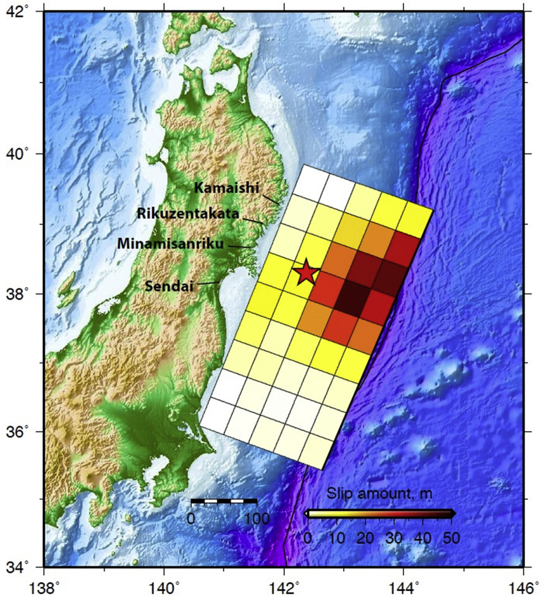
Fig. 1. The slip distribution of the 2011 Tohoku-oki earthquake (Gusman et al., 2012) was used as an original source model in this study. The four test sites: Kamaishi, Rikuzentakata, Minamisanriku, and the Sendai Plain used, for a synthetic tsunami inundation forecast for the 2011 Tohoku-oki tsunami.
