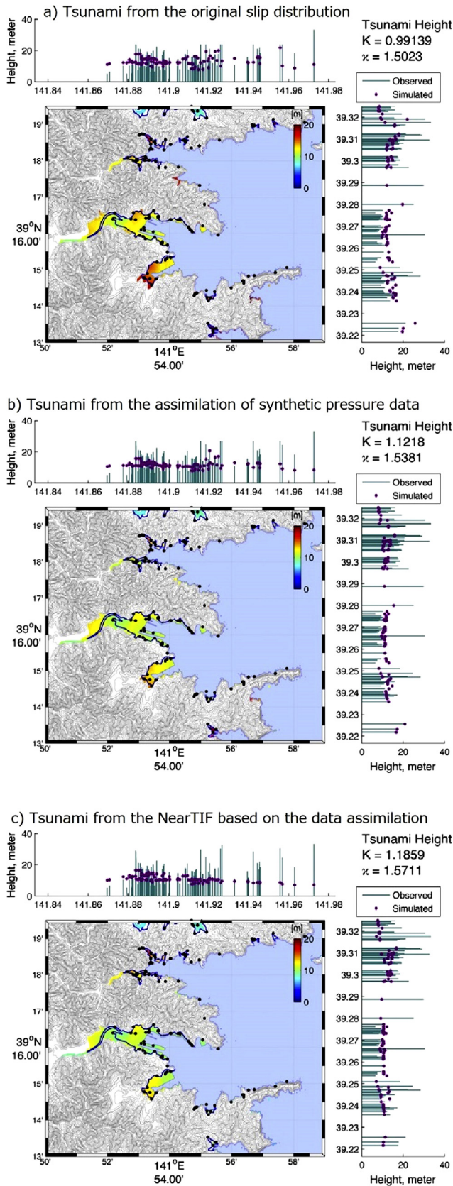
Fig. 7. For Kamaishi, (a) the tsunami inundation computed from the original slip distribution, (b) from the assimilation of synthetic pressure data, and (c) from the NearTIF based on the data assimilation. Bars are observed tsunami heights. Purple dots are the computed maximum tsunami heights. The geometric mean ratio of Aida (1978) number K , and its corresponding standard deviation, \kappa , are also shown.
