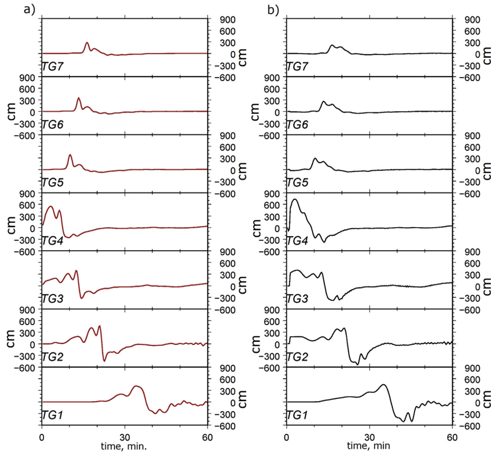
Fig. 6. Comparison of tsunami waveforms at seven locations, the open circles in Fig. 5. (a) Tsunami simulation from the original slip distribution, (b) that from the assimilation of synthetic pressure data.
