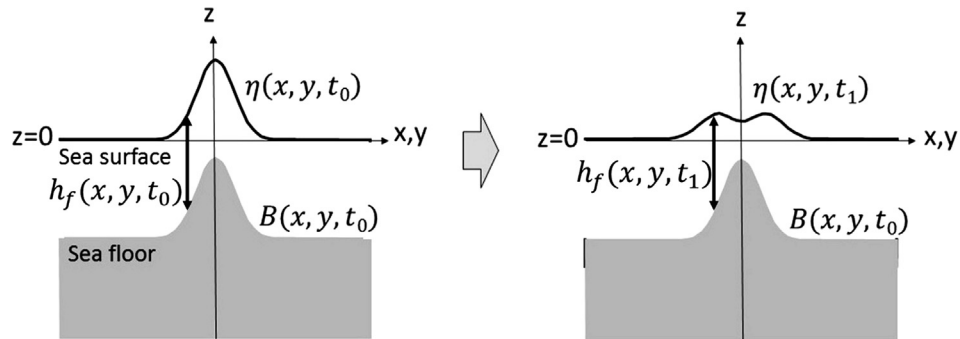
Fig. 2. Schematic illustrations of the ocean surface displacement or tsunami height, \eta(x, y, t) , permanent sea floor deformation caused by the earthquake, B(x, y, t) , and the water-depth fluctuation, h_f(x, y, t) . The earthquake or tsunami generation is completed at a time of t_0 .
