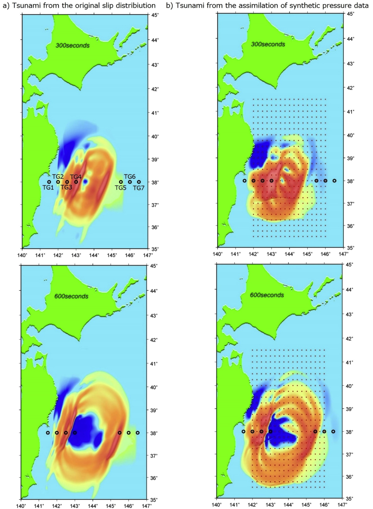
Fig. 5. Tsunami height distribution at 300 s, and 600 s after the origin time. (a) Tsunami numerical simulation from the original slip distribution, and (b) tsunami simulation from the assimilation of synthetic pressure data at sensors shown in Fig. 3.
