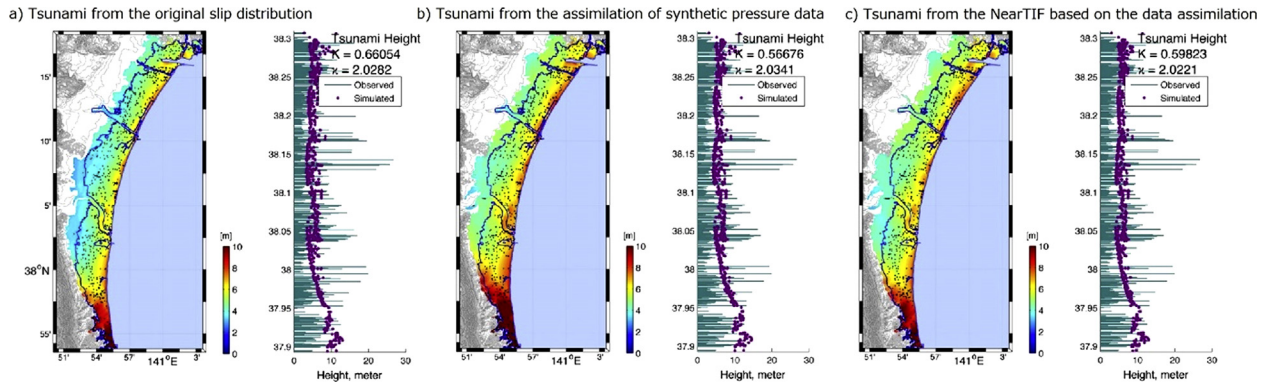
Fig. 10. For Sendai Plain, (a) the tsunami inundation computed from the original slip distribution, (b) from the assimilation of synthetic pressure data, and (c) from the NearTIF based on the data assimilation. Bars are observed tsunami heights. Purple dots are the computed maximum tsunami heights. The geometric mean ratio of Aida (1978) number K , and its corresponding standard deviation, \kappa , are also shown.
