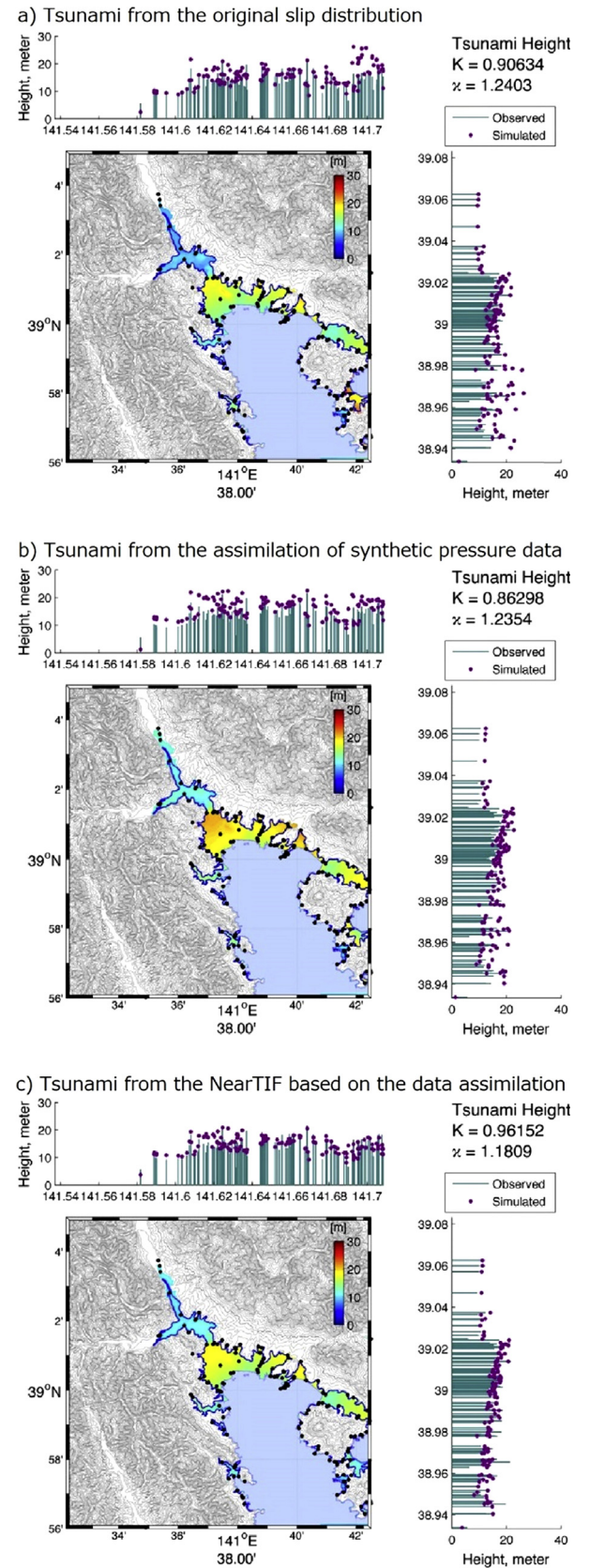
Fig. 8. For Rikuzentakata, (a) the tsunami inundation computed from the original slip distribution, (b) from the assimilation of synthetic pressure data, and (c) from the NearTIF based on the data assimilation. Bars are observed tsunami heights. Purple dots are the computed maximum tsunami heights. The geometric mean ratio of Aida (1978) number K , and its corresponding standard deviation, \kappa , are also shown.
