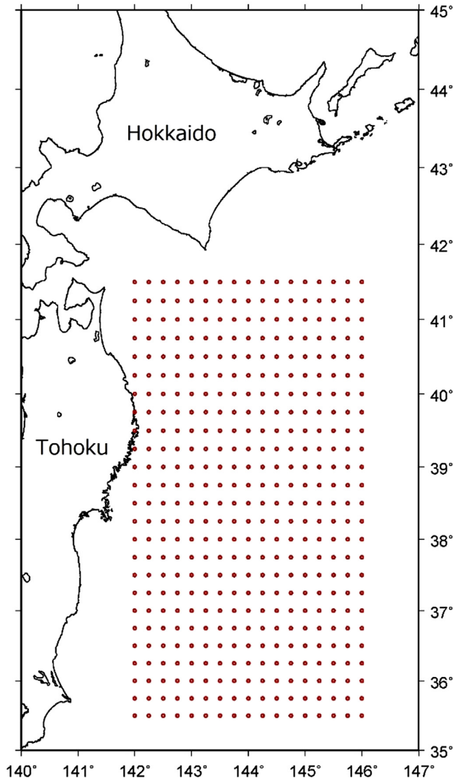
Fig. 3. Ocean bottom pressure sensor distribution for the synthetic test. Sensors (red circles), are located with 15 arc-min intervals.
