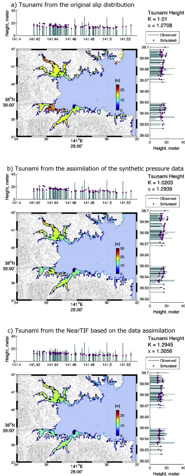
Fig. 9. For Minamisanriku, (a) the tsunami inundation computed from the original slip distribution, (b) from the assimilation of synthetic pressure data, and (c) from the NearTIF based on the data assimilation. Bars are observed tsunami heights. Purple dots are the computed maximum tsunami heights. The geometric mean ratio of Aida (1978) number K , and its corresponding standard deviation, \kappa , are also shown.
