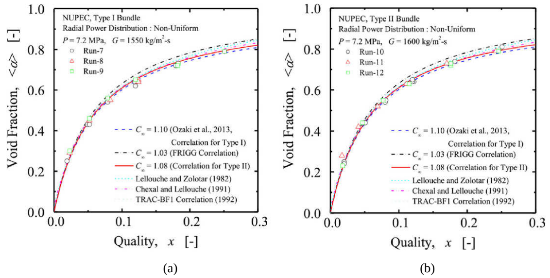
Figure 2-3 Comparison of Ozaki and Hibiki's correlation with void fraction measured in vertical 8×8 rod bundle [2-16].
