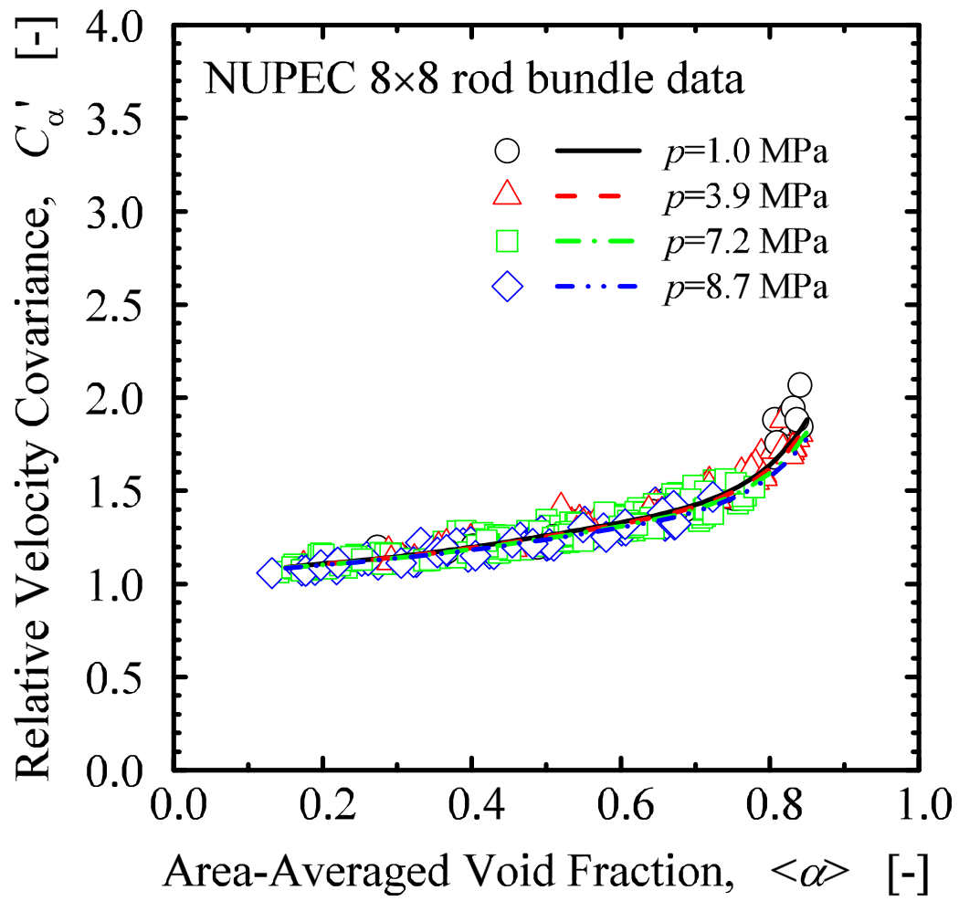
Figure 2-6 Comparison of Ozaki and Hibiki's correlation with relative velocity covariance measured in vertical 8x8 rod bundle [2-44].
