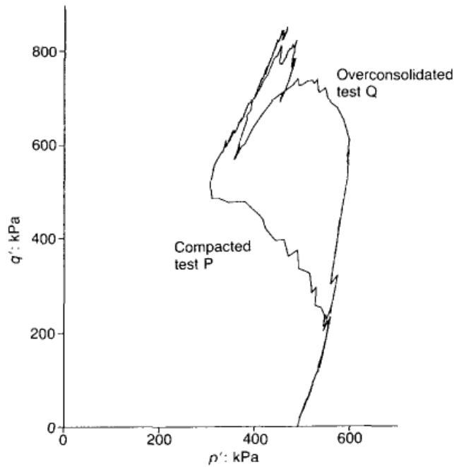
Figure 3.2. Comparison of strength behavior between compacted and overconsolidated samples of carbonate sand (Coop, 1990)
