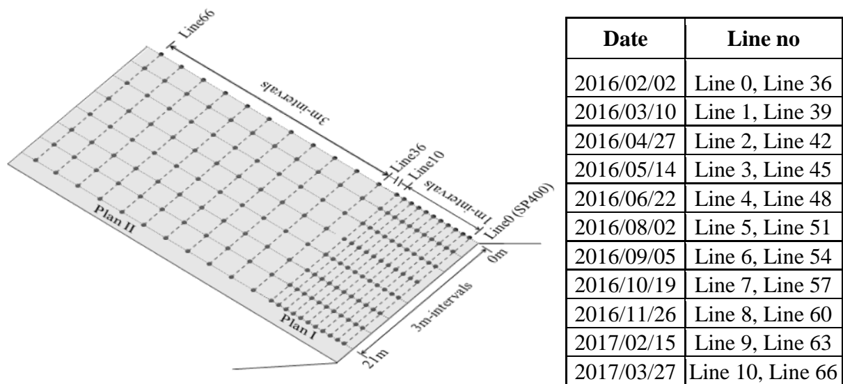
Figure 5.13. Plans and dates of cone penetrometer testing in Maizuru river dyke slope
