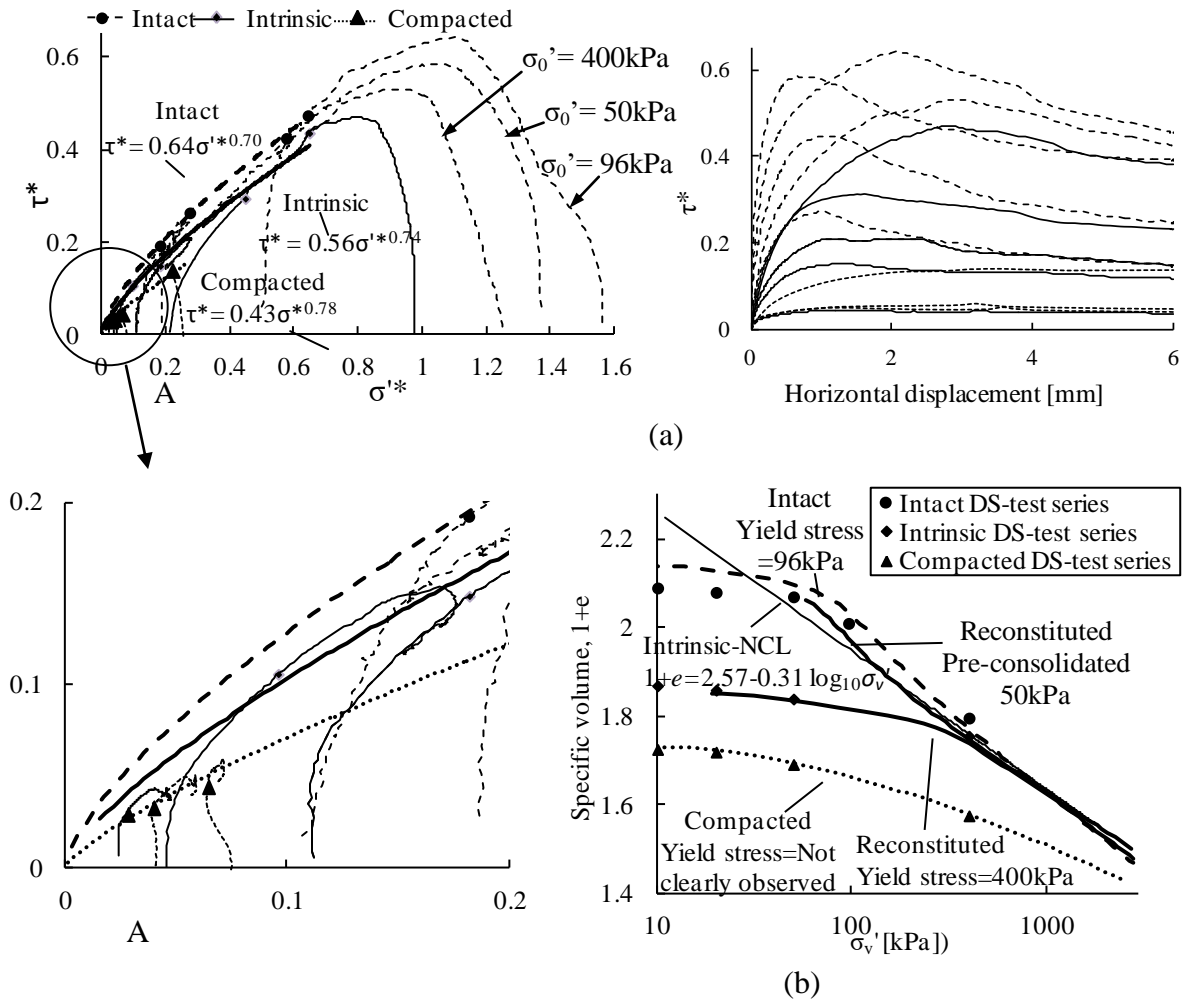
Figure 6.5. (a) Normalized stress paths and state bounding surfaces (b) Compression curves and volume-effective stress states before undrained shearing
