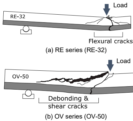
Fig. 3. Typical crack patterns observed from the tests.
