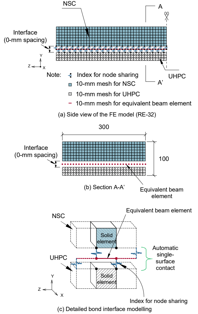
Fig. 4. Details of FE modelling.
