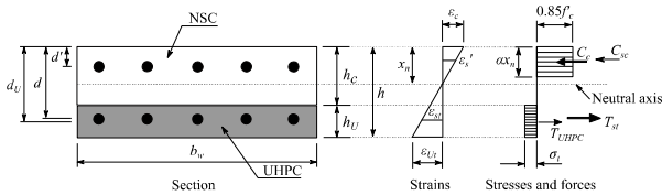
Fig. 12. Calculation assumptions for flexural strength of composite UHPC-concrete members.
