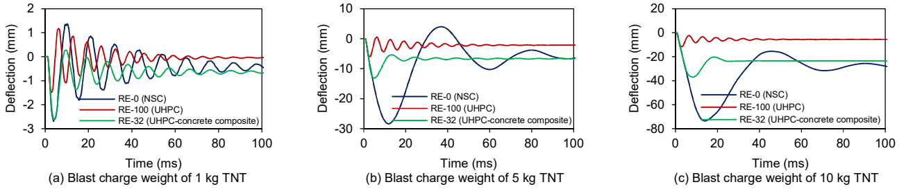
Fig. 8. Comparisons of simulated deflection-time histories for UHPHC-concrete composite specimen RE-32, and non-composite specimens RE-0 (NSC) and RE-100 (UHPHC).
