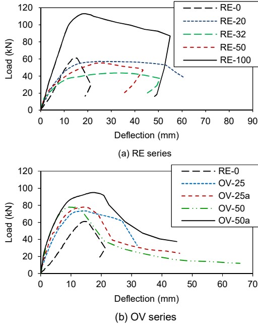
Fig. 2. Load-midspan deflection curves of the test specimens.
