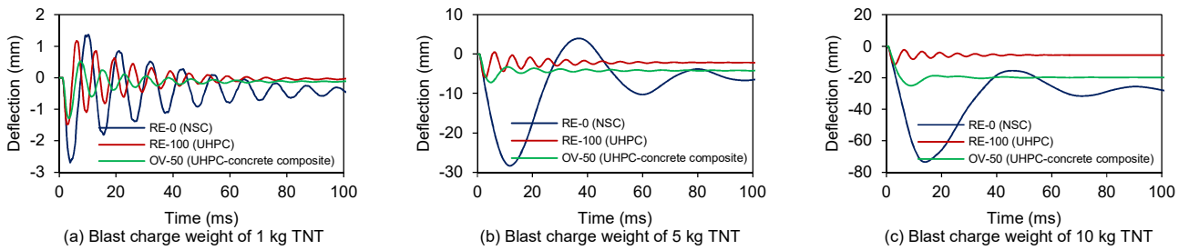
Fig. 9. Comparisons of simulated deflection-time histories for UHPHC-concrete composite specimen OV-50, and non-composite specimens RE-0 (NSC) and RE-100 (UHPHC).
