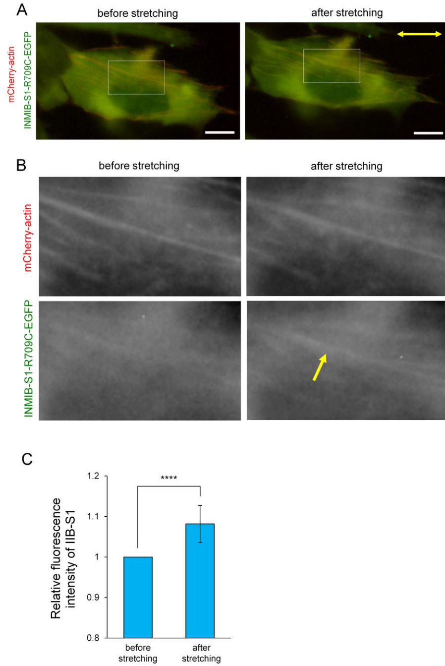
Figure 12. NMIIB-S1-R709C-EGFP can be used as a probe for stretched actin filaments.
