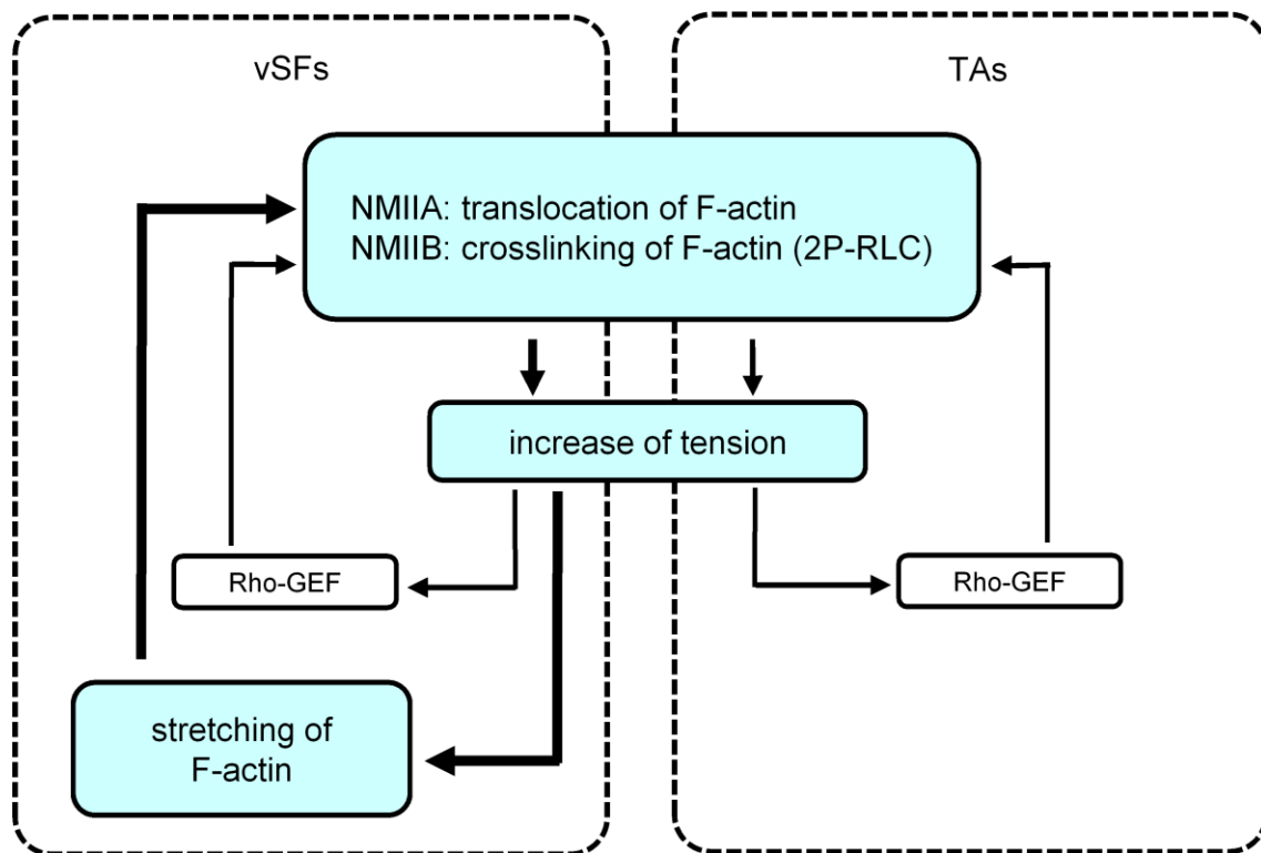
Figure 35. Proposed schematic model of the positive feedback loops of tension generated by the SF subtypes. In addition to the positive feedback loop regulated by Rho-GEF activation, there is another feedback loop that involves stretch-induced conformational changes of actin filaments in vSFs in cell bodies.
