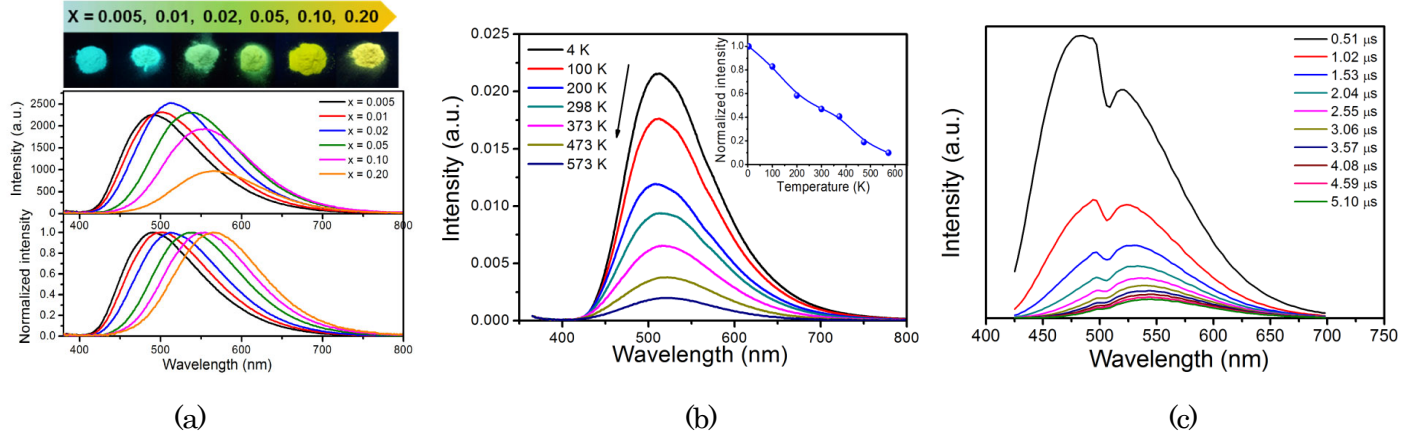
Figure 4 (a) Emission spectra of JEM:Eu phosphors with different Eu concentrations, thermal quenching behavior (b) and time resolved emission spectra (c) of JEM:0.02Eu phosphor.
