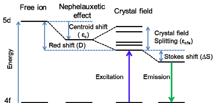
Figure 2 A diagram of the effects of centroid shift, crystal field splitting and Stokes shift on lowering of the energy of the 5d levels for \text{Eu}^{2+} or \text{Ce}^{3+} ion in a compound.
