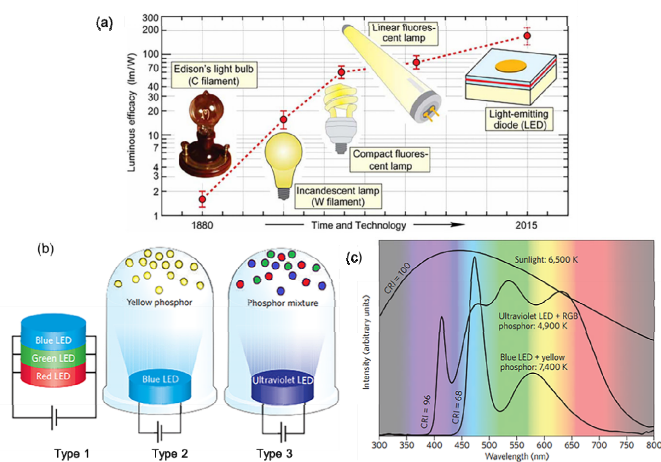
Figure 1 (a) Comparison of the luminous efficacy of several lighting technologies; (b) three dominant ways to produce white LEDs; (c) comparison of the spectrum of ideal sunlight with two LED-based white-light sources.
