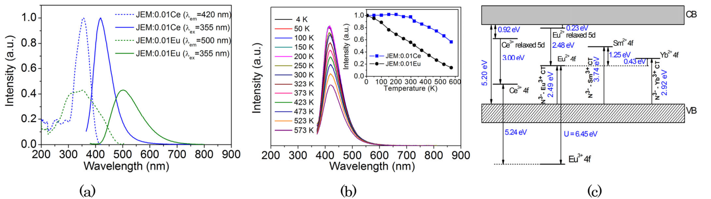
Figure 5 (a) Photoluminescence spectra of JEM:0.01Eu and JEM:0.01Ce phosphors; (b) thermal quenching behavior of JEM:0.01Ce phosphor and (c) an energy level scheme of JEM:Ln phosphors (Ln = Ce, Eu, Sm, Yb).
