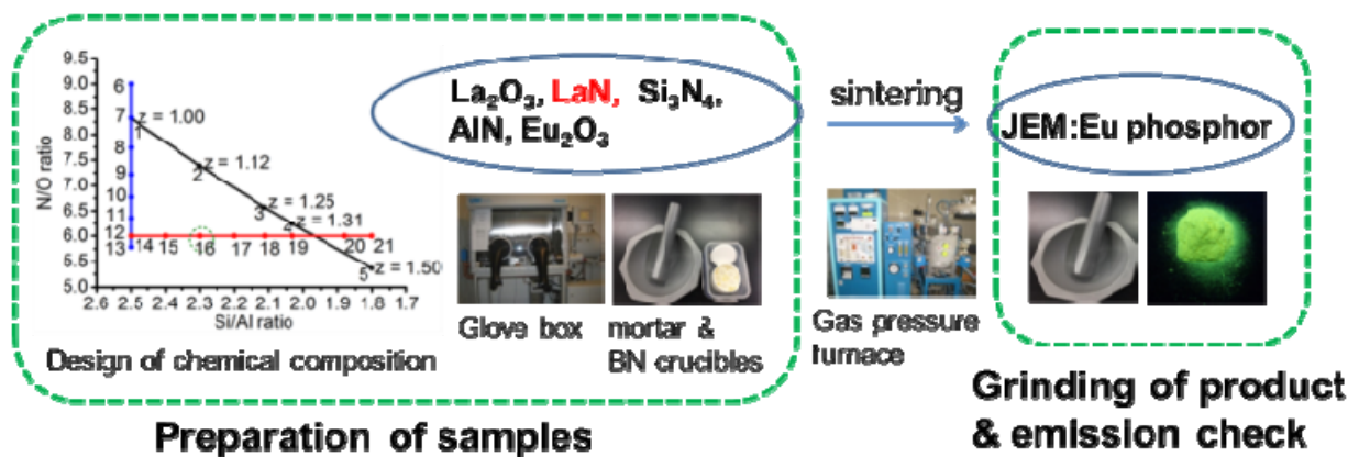
Figure 3 A schematic diagram of process to synthesize JEM:Eu phosphor.
