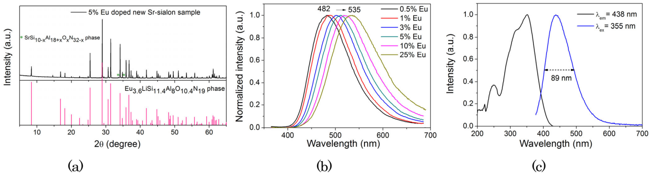
Figure 7 (a) XRD pattern of 5% Eu doped new Sr-sialon phase sample; (b) Eu concentration dependent emission spectra and (c) photoluminescence spectra of 5% Ce,Li doped new Sr-sialon phase.
