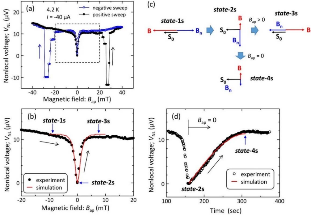
Fig. 4.9: (a) Experimental results of the nonlocal spin-valve signal measured at 4.2 K for a fixed bias current I_{bias} = -40 \mu A , (b) (closed circles) spin-valve signal for positive sweep only along with (red curve) fit with simulation result for parallel configuration, (c) schematic vector diagrams showing relative orientations of S_0 , B , and B_n in the spin-valve measurement, and (d) V_{NL} as a function of time ( t ). Open circles show the experimental result and the red curve indicates the simulation after B_{ap} was switched off at t = 160 s.
