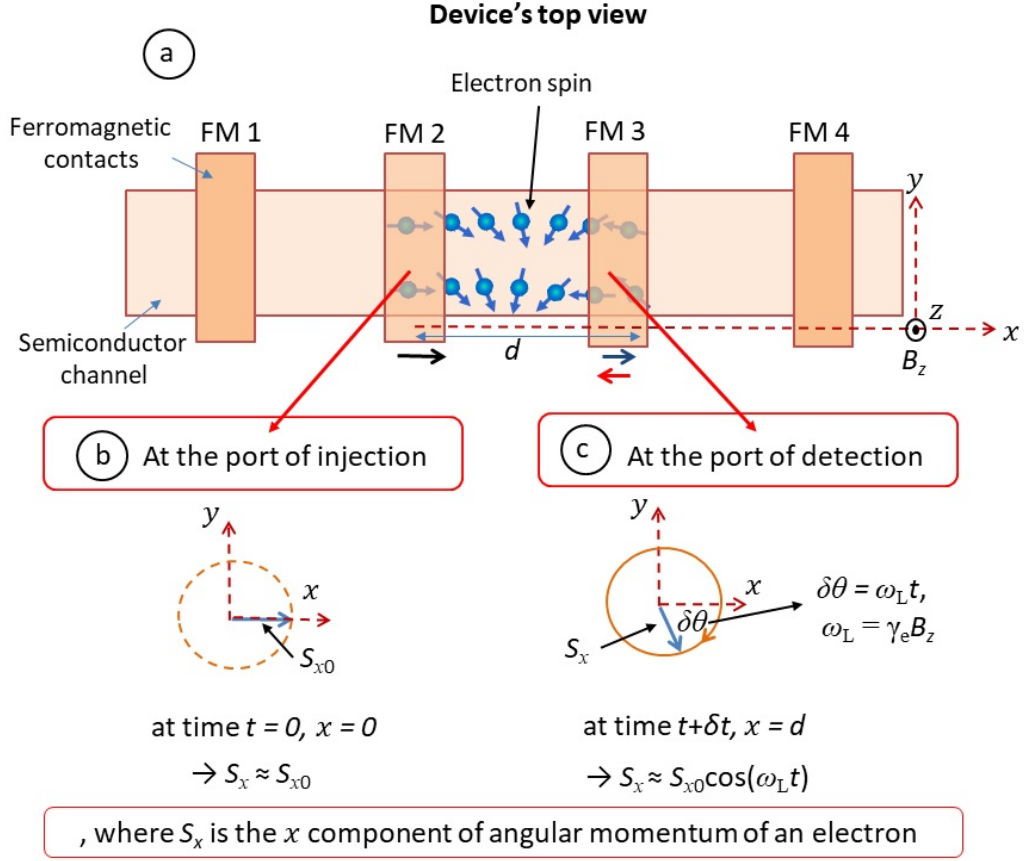
Fig. 2.5: A schematic description for the behavior of an electron spin under a magnetic field B_z perpendicular to the direction of spin polarization (Hanle effect), where x axis is considered the direction of spin polarization, see text.
