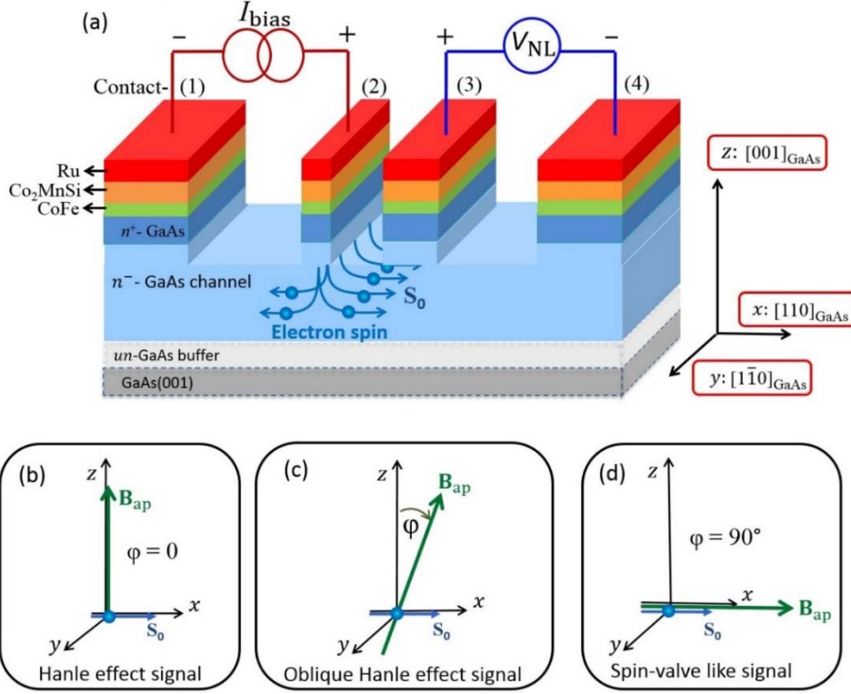
Fig. 3.6: (a) A schematic description of the electrical spin injection along with the nonlocal voltage detection geometry, (b), (c) and (d) the direction of the applied magnetic field \mathbf{B}_{ap} during measurement of the typical Hanle signal, oblique Hanle signal (without and with irradiation by rf-magnetic field), and spin-valve like signal, respectively, with respect to the direction of electron spin polarization \mathbf{S}_0 .
