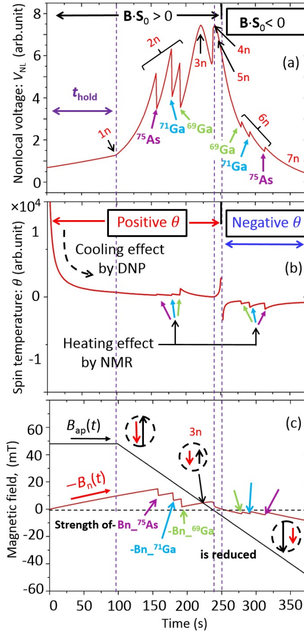
Fig. 5.3: Simulation results of the change in (a) a nonlocal voltage V_{NL} , (b) a spin temperature \theta and (c) a transient nuclear field B_n along with a magnetic field B_{\text{ap}} of an oblique Hanle signal with irradiation by rf magnetic field.
