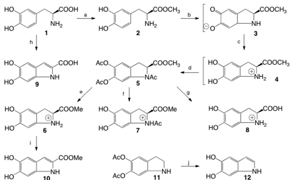
Figure 1. Synthetic scheme for the preparation of cycloDOPA derivatives. (a) SOCl_2 , MeOH, reflux, 1 h, quant; (b) K_3[Fe(CN)_6] , sodium phosphate (pH = 8), 0 °C, 75 s; (c) Na_2S_2O_4 , sodium phosphate (pH 8), 0 °C, 30 s; (d) Ac_2O , pyridine, rt, 4 h, 60% (3 steps); (e) AcCl , MeOH, 60 °C, 16 h, 97%; (f) 1 M HCl, MeOH, rt, 3 days, 59%; (g) 6 M HCl, 80 °C, 5 h, 94%; (h) (1) K_3[Fe(CN)_6] , NaHCO_3 , rt, 5 min, (2) 1M NaOH, rt, 15 min, 71%; (i) NaOH (pH = 10), rt, o/n, 48%; (j) K_2CO_3 , MeOH, 0 °C, 50 min, 51%.
