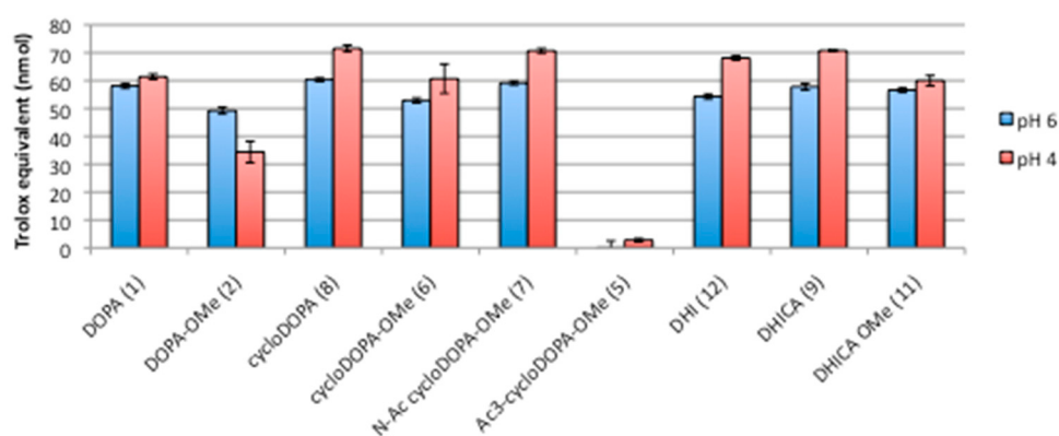
Figure 5. DPPH radical scavenging activity of cycloDOPA and its derivatives. Samples (20 \mu M) were subjected to the scavenging assay after an incubation time of 20 min. Activities were expressed by Trolox equivalent values. The DPPH assay was performed in triplicate for each sample.
