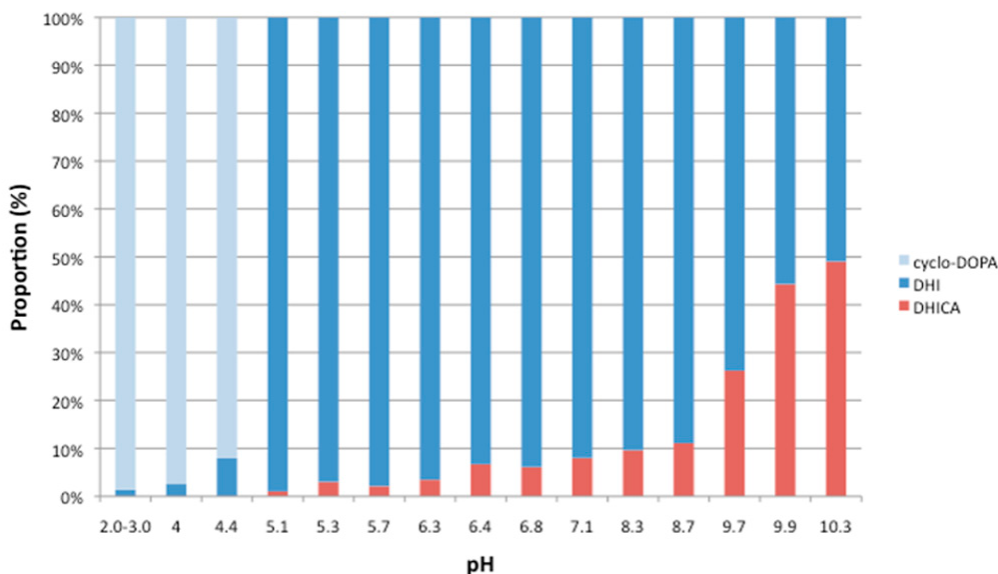
Figure 3. The products distributions of the decomposition of cycloDOPA ( 8 ) at different pH levels. CycloDOPA ( 8 , 35 mg) was dissolved in D 2 O (0.5 mL) and CH 3 CN (1 \mu L), and the solution was adjusted to the indicated pH with a NaOD solution. The incubation time refers to the time required for cycloDOPA to be consumed completely, expected pH = 3.6 and pH = 4.4.
