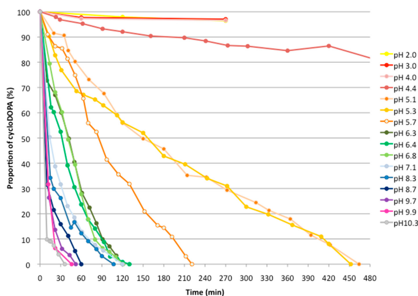
Figure 2. pH stability of cycloDOPA (8) in D 2 O solution. Solutions of CycloDOPA (4 mg) in D 2 O (0.5 mL, 34 mM, pH < 2) were adjusted to pH levels ranging from 2 to 10 using 1 M NaOD/D 2 O. The resulting samples were analyzed, and the decreases in the α- and β- protons of cycloDOPA were calculated.
