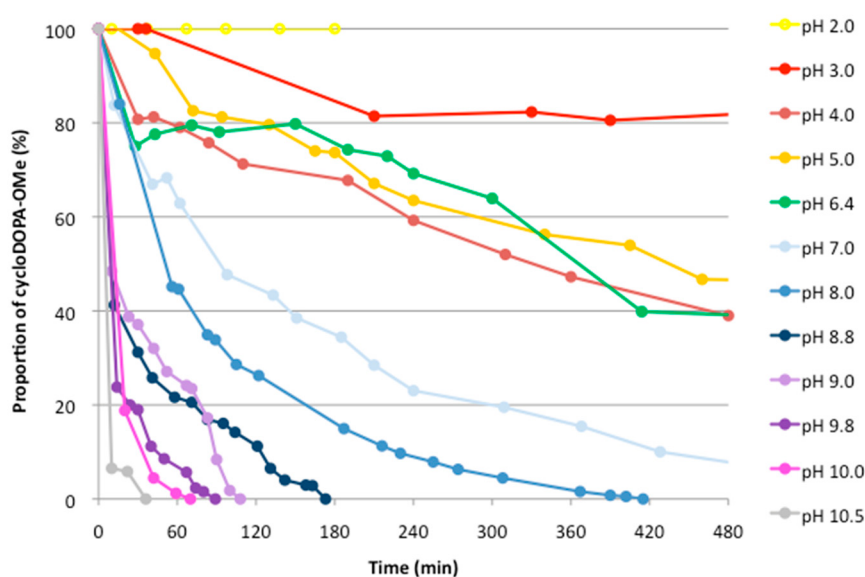
Figure 4. pH stability of cycloDOPA-OMe (6) in a D 2 O solution. Solutions of cycloDOPA methyl ester (4 mg) in D 2 O (0.5 mL, 34 mM, pH < 2) were adjusted to each of the listed pH values using 1 M NaOD/D 2 O. These samples were measured after certain time intervals, and the decrease in the \alpha - and \beta -protons of the cycloDOPA-OMe was calculated.
