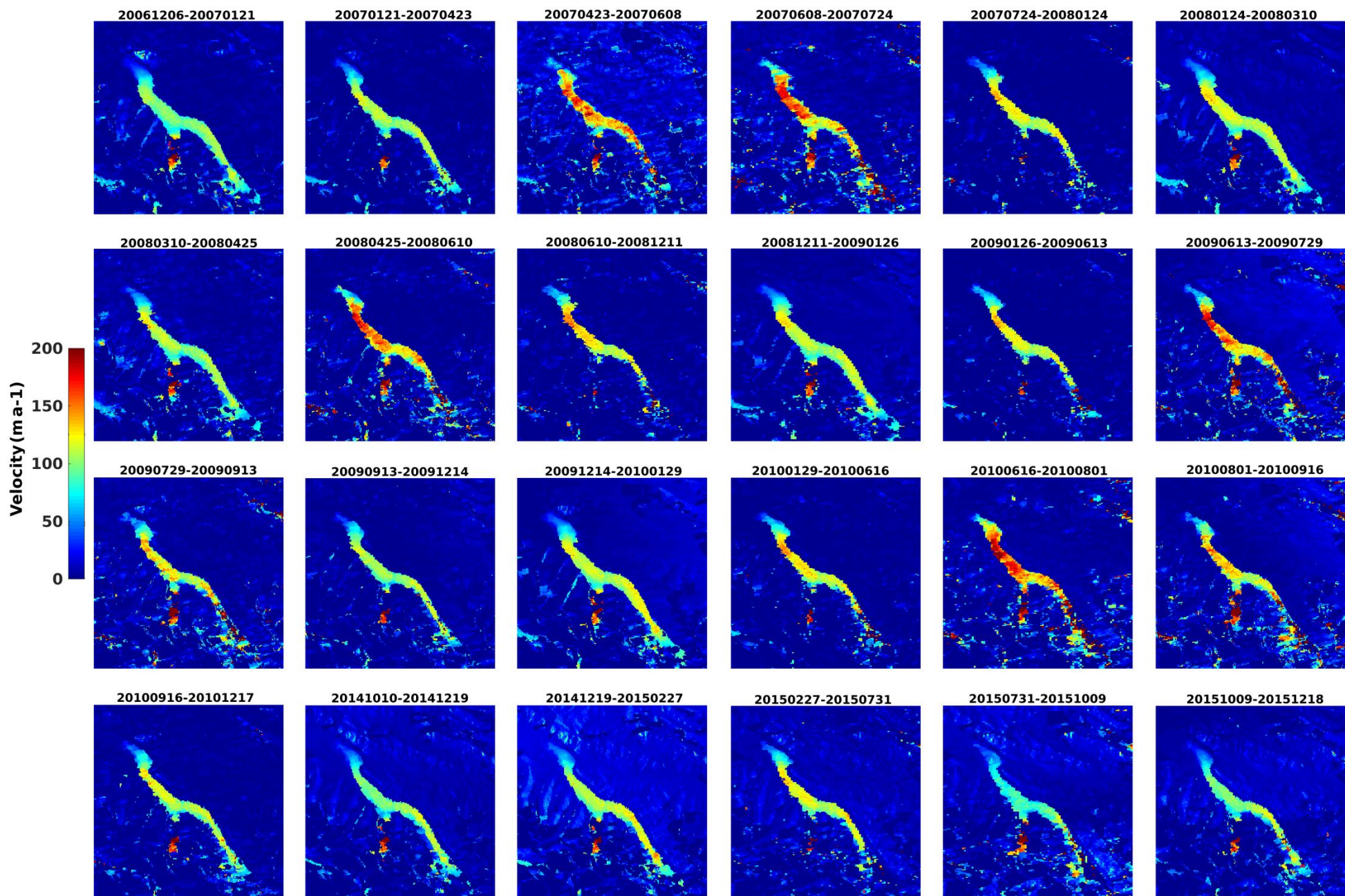
Figure S5. Surface velocity field of Singkhu Glacier from 2007 to 2015
