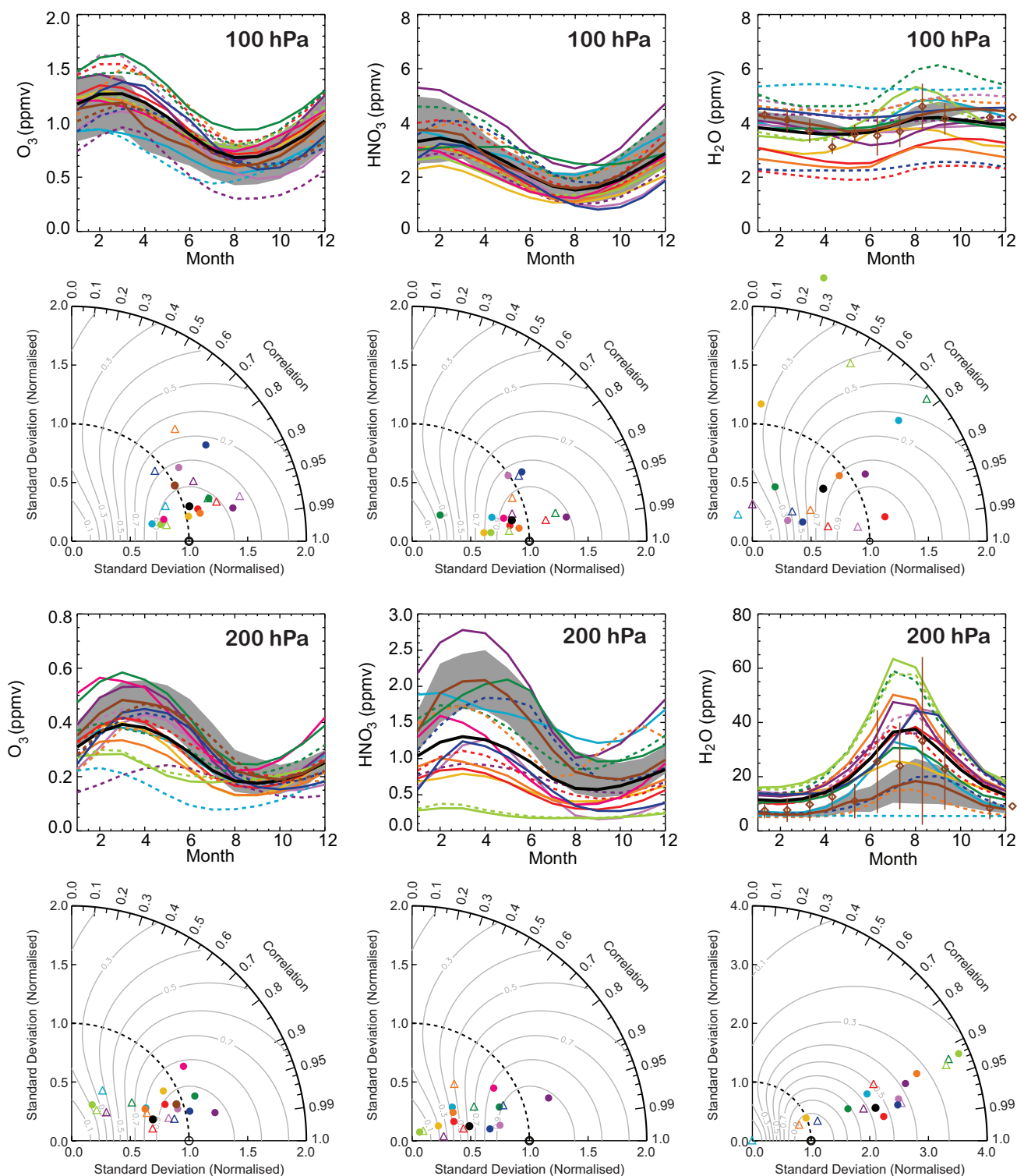
Figure 7.22: Seasonal cycles in monthly mean O_3 , HNO_3 , and H_2O between 40^\circ N and 60^\circ N and corresponding Taylor diagrams at 100 hPa (upper two rows) and 200 hPa (lower two rows) for different models (colour-coded) compared to MIPAS satellite data and their 1\sigma uncertainty (brown solid lines and gray shading) over the years 2004-2008. For O_3 , MLS data over the years 2004-2008 (brown dashed lines and dots), and for H_2O , ACE-FTS data (brown diamonds) are shown in addition to the MIPAS data. Black lines and dots indicate the multi-model mean.
