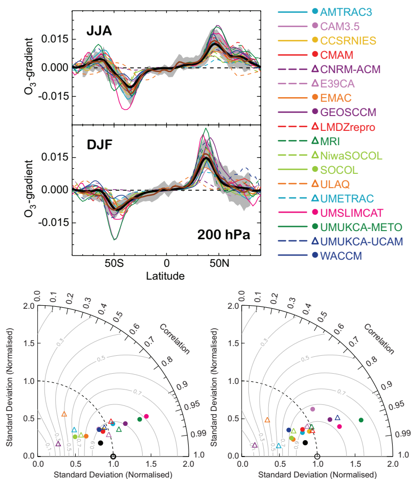
Figure 7.24: Meridional gradient in \text{O}_3 (ppmv/deg) at 200 hPa and corresponding Taylor diagrams for JJA (left panel) and DJF (right panel). Brown lines indicate MLS data averaged over the years 2004-2008, black thick lines and dots the multi-model mean. The gray region in the top panel indicates 1\sigma from the observations.
