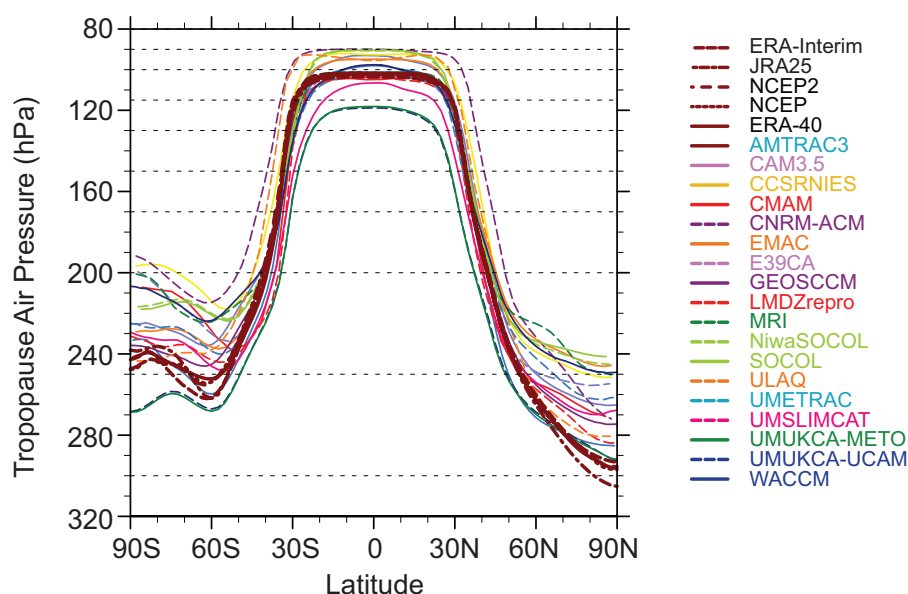
Figure 7.5: REF-B1 lapse rate tropopause pressure (PTP) annual zonal mean for 1980-1999 from models and analysis systems. Dotted lines represent CCMVal-2 vertical level structure in the UTLS, with levels at 400, 300, 250, 200, 170, 150, 130, 115, 100, 90, 80, 70, 50 hPa.
