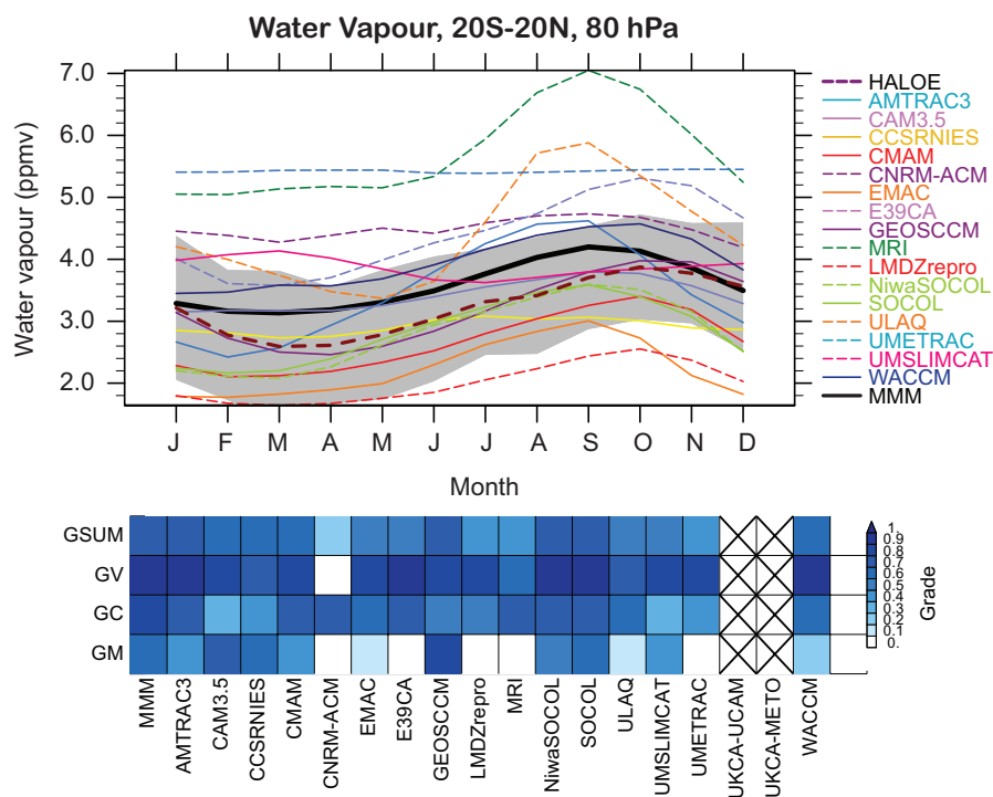
Figure 7.10: (Above): Annual cycle of tropical (20°S-20°N) water vapour at 80 hPa from models and observations. Output from the period 1992-2004. Gray shaded region is 3σ variability from HALOE observations over 1992-2004 (brown dashed line). (Below): Quantitative metrics summary of 80hPa H 2 O for mean (GM), correlation (GC), variance (GV) and the average of all three grades (GSUM).
