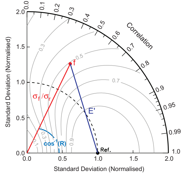
Figure 7.2: A sample Taylor diagram. f indicates the test or model field, and Ref. (or r ) a reference field. The inverse cosine of the correlation R between the test and reference field (indicated in light blue) determines the location on the azimuthal axis. The radial distance of f from the origin corresponds to the standard deviation of the test field normalised by the standard deviation of the reference field ( \sigma_f / \sigma_r , red line). The RMS difference ( E' , dark blue line) between test and reference field is proportional to the distance between the two fields on the diagram. Grey thin lines indicate the skill score ( S ) of the test field, which obtains in this example a value of 0.51.
