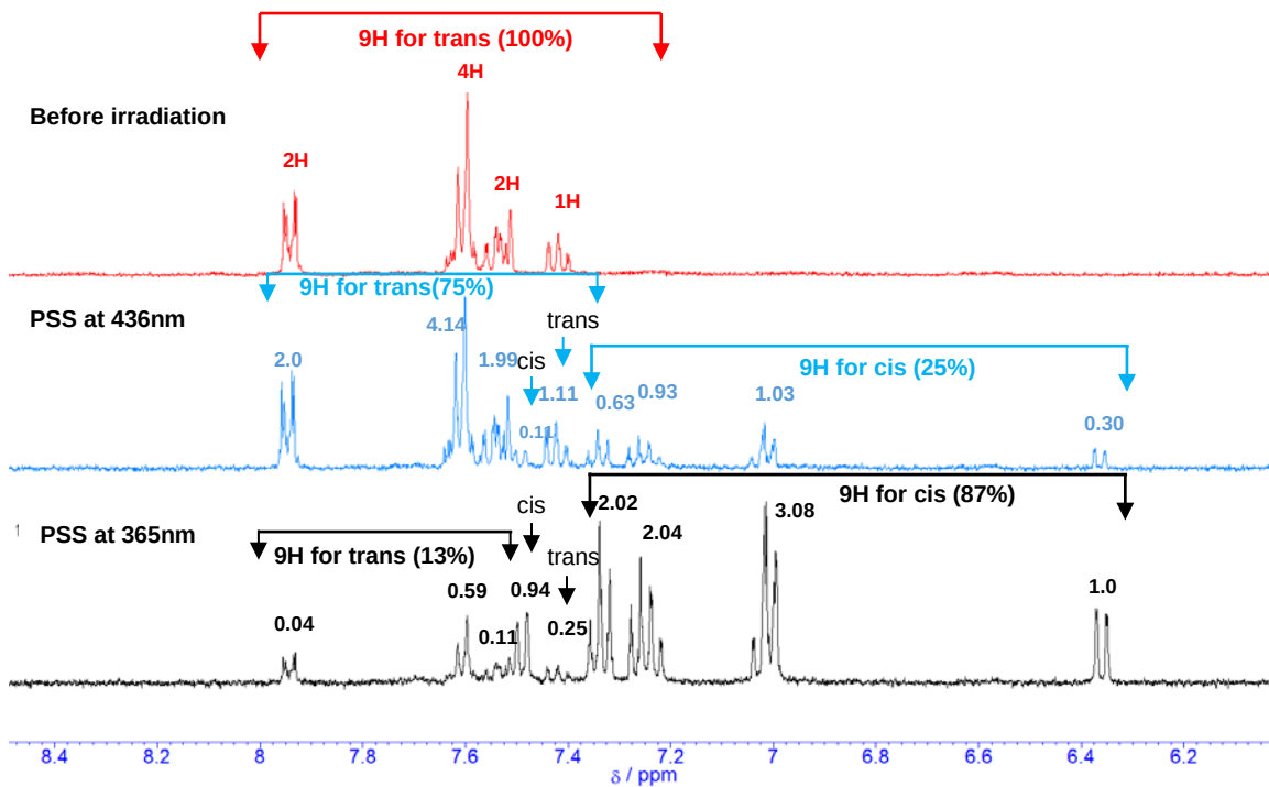
Fig. S2. ^1\text{H} NMR spectra (400 MHz, \text{D}_2\text{O} ) showing the trans and cis isomer ratios of a ) AzoethoxyTP ( 4b ), b ) DimethylAzoTP ( 4c ) and c ) AzoethylTP ( 4d ) before irradiation, at UV PSS and Visible PSS.
