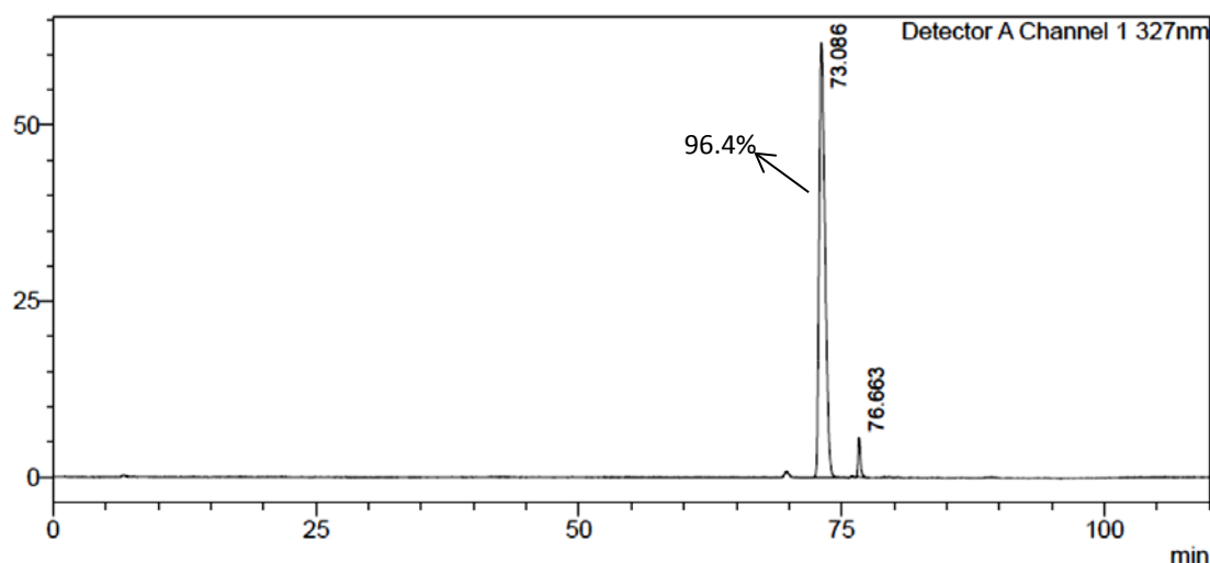
Fig. S4. Reverse phase HPLC chromatograms of a) AzoTP ( 4a ), b) AzoethoxyTP ( 4b ), c) DimethylAzoTP ( 4c ), d) AzoethylTP ( 4d ) showing > 95% purity. Conditions of the RP-HPLC analysis; Column: CN-80Ts, 4.6 × 250 mm (TOSOH). Eluent: Eluent - CH 3 CN/NaPi buffer (pH 6.5). Solvent gradient: 15 – 45% of CH 3 CN in NaPi buffer. Monitoring wavelength: \lambda = 327 nm. Flow rate: 0.5 mL/min at room temperature (23 °C). Injection volume: 20 \mu L.
