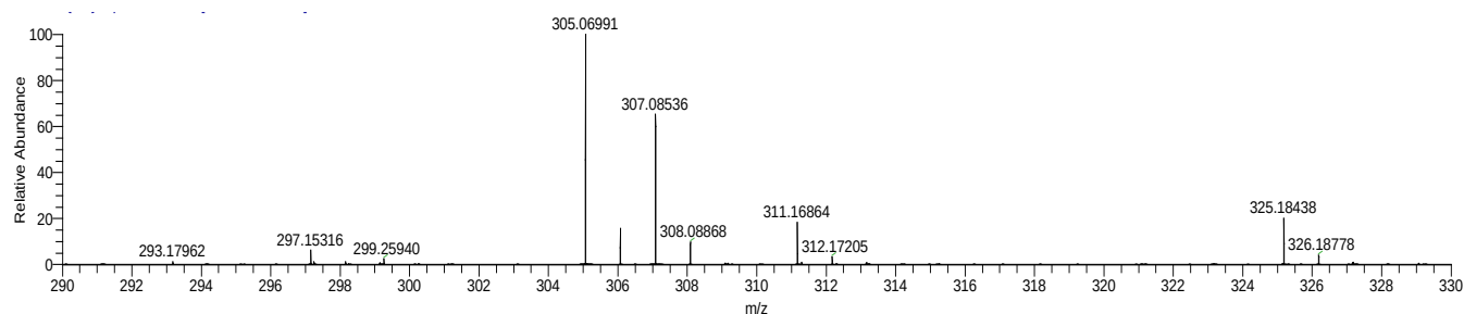
Fig. S20. High-resolution mass spectrum of 3d C_{14}H_{14}N_2O_4P [M - C_6H_{16}N(TEA)]^- : 305.06967.
