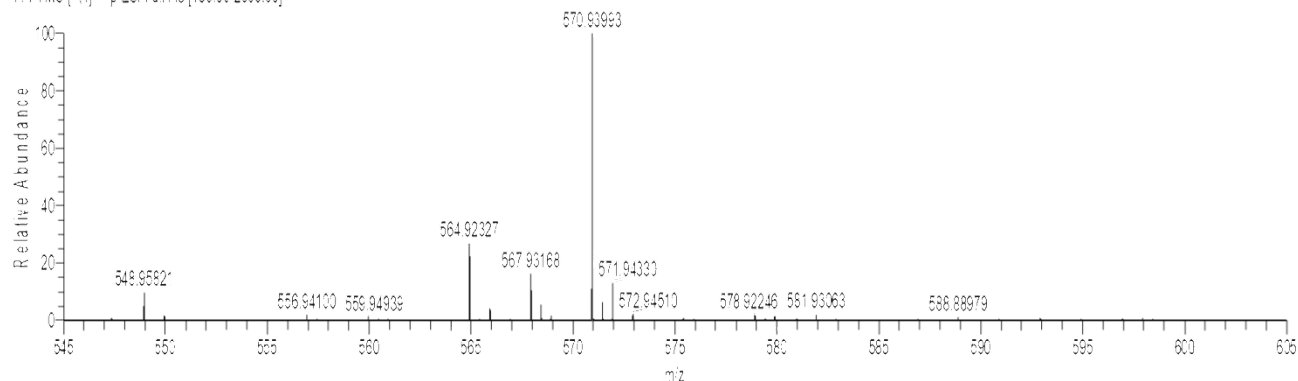
Fig. S11. High-resolution mass spectrum of AzoethoxyTP ( 4b ) as tetrasodium salt calculated for C_{14}H_{14}N_2O_{11}Na_4P_3 [M + H]^+ : 570.93957
