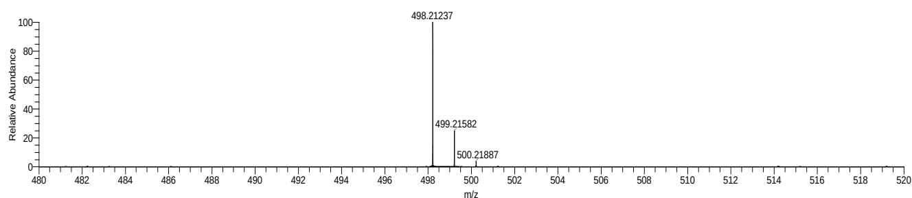
Fig. S15. High-resolution mass spectrum of 2c calculated for C_{24}H_{34}N_3O_5P [M + Na]^+ : 498.21283.
