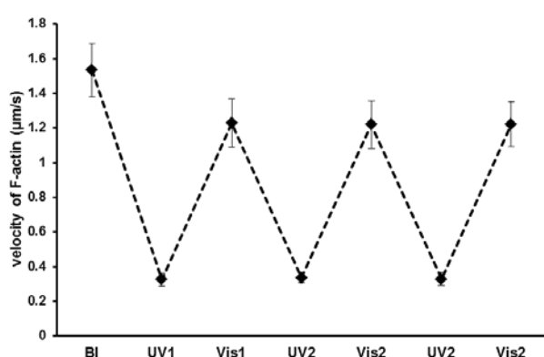
23 24 Fig. 2. Repeatability of the complete and reversible photoregulation of F-actin gliding velocity induced by 4b 25 (AzoethoxyTP) at saturated concentration (0.25 mM). (BI: before irradiation; UV: after irradiation with 365 nm light; 26 Vis: after irradiation with 436 nm light). Error bars: standard deviation for 10 actin filaments.
