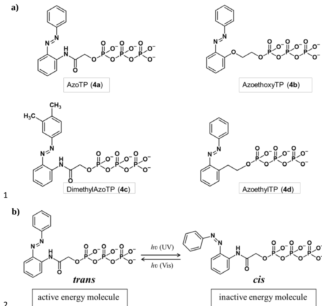
Fig.1. a) Structures of azobenzene based non-nucleoside triphosphates, AzoTP ( 4a ), AzoethoxyTP ( 4b ), DimethylAzoTP ( 4c ) and AzoethylTP ( 4d ). b) Reversible photo-isomerization of 4a .
