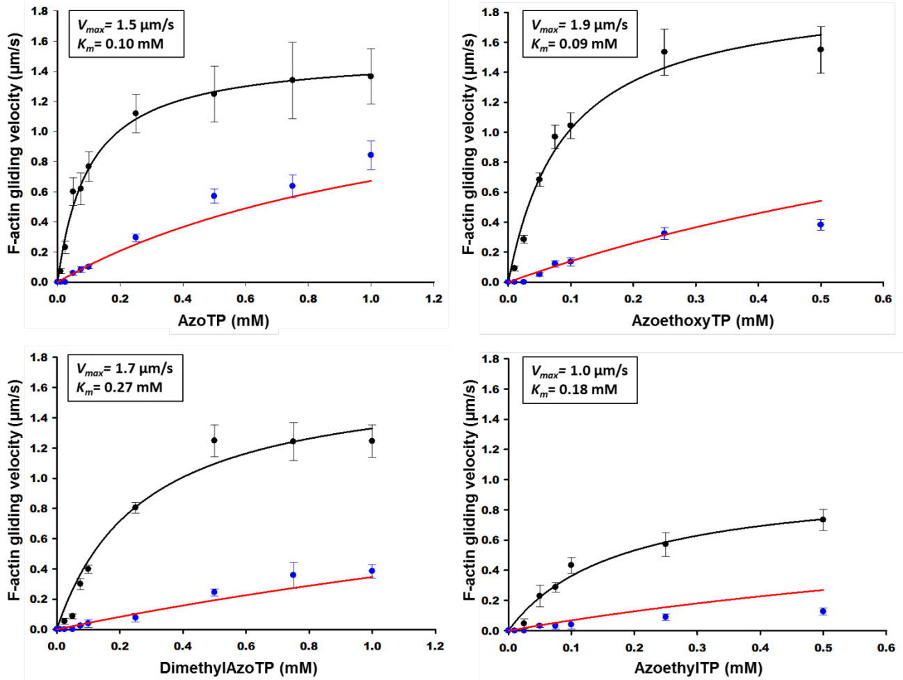
15 16 Fig. 4. Gliding velocity of actin filaments as a function of AzoTPs concentration. (Black solid circles: velocities before 17 irradiation; black line: curve fitted using Michaelis–Menten equation; Blue circles: velocities after irradiating at 365 nm;
