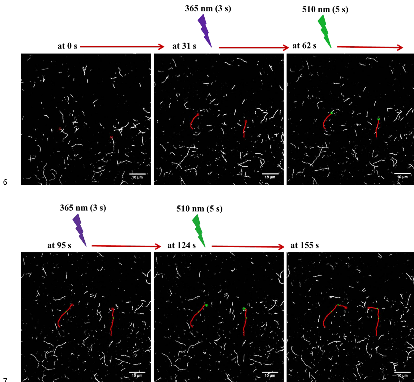
8 Fig. 3. Fluorescence images of F-actin motility driven by trans and cis state of 4a (40 \mu M) by in-situ photo-regulation 9 experiment with alternating irradiation at 365 nm (3 s) and 510 nm (5 s). The distance moved by two actin filaments is 10 indicated in lines by tracking the path of filament heads; red circles denote the position of actin filament heads before 11 irradiation ( trans state), green and red lines denote the distance treaded by F- actin after UV (365 nm) and Vis (510 nm) 12 irradiations respectively.
