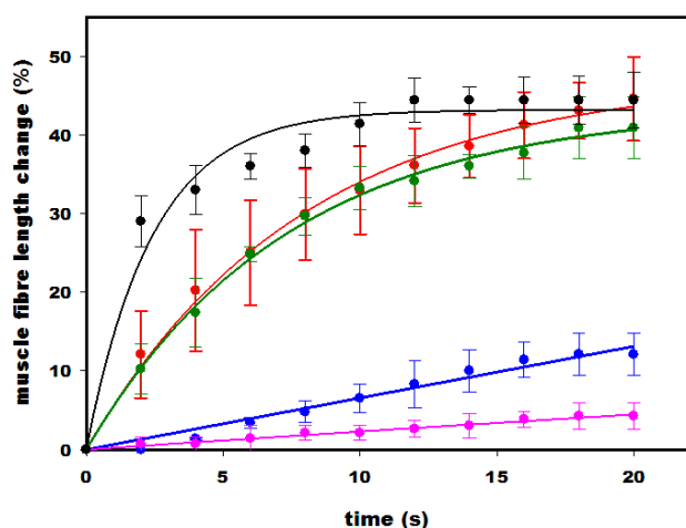
Fig. 6. Muscle fibre length change ( (L_{(t=0)} - L_{(t)}) / L_{(t=0)} ) with respect to the time for AzoTPs (3 mM) 4a , 4b , 4c and 4d induced fibre shortening. Black, red, green, blue and pink circles represent the % length change induced by ATP, 4a , 4b , 4c and 4d respectively; the lines are best-fit through the data trend. Error bars: standard deviation for 4 fibres.
