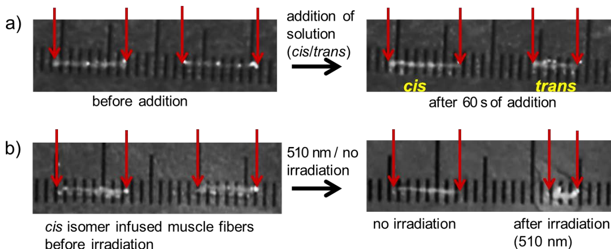
Fig. 5. Non-nucleoside triphosphate 4a induces and photo-controls the shortening of glycerinated muscle fibre. a) buffer solution with trans - 4a (3 mM) induces shortening while cis - 4a has no significant effect on shortening. b) cis - 4a infused muscle fibre shortens after irradiation with 510 nm light, no significant change in length in non-irradiated fibre. Red arrows point at the two edges of the fibre. The scale seen in the photographs is 1 mm.
