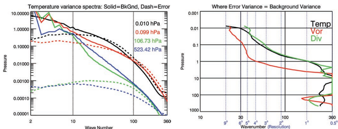
Figure 8: (left) Average power spectra for temperature forecast (solid line) and temperature analysis error (dashed lines) for several pressure levels. (right) Limit of predictability, defined as the wavenumber where the error variance exceeds the forecast variance. Analysis errors for temperature (black), vorticity (red), and divergence (green) were estimated as the difference between two December 2011 analyses produced from a random-observation denial experiment. (Provided by Karl Hoppel).
