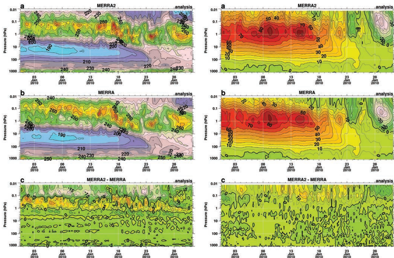
Figure 7: Time series of temperature averaged from 60°N-90°N (left) and zonal wind at 60°N (right) from MERRA-2 (top), MERRA-1 (middle), and their differences (bottom), for January 2010 when a stratospheric sudden warming occurred. (Provided by Lawrence Coy).
