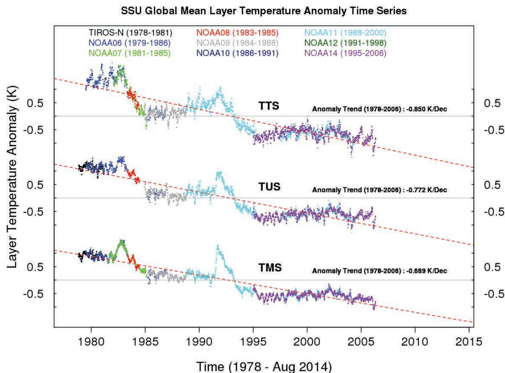
Figure 9: SSU global mean anomaly time series and trends for layer temperatures of mid-stratosphere (channel 1), upper-stratosphere (channel 2), and top-stratosphere (channel 3) after recalibration and adjustment of multiple instrument drifting effects of the level 1c radiances. (Provided by Cheng-Zhi Zou).
