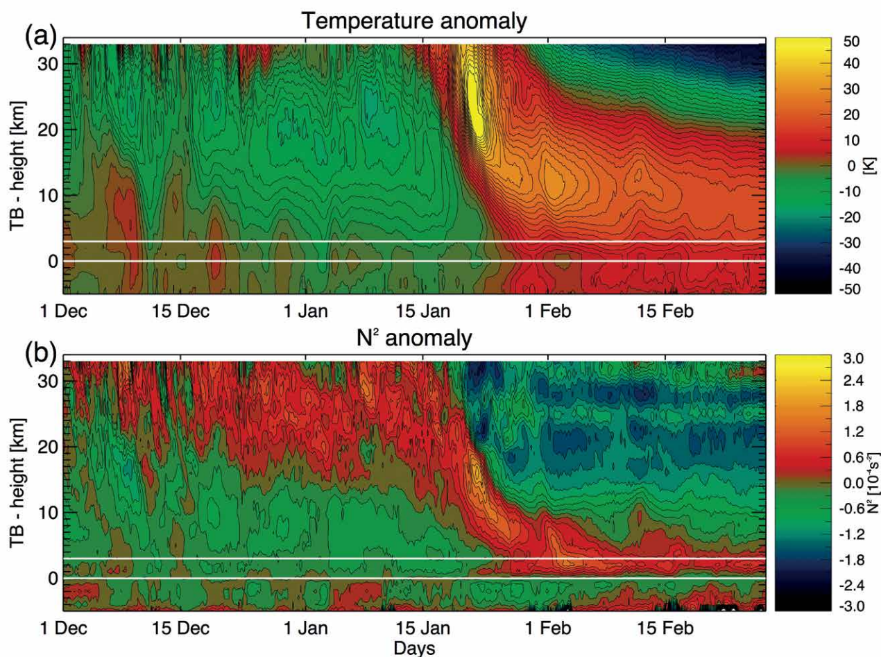
Figure 6: Temperature anomaly (top) and Brunt-Väisälä buoyancy frequency squared ( \text{N}^2 , bottom) zonally averaged between 75-90°N from MERRA-2 reanalysis.
