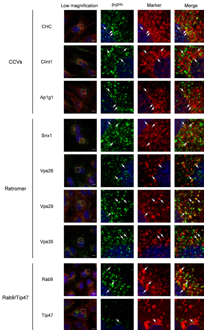
Figure 2. Co-localization of PrP Sc with the components of machineries involved in retrograde transport from the endosomes to the TGN in ScGT1-7-22L cells. ScGT1-7-22L cells grown on the Chambered Coverglass for 96 h were subjected to IFA to monitor PrP Sc and the component molecules of CCVs, as well as those of the retromer complex and Rab9/Tip47 pathway. The leftmost column shows lower magnifications of merged images of PrP Sc (green), the component molecules (red), and nuclei (blue). Individual and merged high-magnification images of the boxed regions are shown on the right. The arrows indicate representative examples of areas where PrP Sc and the corresponding component molecules are co-localized. The co-localization areas were defined as pixels that were positive for both PrP Sc signals and signals of the corresponding component molecules. The ratios of PrP Sc signals co-localized with the signals of corresponding component molecules relative to the total signals of PrP Sc are shown in Supplementary Fig. S1b. Scale bars: 10 \mu m.
