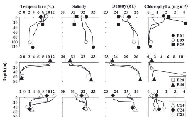
Fig. 2. Vertical profiles of temperature, salinity, density, and chlorophyll a in the southeastern Bering Sea (upper), northern Bering Sea (middle), and Chukchi Sea (lower) during 24 July–11 August 2007.
