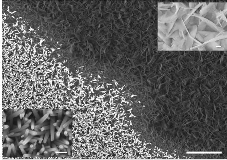
Fig. 2. SEM image of the boundary between the ZnO nanowire area (bottom-left) and nanosheet area (top-right). The scale bar is 5 μm in length. Inset: magnified SEM images of nanowires (bottom-left) and nanosheets (top-right). The scale bar in either inset is 200 nm.
