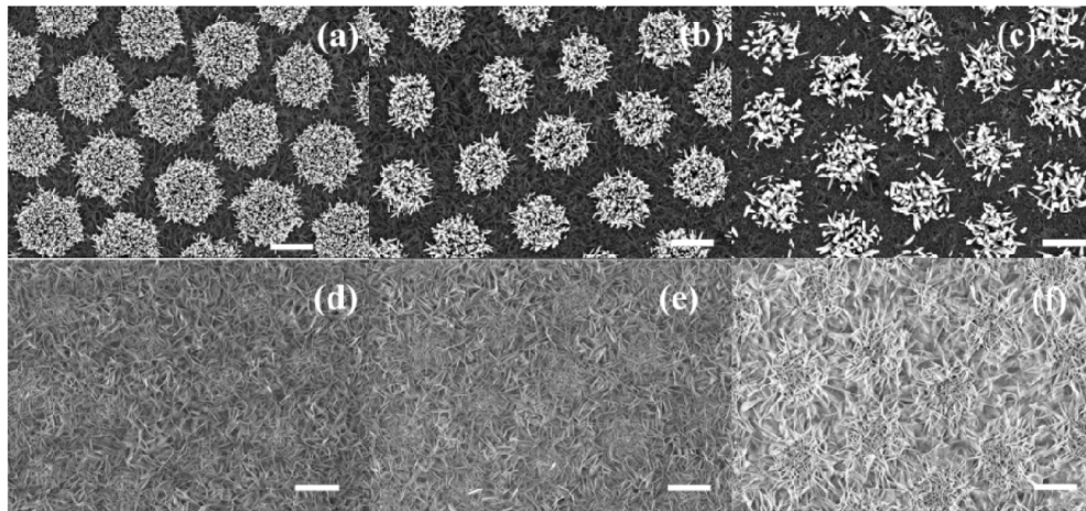
Fig. 4. SEM images of controllable periodic pattern of ZnO nanowires/nanosheets. The Al nanohole size is decreasing from panel a to panel f . For smaller hole size (panel d-f ), ZnO nanowires are prevented from growing and ZnO nanosheets prevail. The scale bars in all panels are 2 \mu\text{m} in length.
