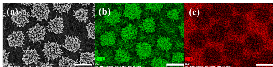
Fig. 6. SEM image of ZnO nanowire/nanosheet pattern (a) and the corresponding Zn (b) and O (c) distribution map obtained with EDS. The scale bars in all panels are 4 \mu\text{m} .
