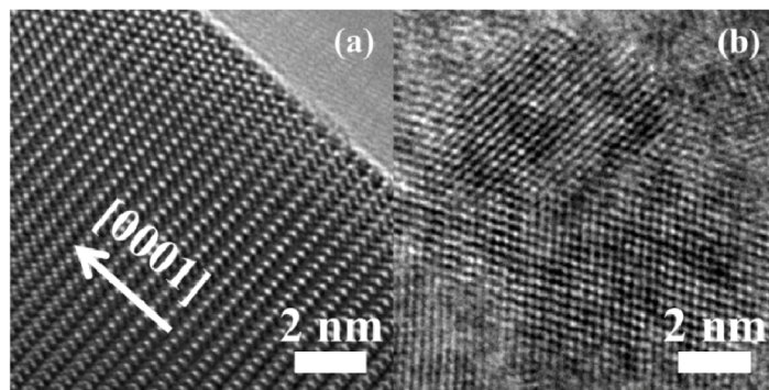
Fig. 7. High resolution TEM images of ZnO (a) nanowire and (b) nanosheet.
