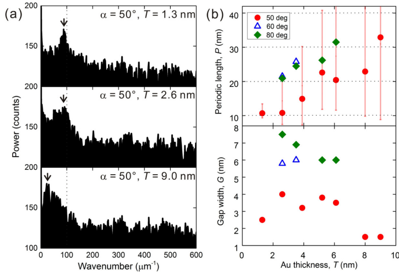
Fig. 2. (a) Power spectra obtained by two-dimensional Fourier transform of the SEM images of the samples deposited at \alpha = 50^\circ and T = 1.3 (top), 2.6 (middle), and 9.0 nm (bottom), collected along the line perpendicular to the grating. The arrows indicate the peaks corresponding to the periodic length ( P ), and the vertical dotted line denotes P = 10\text{ nm} , the periodicity of the MPS. (b) Relation between the Au thickness T , and P (top panel) and the gap width, G (bottom panel). The circles, the triangles and the squares represent the data for the samples deposited at \alpha = 50, 60 , and 80^\circ , respectively. The vertical red lines denote the variation in P estimated for the samples with \alpha = 50^\circ from the width of the peak in (a).
