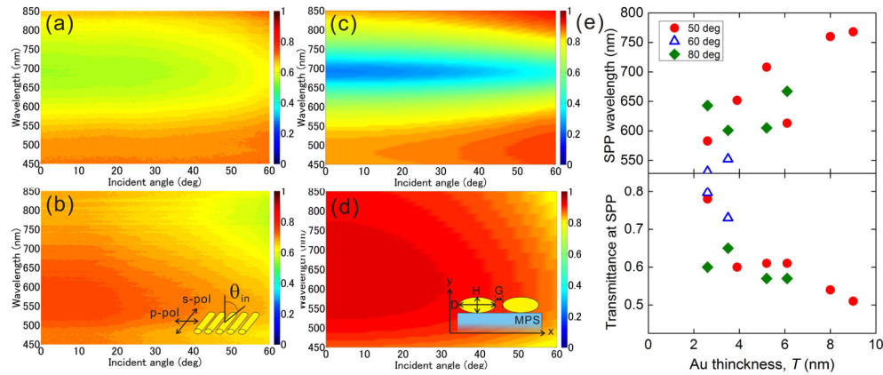
Fig. 3. Transmission spectra as a function of angle of incidence for the sample deposited at \alpha = 50^\circ with T = 5.2 nm for (a) p- and (b) s-polarized light. The inset in (b) is the sketch of the experimental geometry. Simulated transmission spectra for (c) p- and (d) s-polarized light. The model is a two-dimensional periodic array of Au nanorods with diameter ( D ) = 24 nm, height ( H ) = 3.5 nm and gap width ( G ) of 4 nm, deposited on the 500 nm thick MPS substrate with an effective refractive index of 1.11. The inset in (d) shows the schematic illustration of the model with the coordinate x and y axes. (e) Relation between T , and the wavelength of SPP (top panel) and the optical transmission at the wavelength of SPP (bottom panel), for p-polarized light.
