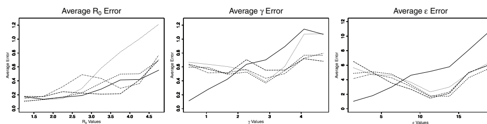
FIGURE 1 | Average error for ABC (solid line), CNN (long dashed line), MLP (dotted line), MLP with time (dashed line), and LSTM (dashed and dotted) estimates against actual parameter values for an SEIR model with three parameters, on 100,000 training datasets.
