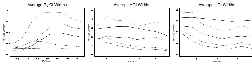
FIGURE 3 | Average credible/confidence interval width for ABC (solid line), CNN (long dashed line), MLP (dotted line), MLP with time (dashed line), and LSTM (dashed and dotted) estimates against actual parameter values for an SEIR model with three parameters, on 100,000 training datasets.
