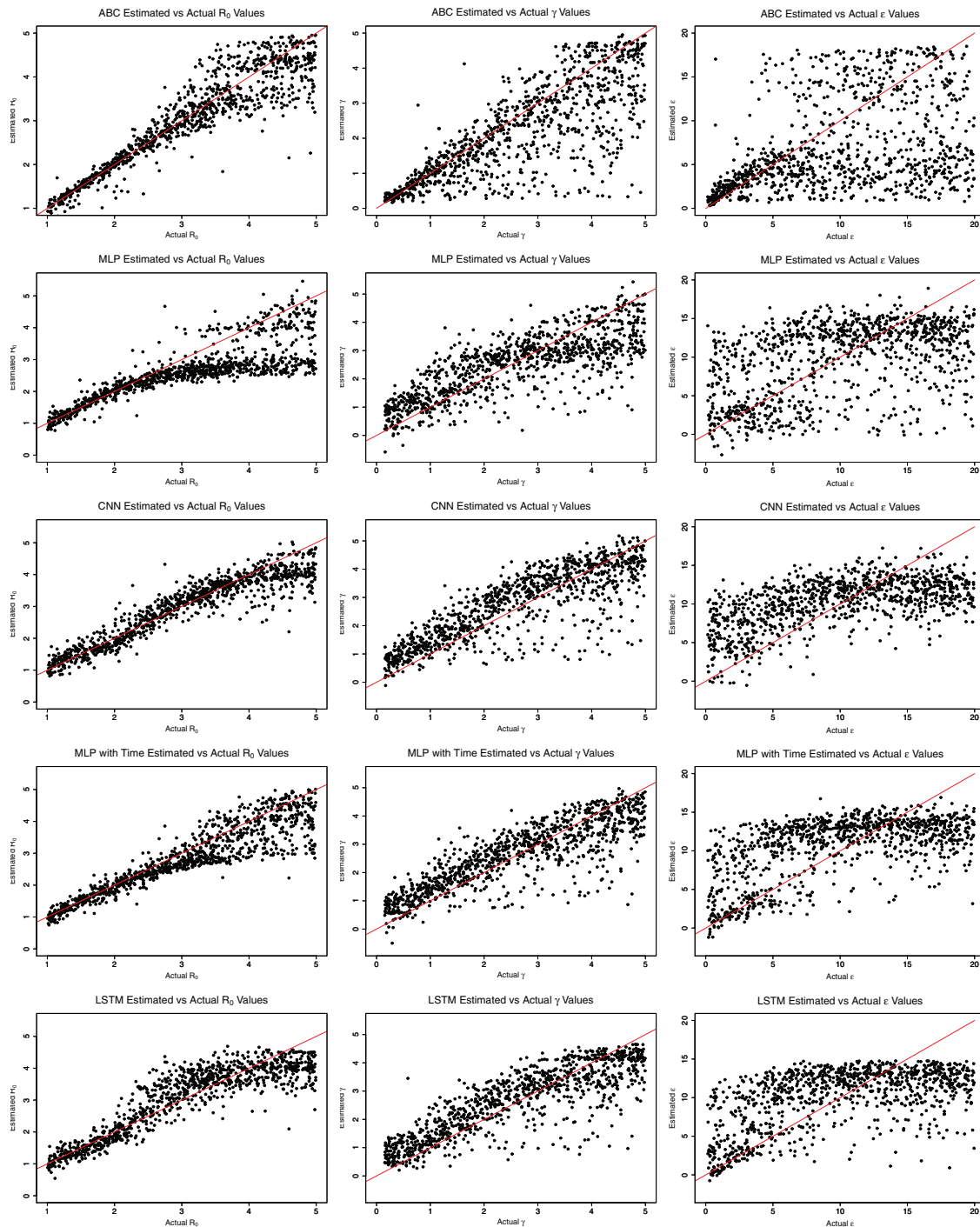
FIGURE 4 | The estimated and actual parameter values from ABC, MLP, CNN, MLP with time, and LSTM.
