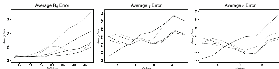
FIGURE 2 | Average error for ABC (solid line), CNN (long dashed line), MLP (dotted line), MLP with time (dashed line), and LSTM (dashed and dotted) estimates against actual parameter values for an SEIR model with three parameters, for one million training datasets.
