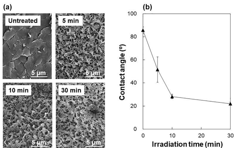
Fig 7. SEM images (a) and contact angles of water droplet (b) of the surfaces of the untreated PEEK substrate and those after laser irradiation in ultrapure water at 2 W/cm 2 for 5, 10, or 30 min. Data in (b) are expressed as the average ± standard deviation (n = 3).
