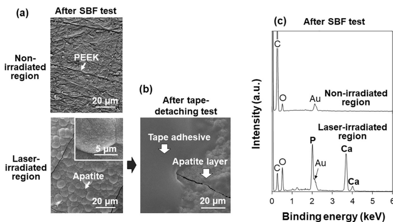
Fig 10. SEM images (a, b) and SEM-EDX spectra (c) of the non-irradiated and laser-irradiated regions of the LAB-processed ( 2 \text{ W/cm}^2 , 30 min) PEEK substrate surface after the SBF test (a, c) and after the subsequent tape-detaching test (b). The Au peak in (c) is due to the gold coating prior to the SEM-EDX analysis.
