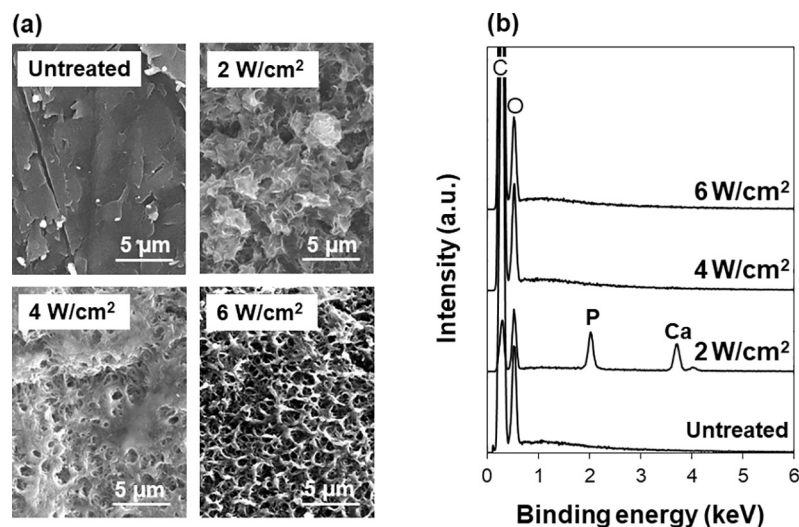
Fig 2. SEM images (a) and SEM-EDX spectra (b) of the surfaces of the untreated PEEK substrate and those after the LAB process at 2, 4, or 6 W/cm 2 for 30 min. The C peak in (b) is due to the carbon coating prior to the SEM-EDX analysis and the base PEEK substrate.
