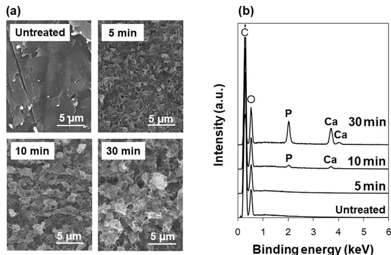
Fig 4. SEM images (a) and SEM-EDX spectra (b) of the surfaces of the untreated PEEK substrate and those after the LAB process at 2 W/cm 2 for 5, 10, or 30 min. The C peak in (b) is due to the carbon coating prior to the SEM-EDX analysis and the base PEEK substrate.
