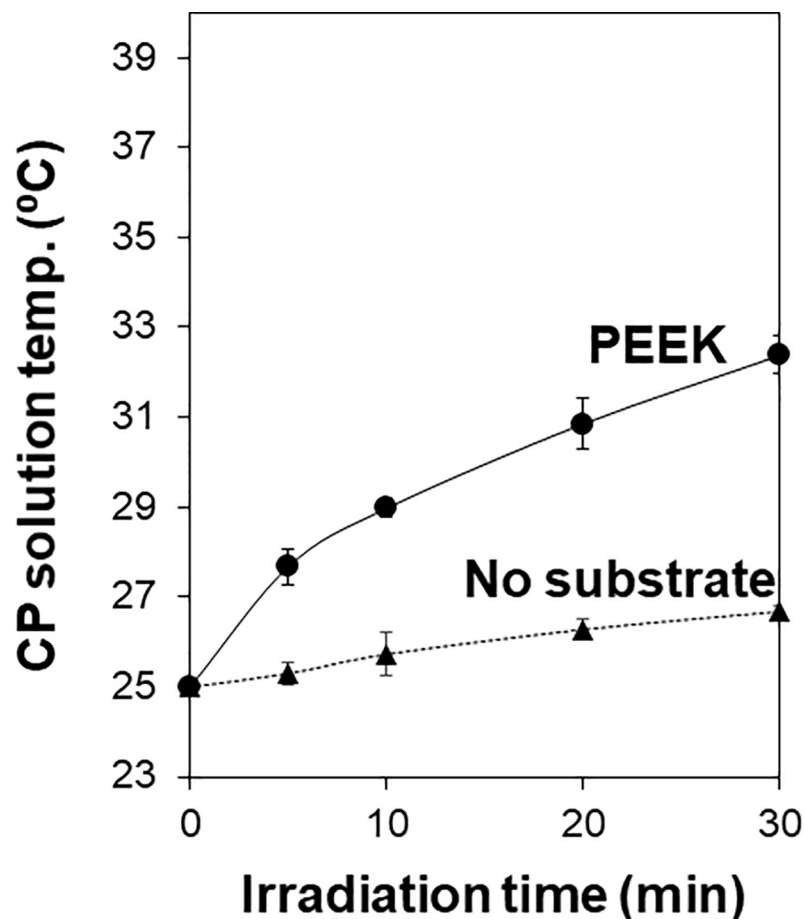
Fig 6. Temperature variations of the CP solution with and without the PEEK substrate during laser irradiation at 2 W/cm 2 without a temperature-controlled water bath. Data are expressed as the average \pm standard deviation ( n = 4 ).
