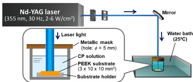
Fig 1. Schematic of the irradiation system of the LAB process for the standard-sized PEEK substrate (3 mm × 10 mm × 10 mm).
