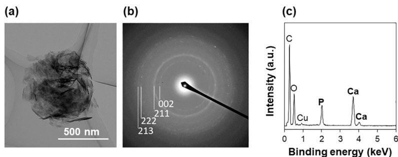
Fig 3. TEM image (a), electron diffraction pattern (b), and TEM-EDX spectrum (c) of the precipitate scraped from the surface of the LAB-processed (2 W/cm 2 , 30 min) PEEK substrate. Rings observed in (b) were indexed to hydroxyapatite (JCPDS No. 09–0432).
