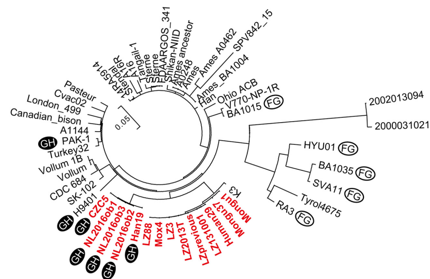
FIG 5 Phylogenetic tree of Zambian and non-Zambian strains of B. anthracis . Zambian strains are indicated in red and bold letters. Strains with the DelFG deletion are indicated by “FG” in a white circle. Strains with the DelGH deletion are indicated by “GH” in a black circle.
