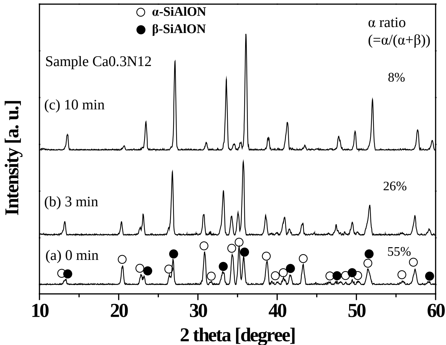
Fig. 5 XRD patterns of \text{Ca}_{0.3}\text{N}_{12} sintered at 1600\text{ }^{\circ}\text{C} for: (a) 0 min: no holding, (b) 3 min and (c) 10 min.
