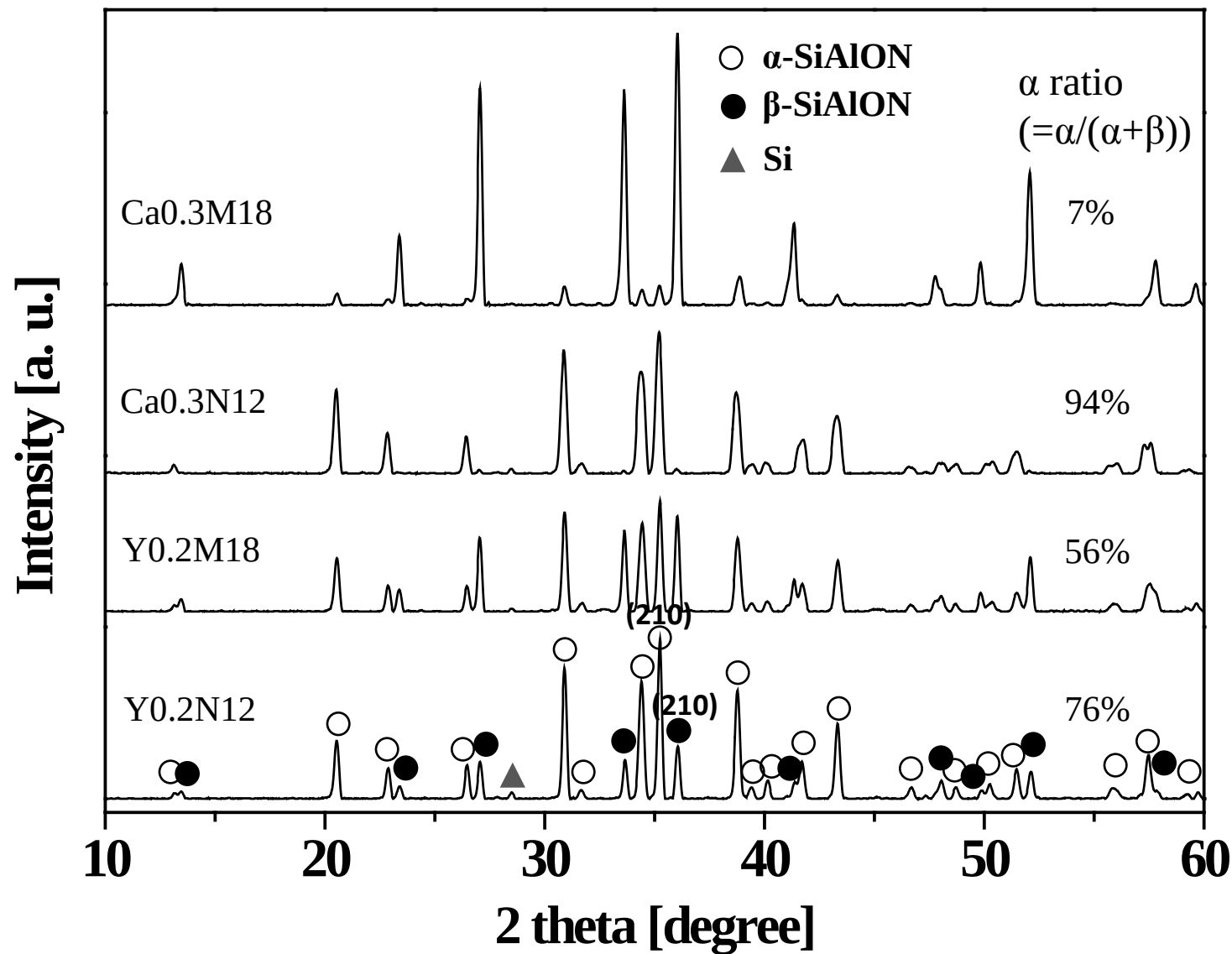
Fig. 2 XRD patterns of combustion synthesized Ca- and Y- \alpha/\beta -SiAlON powders with 12 mass% NaCl (Ca0.3 N12, Y0.2 N12) and 18 mass% \text{MgCl}_2 (Ca0.3 M18, Y0.2 M18) addition.
