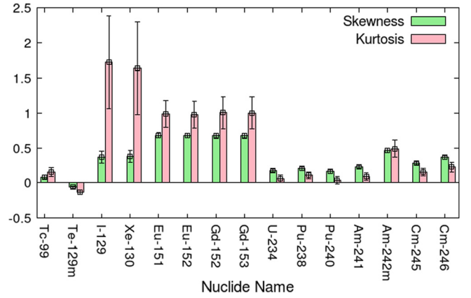
Fig. 3. Skewness and kurtosis of number densities after depletion of several nuclides.
