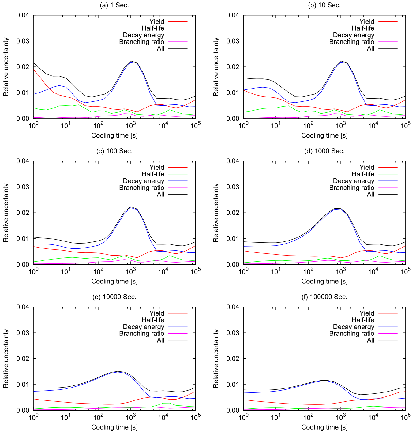
Fig. 7. Nuclear data-induced uncertainty of decay heat after uranium-235 fission with thermal neutrons with different irradiation periods. Default uncertainty is assumed 0%.
