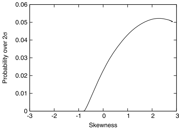
Fig. 2. Relationship between skewness and probability over 2\sigma .
