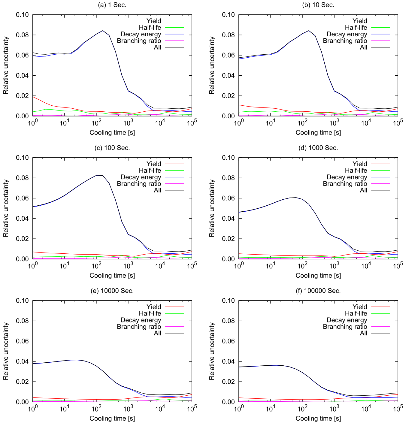
Fig. 6. Nuclear data-induced uncertainty of decay heat after uranium-235 fission with thermal neutrons with different irradiation periods. Default uncertainty is assumed 100%.
