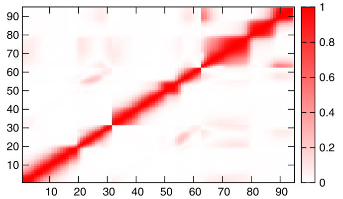
Fig. 5. Correlation matrix of decay heat and \beta -delayed neutron activity after uranium-235 fission by thermal neutrons.
