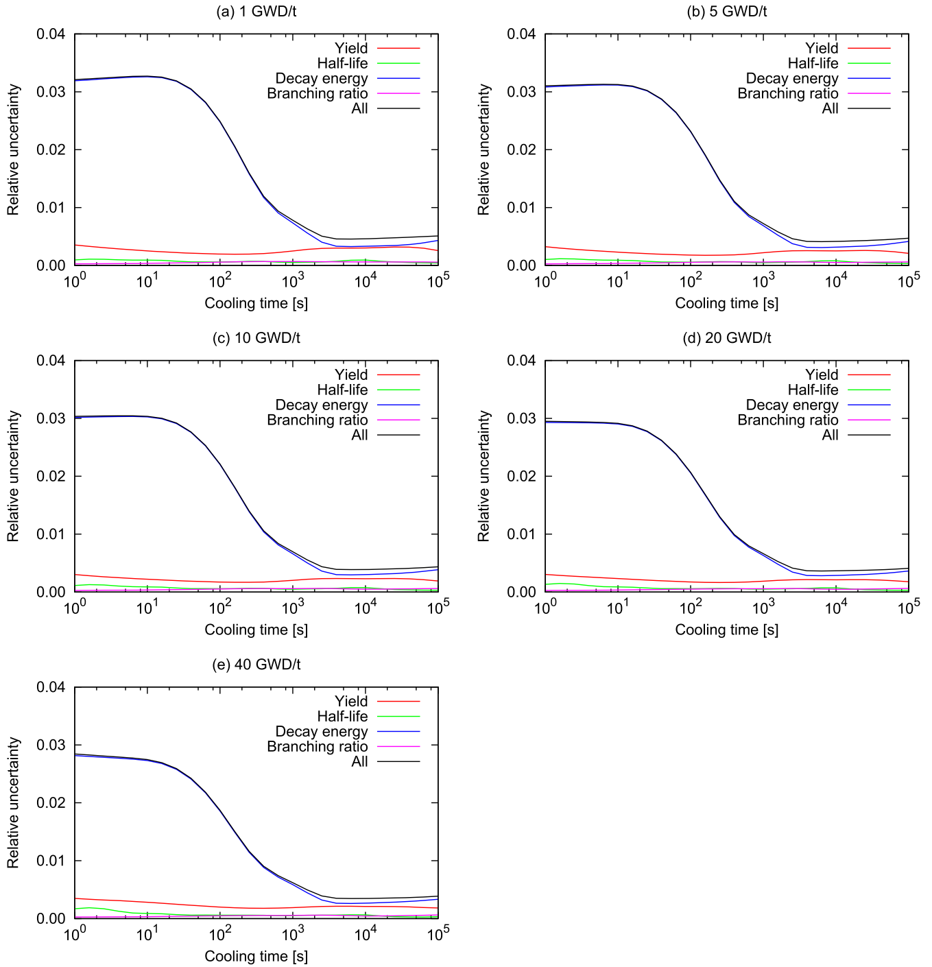
Fig. 8. Nuclear data-induced uncertainty of decay heat after uranium-235 fission with thermal neutrons with different burnup. Default uncertainty is assumed 0%.
