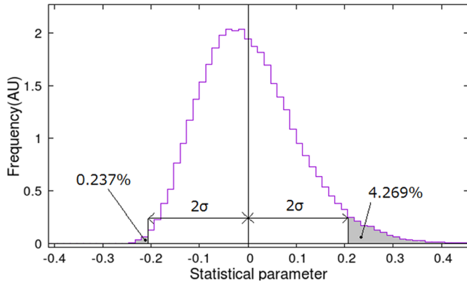
Fig. 1. Example of distorted probability density distribution.
