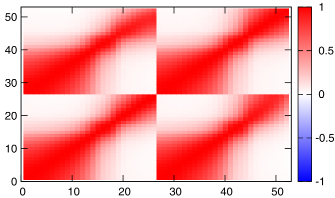
Fig. 9. Correlation matrix of decay heat uncertainties after 100 000-second irradiation and 1 GWD/t burnup.
