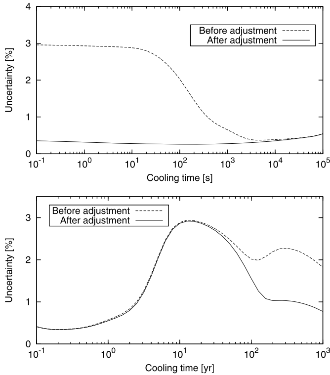
Fig. 4. Nuclear data-induced uncertainty of decay heat. The upper one is the short-term decay heat and the lower is the long-term one.
