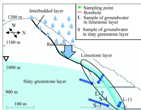
Fig. 10. Groundwater flow paths (blue arrows indicate L-7, L-11, S-3 and S-4 formed by groundwater mixing between the layers; \bigcirc : circled area indicates the sensitive zones).
