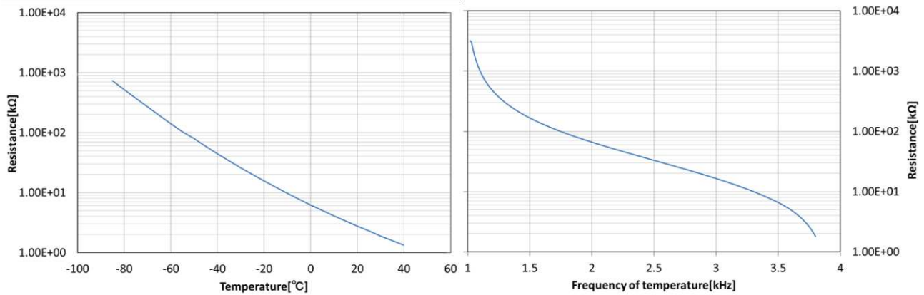
Figure 3.2: An example of the characteristics of the temperature sensor used for the RS-11G radiosonde. (Left) Relationship between the temperature and the resistance of the thermistor. (Right) Relationship between the frequency of temperature and the resistance. The obtained frequency is converted to the resistance, and the resistance is converted to temperature with these relationships.
