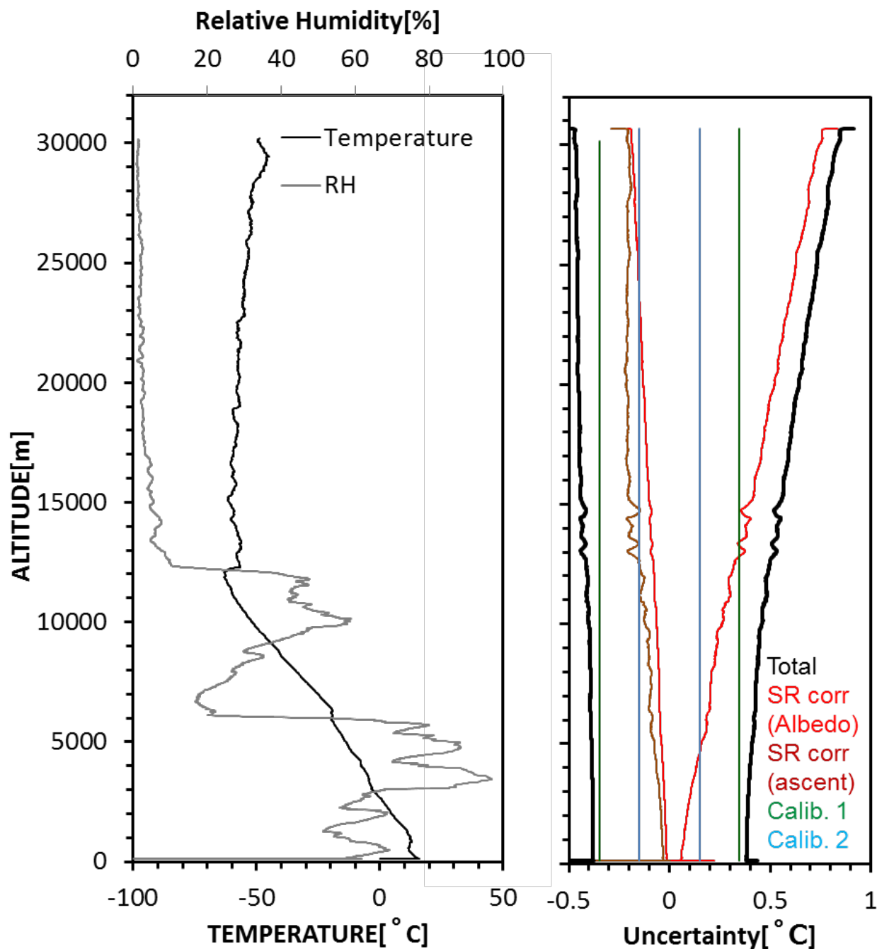
Figure 3.14: Example of the temperature uncertainty profile for the RS-11G radiosonde launched at 14:00 LT on 7 October 2014 at Lindenberg (52.21°N, 14.12°E), Germany. (Left) Profiles of temperature and RH. (Right) Uncertainty of temperature measurement ( k=2 ). Calib. 1 corresponds to the thermistor calibration error, while Calib. 2 corresponds to the component of variability in the calibration chamber in Table 3.1. As shown in Figure 3.9, the uncertainty has different positive and negative values for both SR corr (Albedo) and SR corr (Ascent). Therefore, the total uncertainty is also different for different signs. Also, the SR corr (ascent) only has the negative component because horizontal, pendulum motion is not considered, which would act to further cool the temperature sensor.
