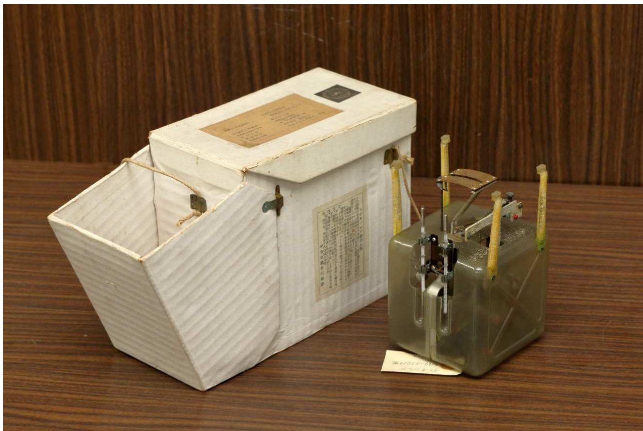
Figure 1.4: Photograph of the S50 type radiosonde. This radiosonde weight was changed to 850g from 1400g of previous type (S49 type).
