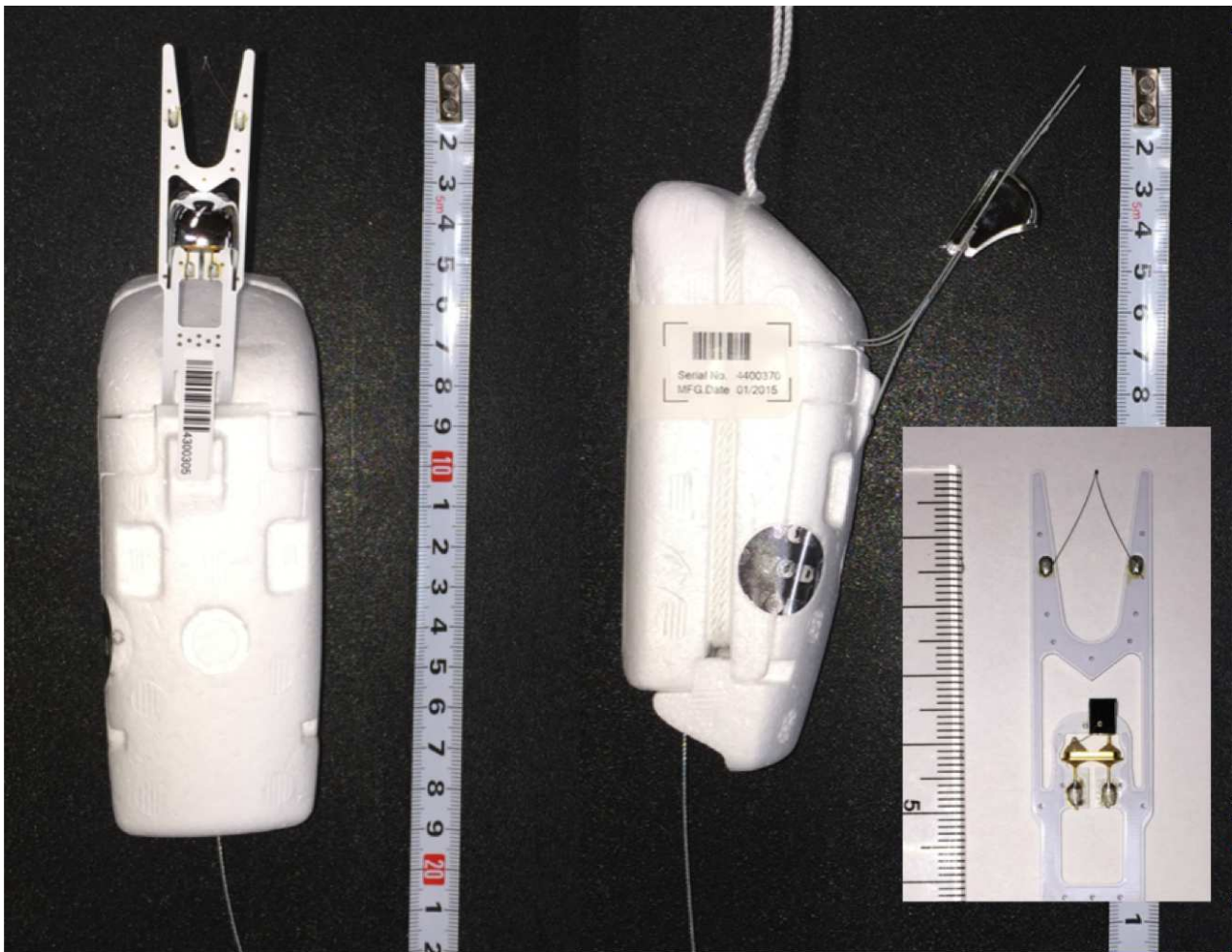
Figure 2.4: Photographs of the iMS-100 radiosonde. The inset at lower right shows a magnified photograph of the sensor boom with the heat type thermistor sensor and thin-film capacitive humidity sensor. The unit of the scales is in cm.
