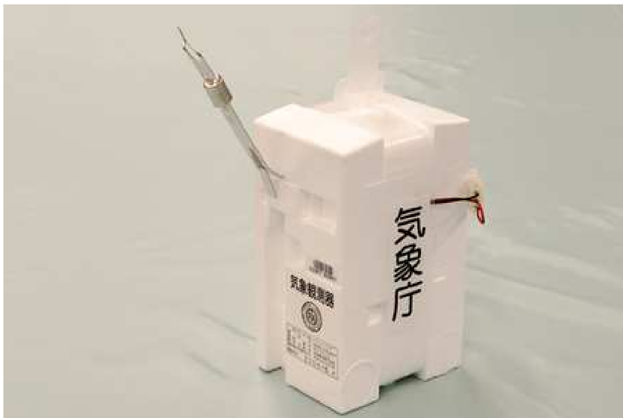
Figure 1.7: Photograph of the RS2-91 type rawinsonde. This type uses an Integrated Circuit in place of transistors.
