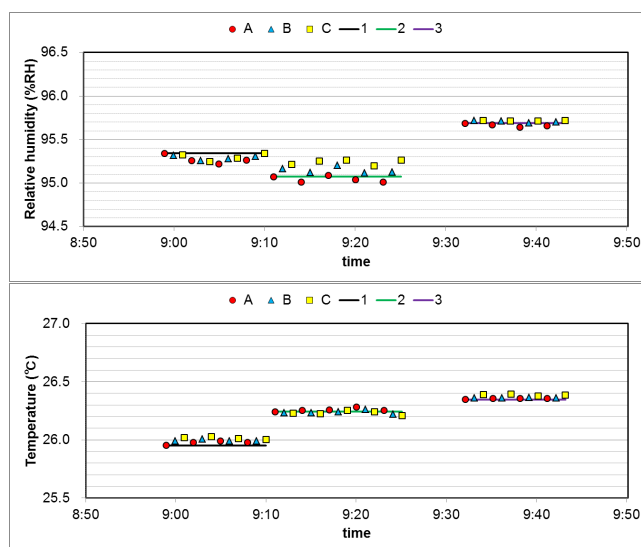
Figure F.13: Same as Figure F.12 but for the anomaly of the one-minute averages with respect to the linear fit (plus the base value) for each period. The first one-minute averages of each period are chosen as the base values for each period.
