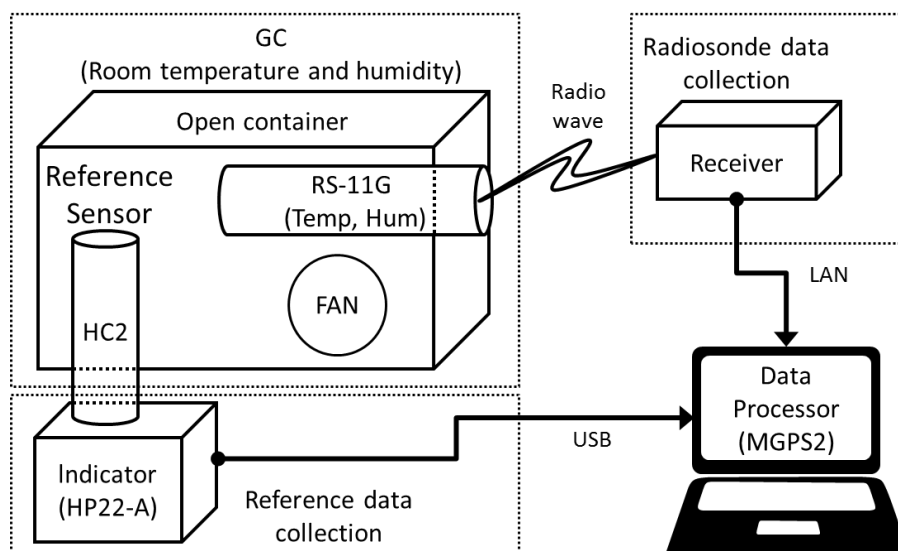
Figure F.3: Schematic diagram of the Meisei's GC system for the RS-11G radiosonde.
