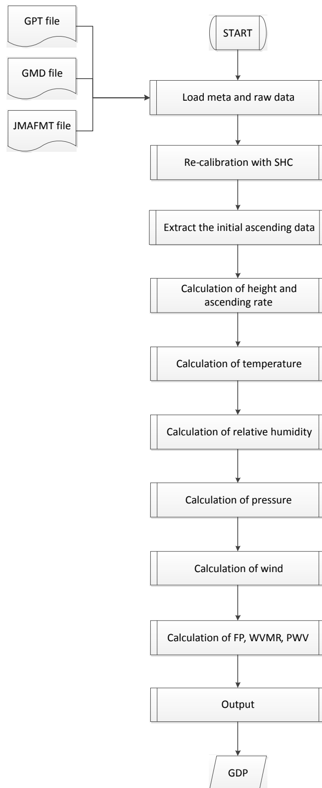
Figure H.1: Overview of the GDP creation workflow.
