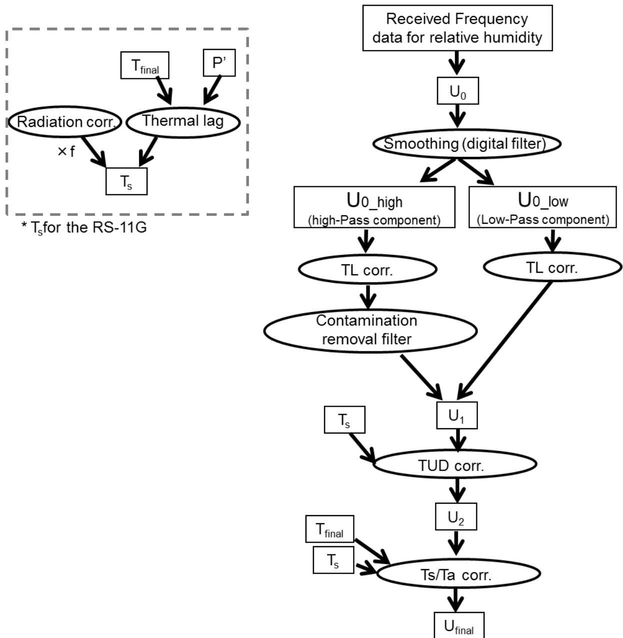
Figure 3.17: Schematic diagram of the processing steps and correction algorithms for the RS-11G and iMS-100 RH measurements in the sounding software MGPS2. The circles indicate processing, and the boxes indicate variables. Shown in the top left dotted box is the process to obtain the RH sensor temperature T_s , only applicable for the RS-11G radiosonde. For the iMS-100 radiosonde, T_s is directly measured with the dedicated thermistor. U_0 is uncorrected RH, P is tentative pressure, T_{final} is the corrected, final temperature, and U_{final} is the corrected, final RH data. U_0 is separated into the high-pass component, U_{0\_high} , and the low-pass component, U_{0\_low} . U_1 is the RH value after the TL correction and contamination removal filter applied. U_2 is the RH value after the TUD correction applied.
