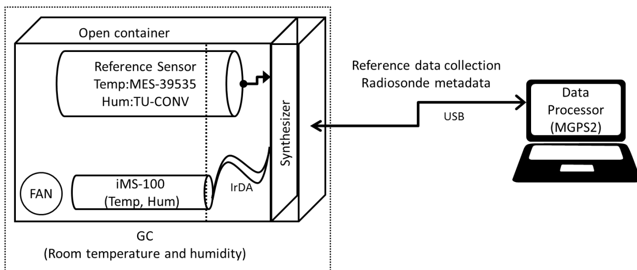
Figure F.5: Schematic diagram of the Meisei's GC system for the iMS-100 radiosonde.
