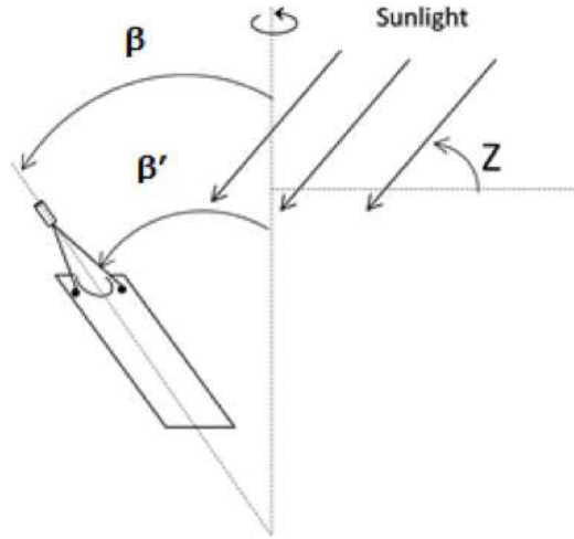
Figure C.2: Schematic illustration of the rotational motions of the radiosonde temperature sensor around the vertical axis.
