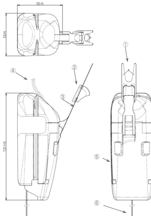
Figure 2.3: External view of the Meisei iMS-100 radiosonde (unit: mm). 1: Temperature sensor; 2: Relative humidity sensor with a cap; 3: Sensor boom; 4: Rope; 5: Styrofoam (EPS) case; and 6: Antenna.
