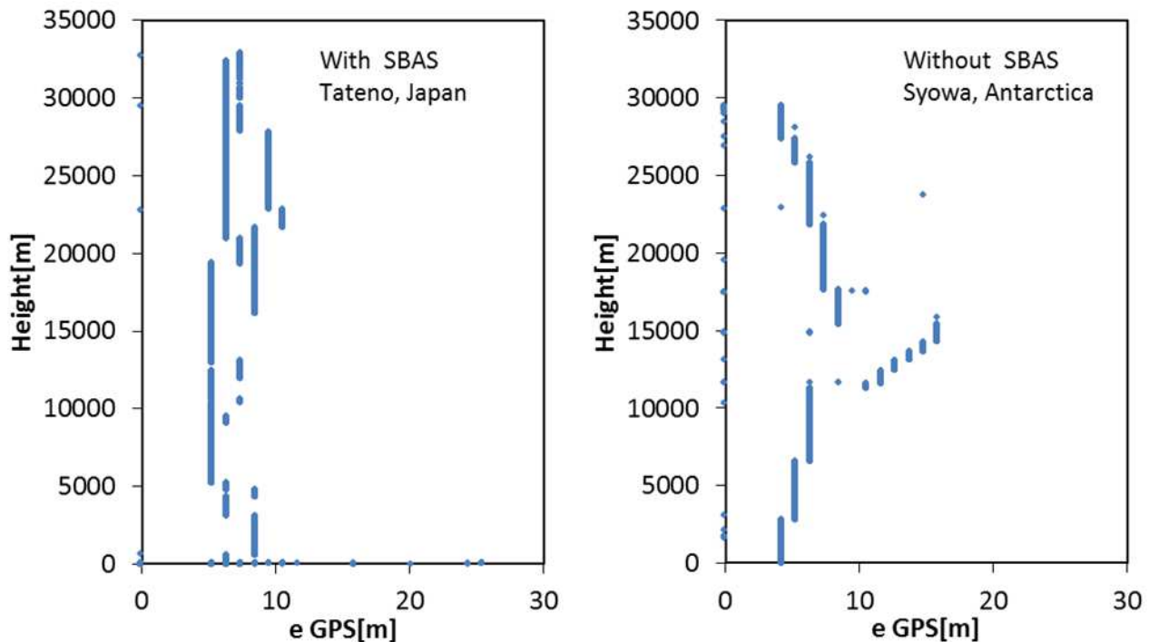
Figure 3.26: Vertical profiles of the 3 dimensional error of GPS geometric height ( e_{GPS} ). (Left) For sounding with the SBAS at Tateno, Japan ( 36.06^{\circ}\text{N} , 140.13^{\circ}\text{E} ) launched at 8:30 LT on 28 May 2014, and (right) for sounding without the SBAS at Syowa, Antarctica ( 69.01^{\circ}\text{S} , 39.59^{\circ}\text{E} ) at 14:30LT on 5 September 2015.
