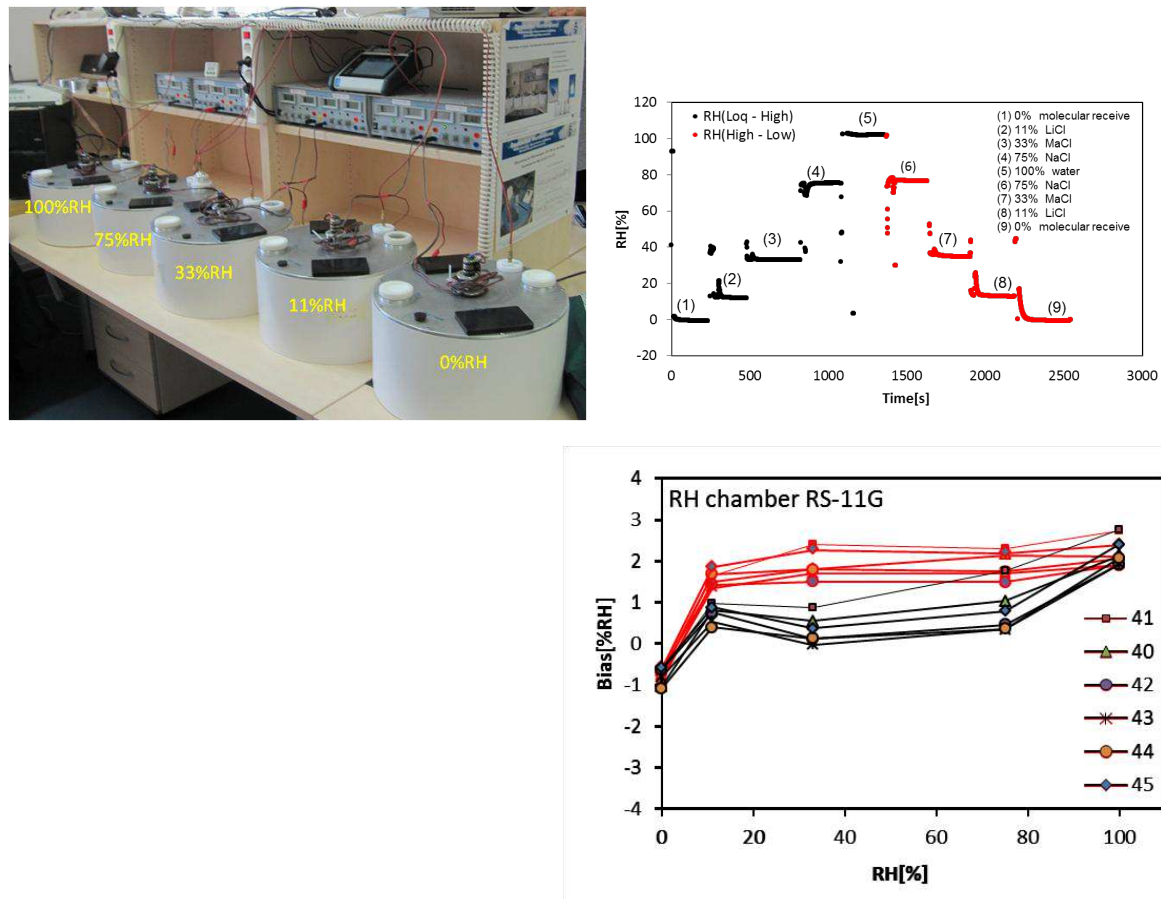
Figure 3.20: (Top left) The experimental setup to investigate the hysteresis of the RS-11G RH sensor. Five chambers of different RH values are prepared by using various saturated salt solutions and pure water. The RH sensor is placed in each chamber for 3 minutes in a dry-to-wet or wet-to-dry order. Six RS-11G RH sensors were investigated. (Top right) An example of a series of experiments using a particular RH sensor. (Bottom right) Summary of the experimental results for all six RS-11G RH sensors (#40 to #45). Black (red) lines indicate the results for dry-to-wet (wet-to-dry) experiments.
