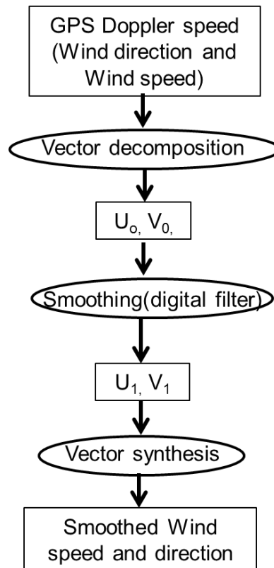
Figure 3.28: Processing steps and correction algorithms for the horizontal wind measurements. Each symbol denotes the following variable: U_0 for the uncorrected zonal wind; V_0 for the uncorrected meridional wind; U_1 for the smoothed zonal wind; and V_1 for the smoothed meridional wind.
