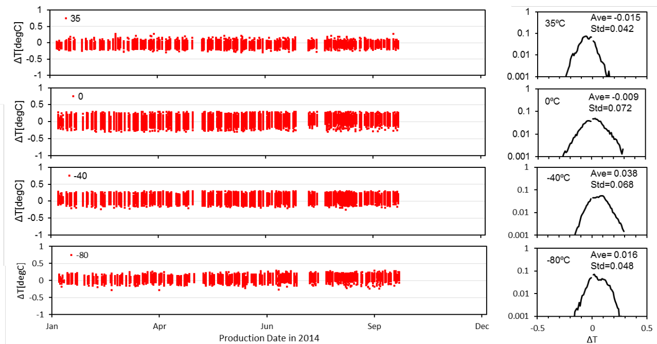
Figure 3.7: Variability of the temperature sensors at the factory calibration process, from top to bottom, +35°C, 0°C, -40°C, and -80°C. (Left) Time series of difference of the temperature measurement of individual radiosonde sensors with respect to the simultaneous measurement of a reference instrument (see Section 5 and Figure 5.1 for the details) during 2014. These data were obtained at the actual production process. All calibration data produced during this period were plotted. (Right) The frequency distribution of the temperature difference.
