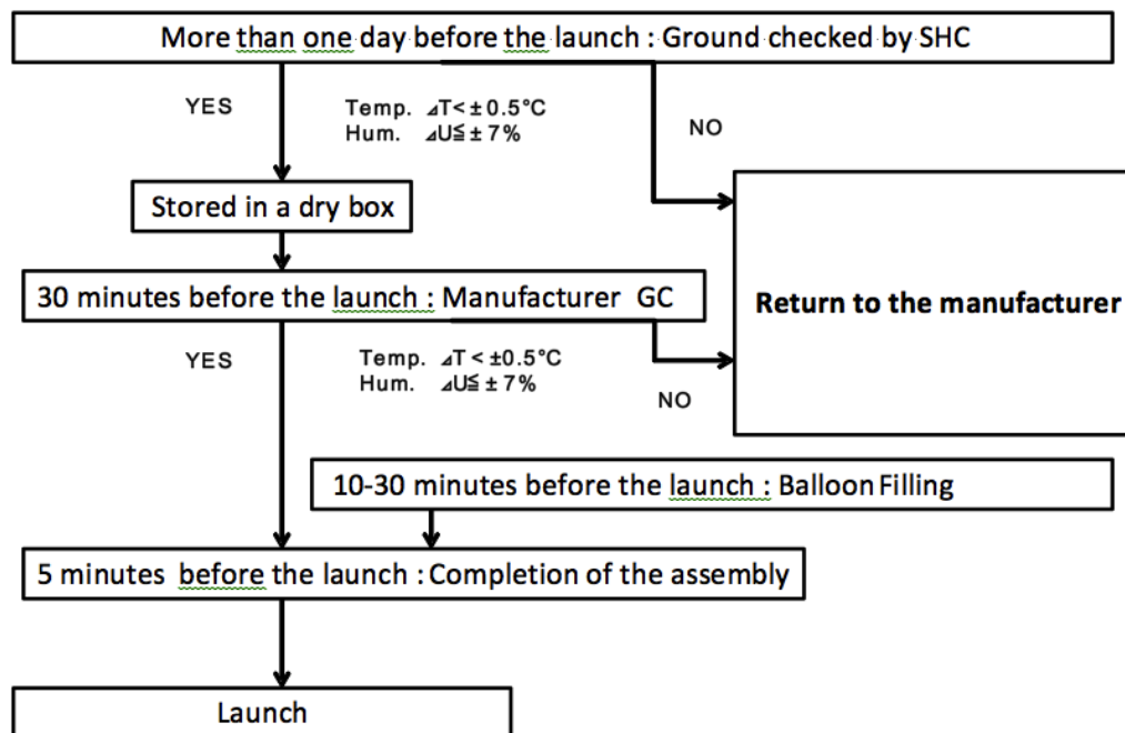
Figure 2.6: Prelaunch procedures for the RS-11G or iMS-100 radiosonde at Tateno.
