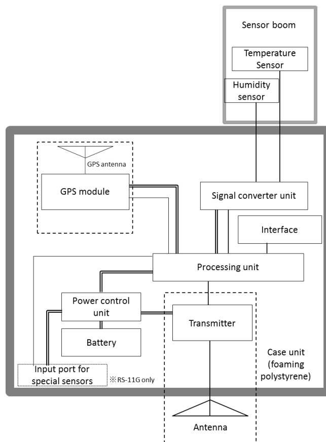
Figure 2.5: System diagram of the Meisei RS-11G and iMS-100 radiosondes. The input port for external sensors is available only for the RS-11G radiosonde. Single lines indicate those for signals, and double lines indicate the power lines.
