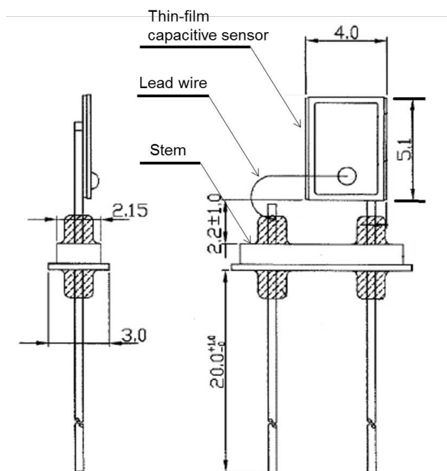
Figure 3.15: Appearance and dimensions of the RH sensor of the RS-11G and iMS-100 radiosondes (unit: mm).
