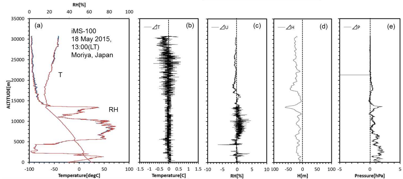
Figure 6.7: As for Figure 6.5, but for a daytime multiple-payload sounding of two iMS-100 radiosondes launched at 13:00 LT on 18 May 2015.
