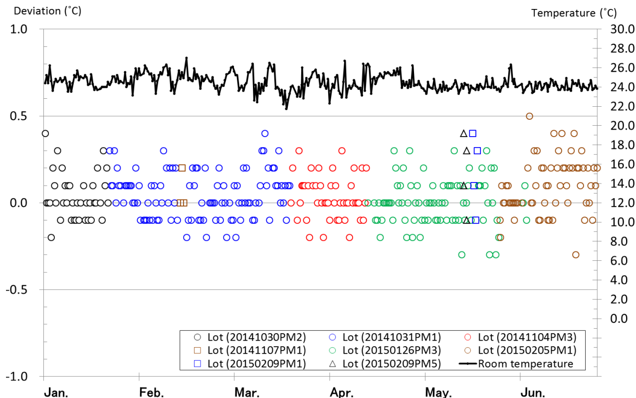
Figure 6.1: Time series of the temperature deviation of radiosonde reading with respect to the standard instrument reading under room temperature conditions (22–27°C, black line) using the manufacturer’s Ground Checker. Different marks indicate radiosondes from different lots.
