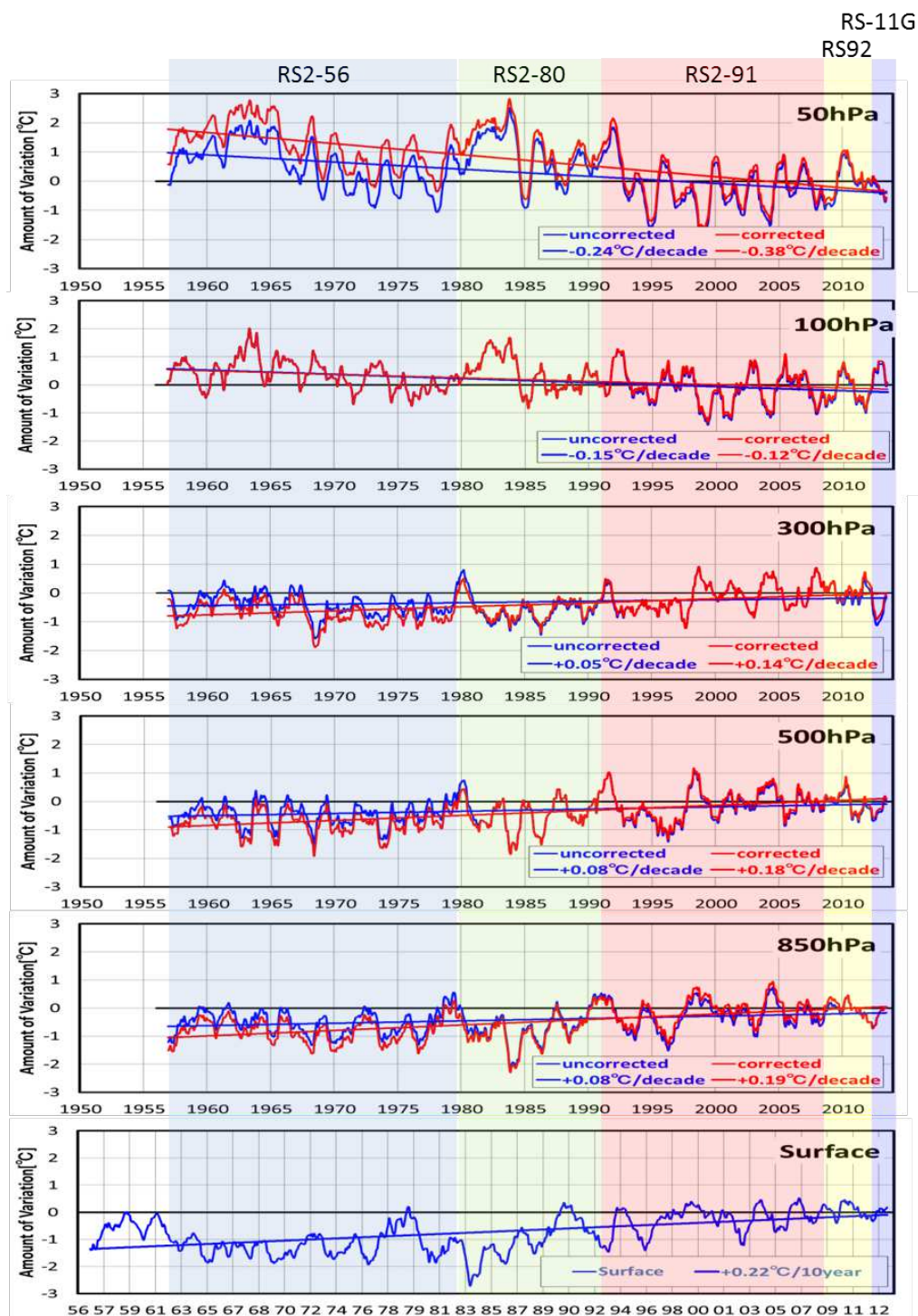
Figure 1.8: Time series of monthly mean temperature at Tateno at six levels. Blue curves are for uncorrected data, while red curves for corrected data using the intercomparison results at the instrument changes. Adopted and updated from Figure 2 of Uesato et al. (2008) .
