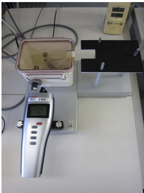
Figure F.4: Photograph of the GC system for the RS-11G radiosonde.
