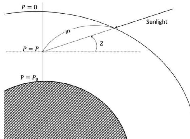
Figure C.3: Atmospheric path length for the solar radiation for a radiosonde located at pressure P.
