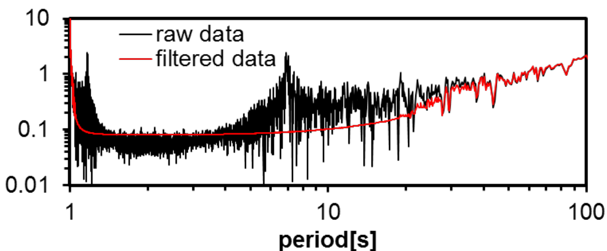
Figure 3.32: Power spectra of the meridional wind between surface and \sim 15 km shown in Figure 3.30. The black line indicates the spectrum for raw data, and the red line indicates the one for filtered data.
