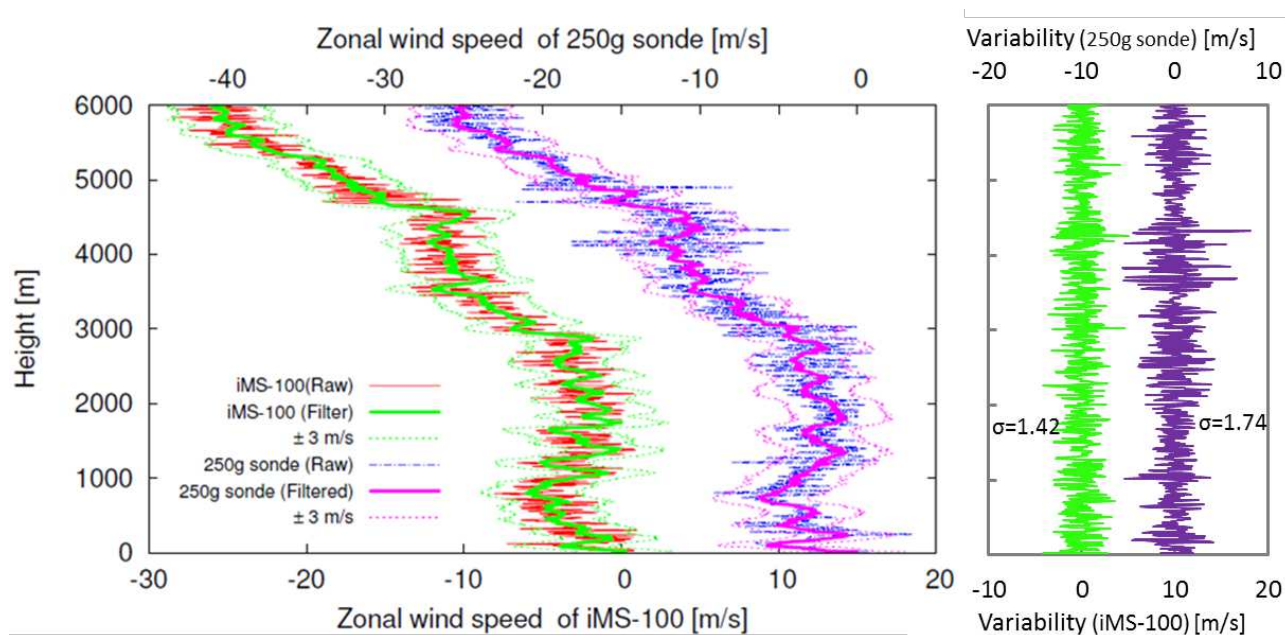
Figure 3.33: (Left) Comparison of zonal wind measurements with the iMS-100 (green line, reference to lower axis) and a 250-g radiosonde (another iMS-100 with a 200-g weight) (purple line, reference to upper axis). Both were launched at Moriya, Japan. The horizontal axes are displaced by 15 \text{ m s}^{-1} . (Right) Corresponding profiles of high frequency component for the iMS-100 (green) and the 250-g radiosonde (purple). The horizontal axes are displaced by 10 \text{ m s}^{-1} .
