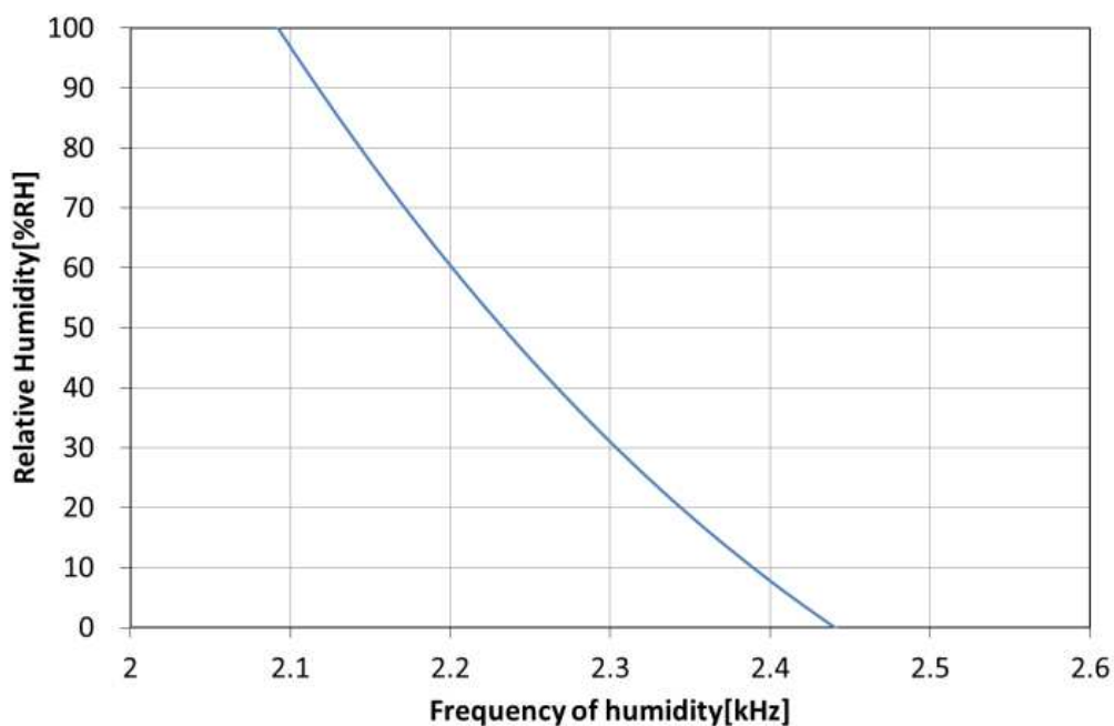
Figure 3.16: Example of the characteristics of a RH sensor used for the RS-11G radiosonde. Shown is the relationship between the frequency and RH at 25°C. The fitted curve is a cubic function.
