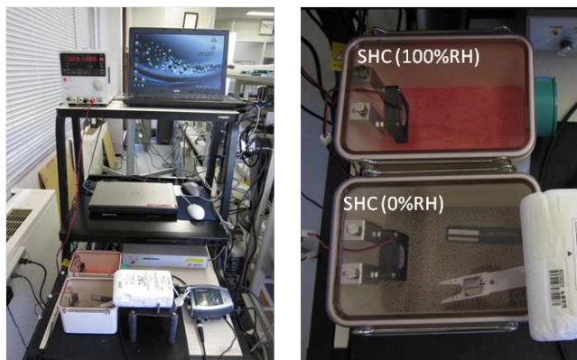
Figure F.2: Photographs of the SHC system. The whole system (left) and the 0 %RH and 100 %RH chambers (right).
