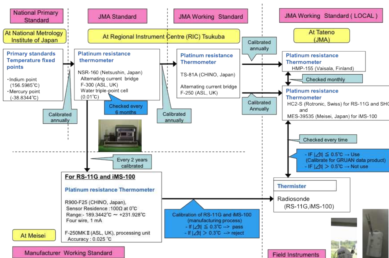
Figure 5.1: Traceability of the temperature sensors on the RS-11G and iMS-100 radiosondes.
