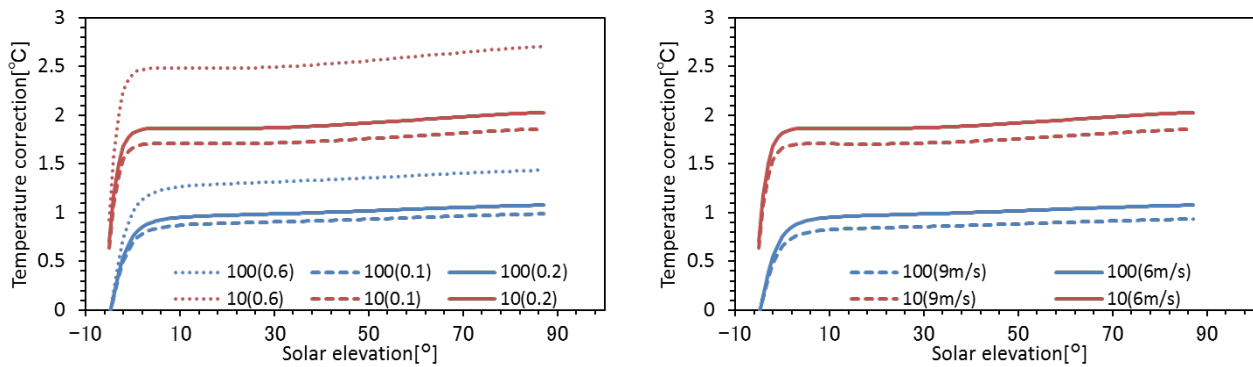
Figure 3.9: Dependence of the solar radiation correction on the assumed albedo and ascent rate (ventilation affect). (Left) The correction amount for albedo of 0.1 (e.g., for sea surface), 0.2 (assumed in the actual correction algorithm), and 0.6 (e.g., under cloudy condition) at pressures of 100 hPa and 10 hPa (see the legends in the panel). (Right) The correction amount for ventilation speeds of 6\text{ m s}^{-1} and 9\text{ m s}^{-1} at pressures 100 hPa and 10 hPa, respectively.
