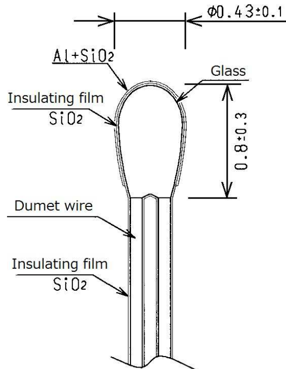
Figure 3.1: Appearance and dimensions of the temperature sensor of the RS-11G and iMS-100 radiosondes (unit: mm).
