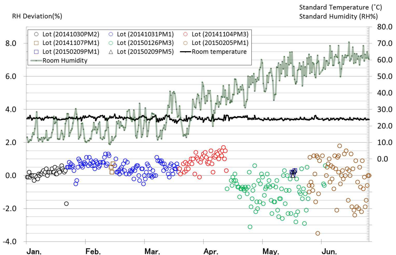
Figure 6.2: Time series of the RH deviation of radiosonde readings from the standard-instrument readings under room RH conditions (10%RH-70%RH, gray line) using the manufacturer's Ground Checker. Different marks indicate radiosondes from different lots.
