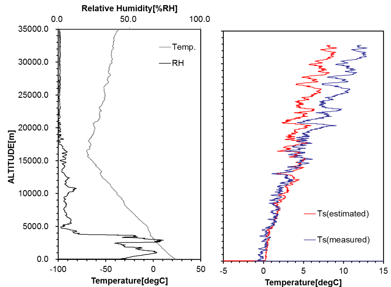
Figure D.1: Temperature profiles of RH sensor for the iMS-100 radiosonde at Moriya, Japan ( 35.9^{\circ}\text{N} , 140.0^{\circ}\text{E} ) launched at 14:30 on 22 September 2014. (Left) temperature and RH profiles from iMS-100 radiosonde, (Right) Blue and red lines indicate the heating amount of the RH sensor measured with dedicated thermistor and that estimated with Equations D.3-D.9.
