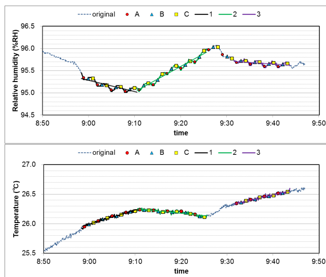
Figure F.12: The HC2 RH (top) and temperature (bottom) data in the SHC(100 %RH) chamber. The measurement data were obtained every 5 seconds (indicated by original). The sensor position was changed sequentially among A, B, and C shown in Figure F.11 every minute. One-minute averages for each position were calculated and shown (indicated by A, B and C). Linear-fit lines are also calculated and shown for three periods, 1, 2, and 3 for both panels.
