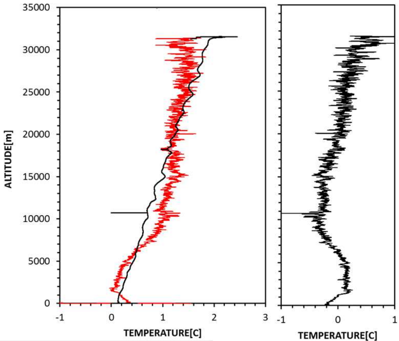
Figure 3.10: (Left) Correction amount for the RS-11G data by the JMA solar radiation correction model (black) and the temperature difference between the MTR and RS-11G results (red) for the multiple-payload flight shown in Figure 3.5 with a 15 m string. (Right) Difference between the two curves in the left panel.
