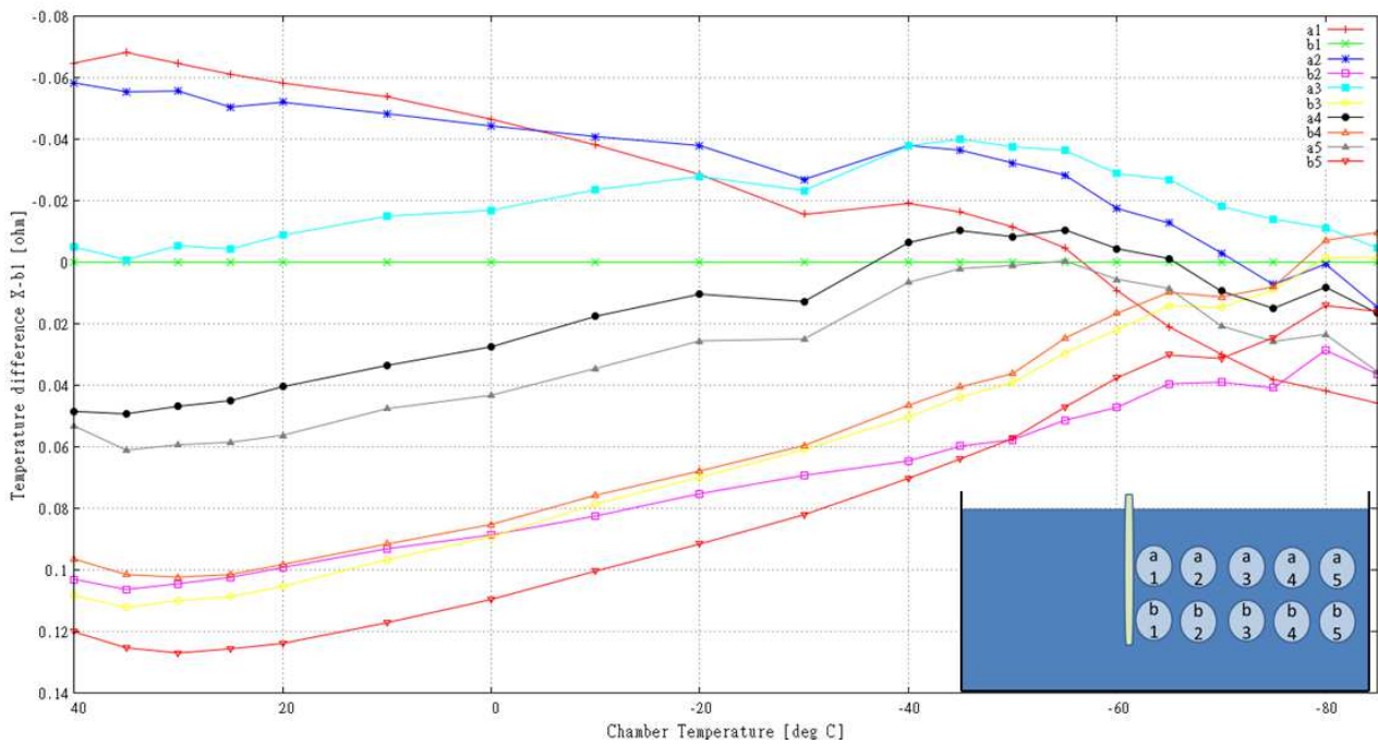
Figure 3.8: Spatial variability in the calibration chamber. The measurement points in the calibration chamber are distributed to 10 areas (a-1 to a-5, and b-1 to b-5) as shown in the schematic. The bar at center indicates the reference thermometer. The thermistors at positions a-1 and b-1 were closest to the reference sensor. Shown are the differences between the measurement at point b-1 and the measurement at the other points in the calibration chamber at various temperatures between +40^{\circ}\text{C} and -85^{\circ}\text{C} .
