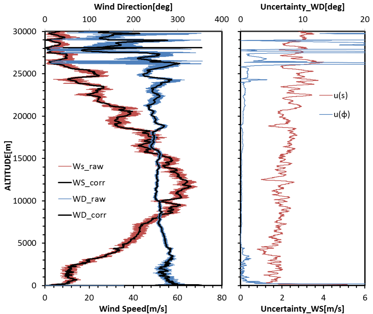
Figure 3.31: Vertical profiles of (left) wind speed and direction and (right) their uncertainties for the same sounding as shown in Figure 3.30.
