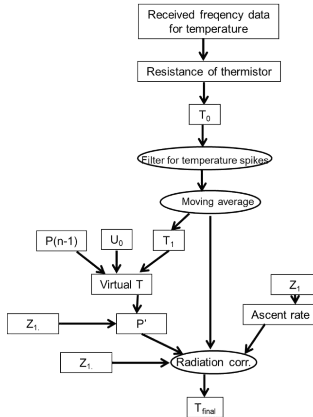
Figure 3.3: Schematic diagram of the processing steps and correction algorithms for the RS-11G and iMS-100 temperature measurements in the sounding software MGPS2. T_0 is the uncorrected temperature, U_0 is the uncorrected RH, P(n-1) is pressure one step before, P is preliminary pressure for radiation correction, Z_1 is the smoothed geopotential height, and T_{final} is the corrected, final temperature data.
