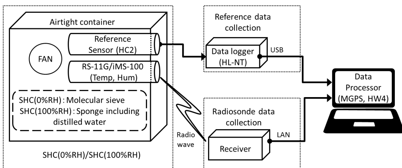
Figure F.1: Schematic diagram of the SHC system used at Tateno.
