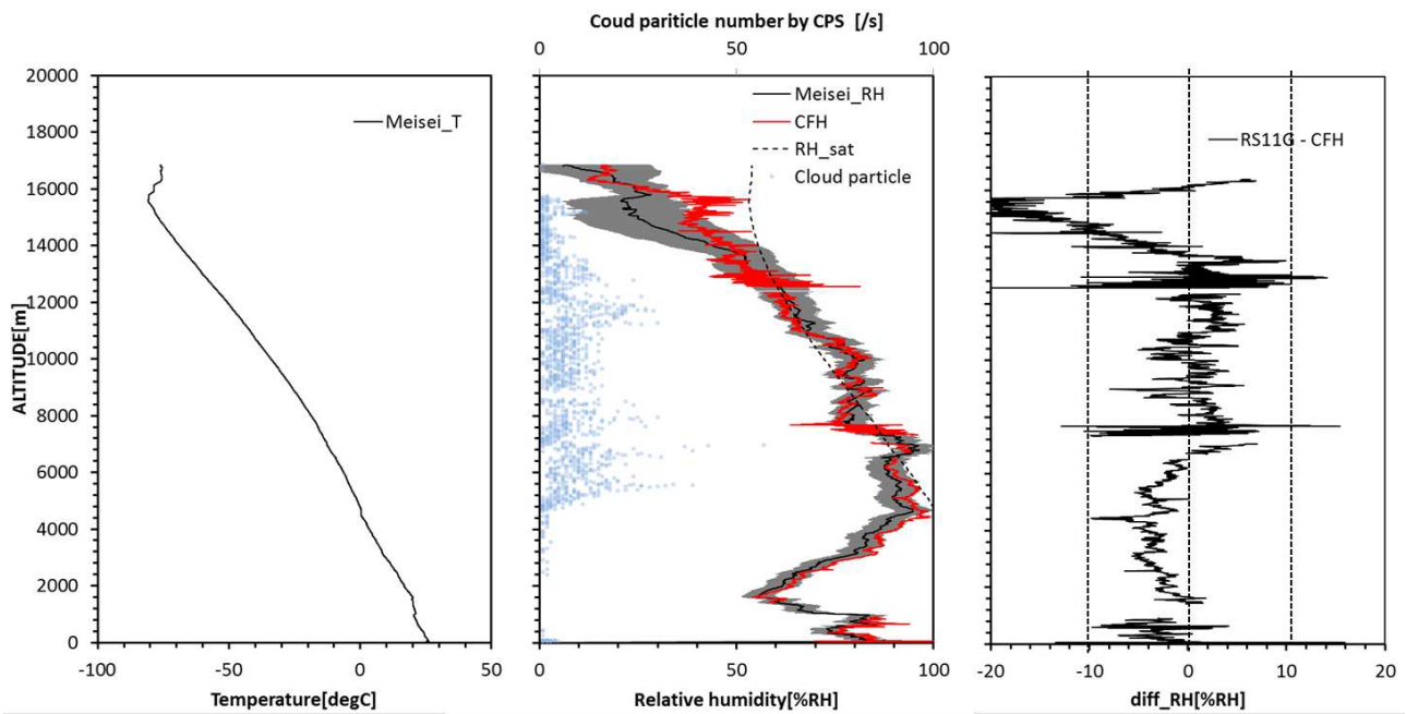
Figure 6.12: As for Figure 6.11, but for a nighttime simultaneous sounding of the RS-11G and CFH at Biak (1.1°S, 136.1°E), Indonesia at 18:00 LT on 23 February 2015. Blue dots in the center panel indicate the cloud particle number by the CPS sonde. This indicates that there are cloud layer between 5 km and 16 km. For this sounding, the balloon burst at ~17 km, around tropopause.
