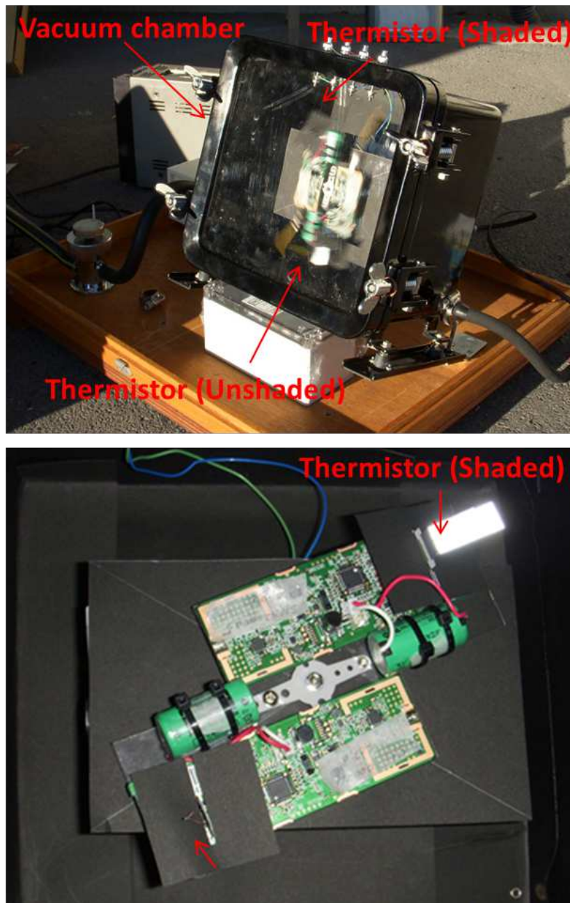
Figure 3.11: The experimental setup to evaluate the solar radiation correction model. See text for the details. Black-colored sheet with very low reflectivity is placed under the sensors and on the inner walls of the chamber to prevent solar light reflection to the sensors.
