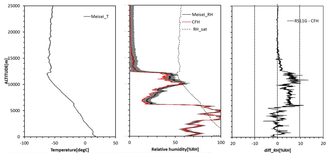
Figure 6.11: Profiles of (left) temperature, (center) RH, and (right) RH difference obtained from a day-time simultaneous sounding of the RS-11G and CFH at Lindenberg (52.21°N, 14.12°E), Germany at 14:00 LT on 7 October 2014. In the center panel, red curve is for CFH RH, black for RS-11G RH, and dotted for saturation RH. Gray shade is the measurement uncertainty calculated according to Section 3.2.4. In the right panel, the RH difference is calculated as RS-11G RH minus CFH RH.
