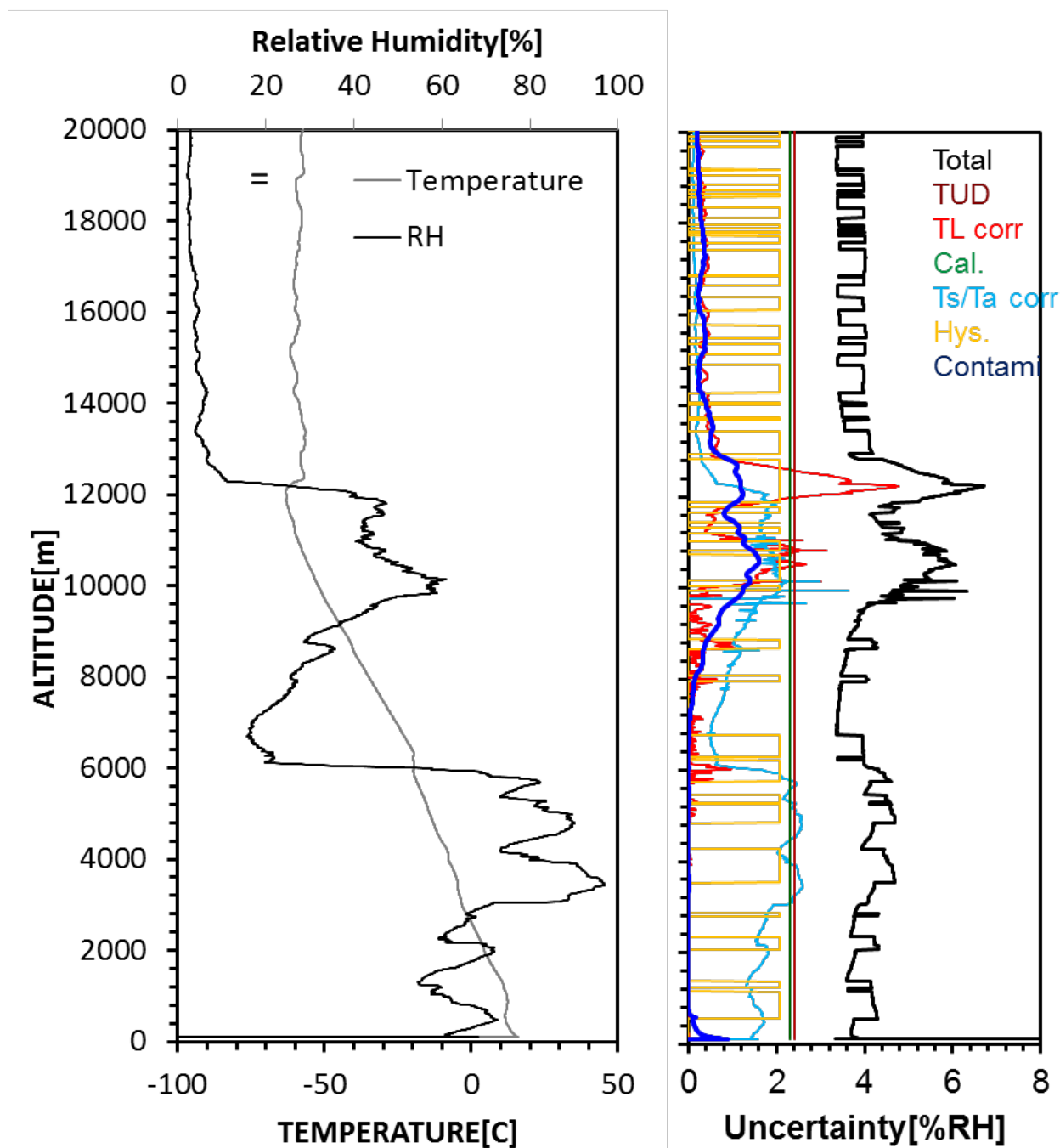
Figure 3.24: An example of the RS-11G RH measurement uncertainty profile at Lindenberg, Germany, launched at 14:00 LT on 7 October 2014. (Left) Obtained profiles of temperature and RH. (Right) Profiles of total uncertainty and individual components.
