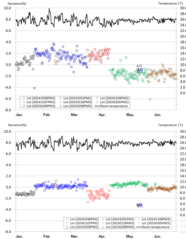
Figure 6.4: Time series of the RH deviation of radiosonde reading with respect to (top) 100 %RH and (bottom) 0 %RH created in the SHC (left axis) and the temperature conditions for the SHC check (right axis). Different marks indicate radiosondes from different lots.
