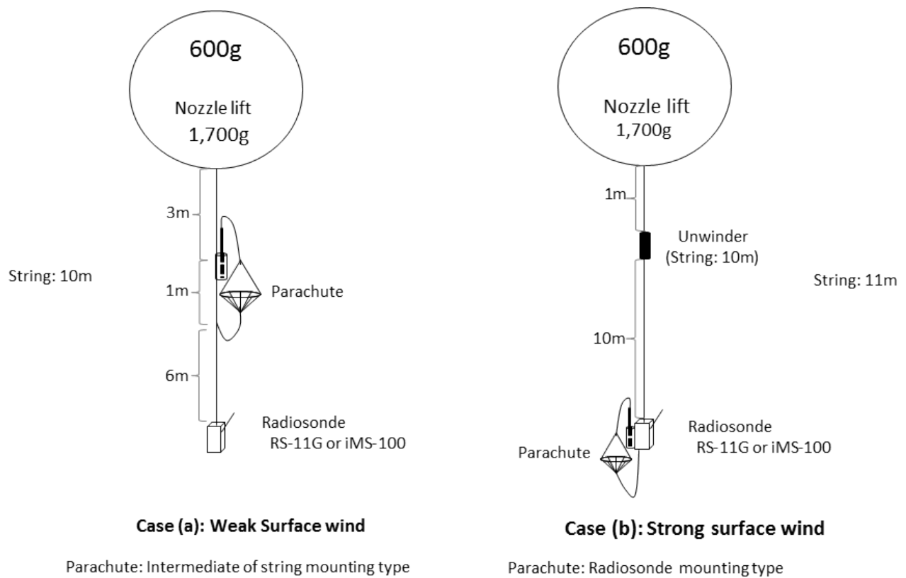
Figure 2.7: Flight configurations for (a) weak surface wind conditions and for (b) strong surface wind conditions (typically, >5 \text{ m s}^{-1} ) at Tateno.
