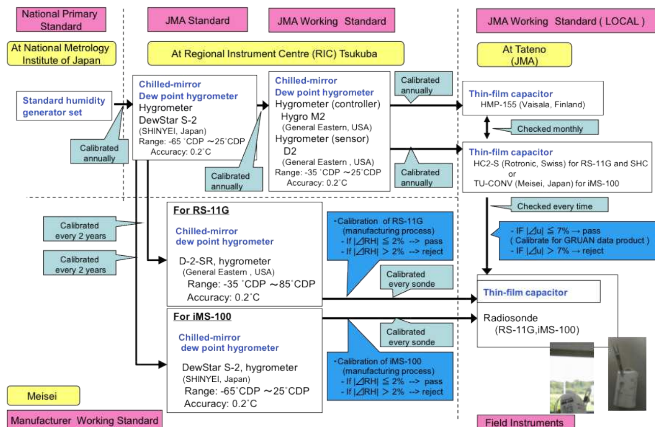
Figure 5.2: Traceability of the RH sensors on the RS-11G and iMS-100 radiosondes.
