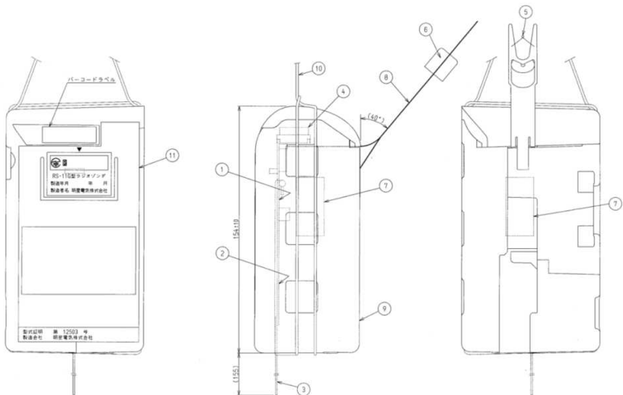
Figure 2.1: External view of the Meisei RS-11G radiosonde (unit: mm). 1: Processing unit and signal converting unit; 2: Transmitter; 3: Antenna; 4: GPS module; 5: Temperature sensor; 6: Relative humidity sensor with a cap; 7: Battery; 8: Sensor boom; 9: Styrofoam (EPS) case; 10: Rope; 11: Label; and 12: Interface.
