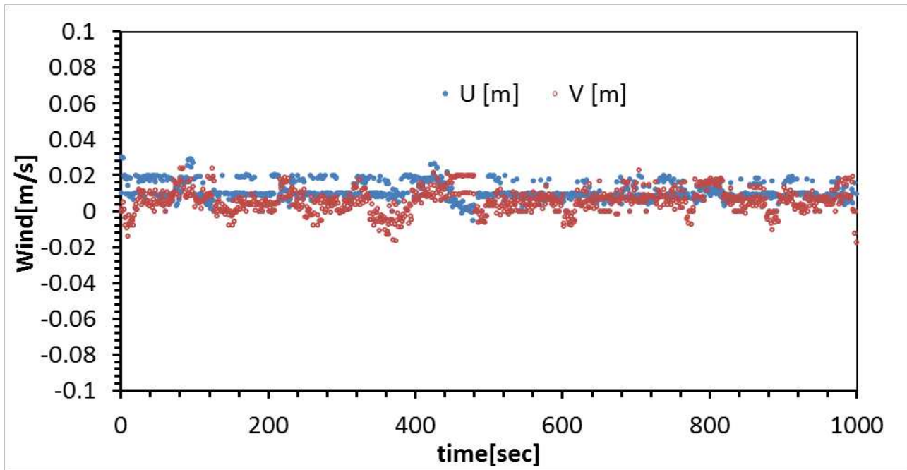
Figure 3.29: Variability of the GPS doppler speed data (i.e., U_0 and V_0 in Figure 3.28) under a static condition. The RS-11G radiosonde was placed on the ground at Moriya, Japan ( 35^\circ\text{N} , 140^\circ\text{E} ) on 22 December 2014.
