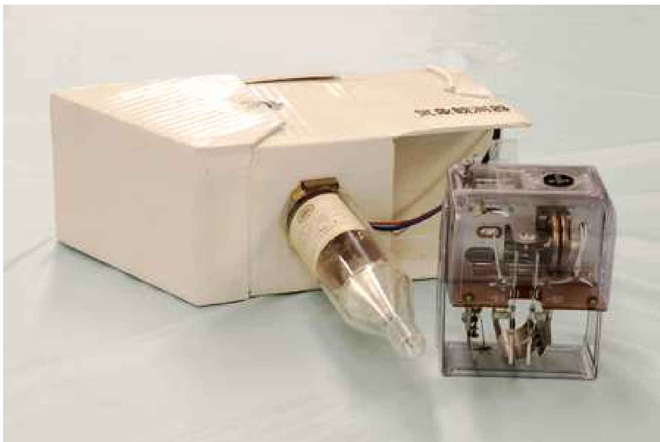
Figure 1.5: Photograph of the RS II-56 type rawinsonde. Before introduction of this type, different radiosonde manufacturers provided their own aneroid barometers. With this model, a unified aneroid barometer was introduced.
