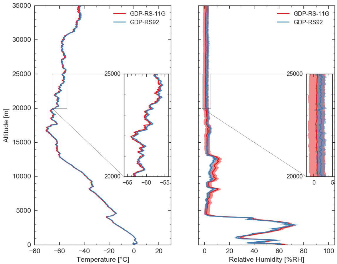
Figure 6.9: Comparison of temperature (left) and RH (right), with uncertainty range, between the RS-11G GDP (red) and RS92 GDP (blue) at Tateno, both launched at 00:00 UTC on 19 January 2015.
