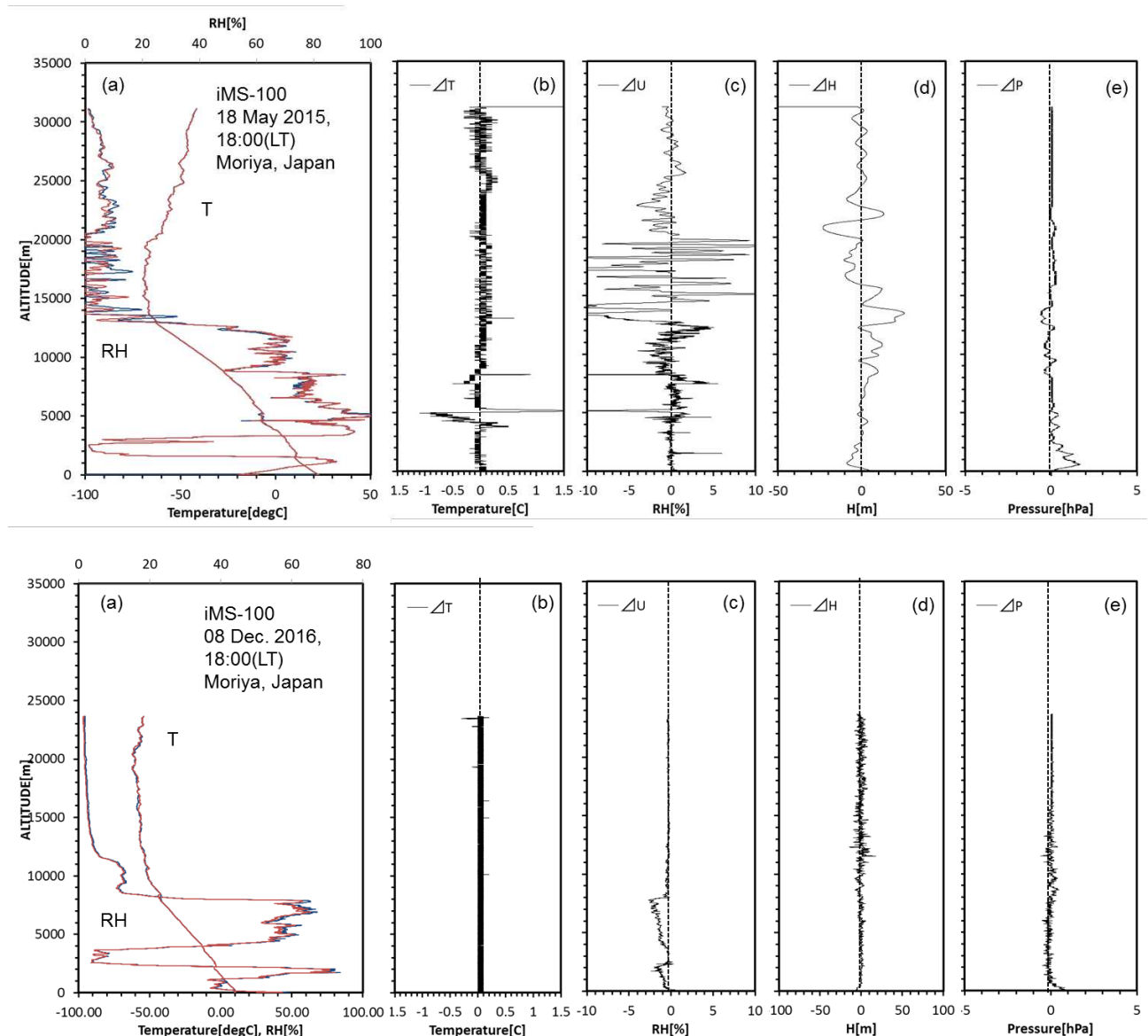
Figure 6.8: As for Figure 6.5, but for a nighttime multiple-payload sounding of two iMS-100 radiosondes. (Top) the sounding under cloudy conditions, launched at 18:00 LT on 18 May 2015, and (bottom) the sounding at 18:00 LT on 8 December 2016.
