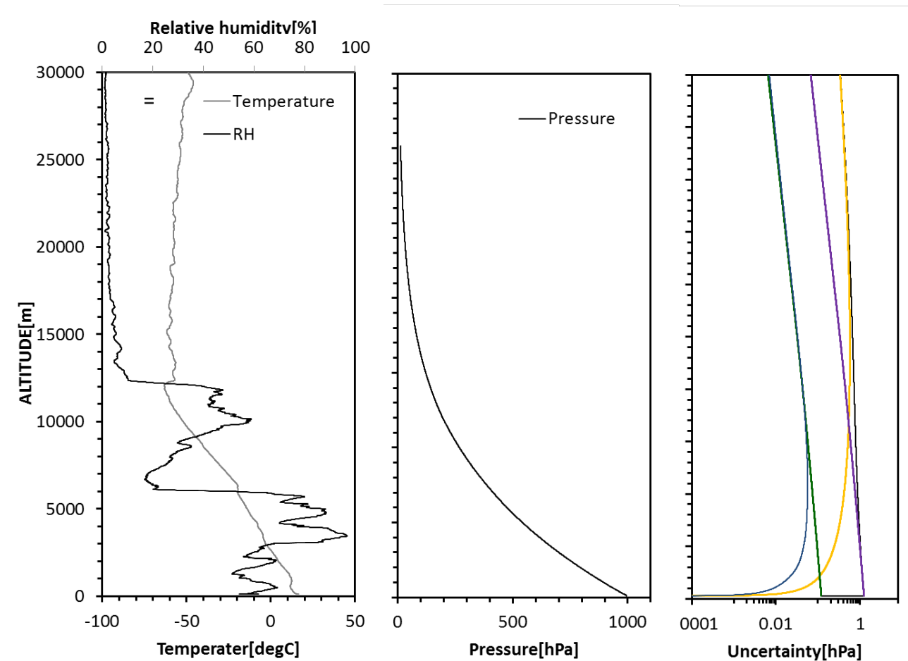
Figure 3.27: Example of the pressure uncertainty profile. (Left) Profiles of temperature and RH. (Middle) Profile of pressure. (Right) Profiles of total and individual uncertainty values ( k=2 ). Purple, blue, and yellow lines indicate the uncertainties from GPS-based geometric height (PDOP is assumed to be 1 throughout the profile), RH, and temperature measurements (taken from the profiles in Figure 3.14 and Figure 3.24), respectively. Green line indicates the surface pressure uncertainty. Black line indicates the total uncertainty.
