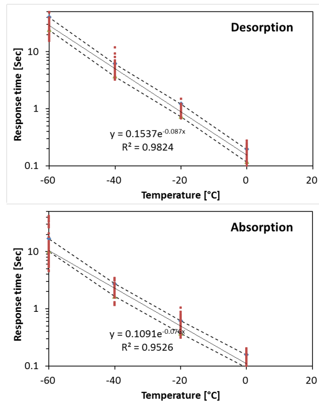
Figure 3.18: Results from laboratory experiments to determine the response time of the RS-11G and iMS-100 RH sensor at four temperatures (red dots). The ventilation speed in the thermostatic chamber was set to 5 \text{ m s}^{-1} . (Top) The response time for desorption conditions (i.e., for a stepwise change from wet to dry condition). (Bottom) The response time for absorption conditions (i.e., for a stepwise change from dry to wet condition). Solid lines indicate the averages of 69 measurement results at each temperature levels, and dotted lines indicate the deviation ( 2\sigma ).
