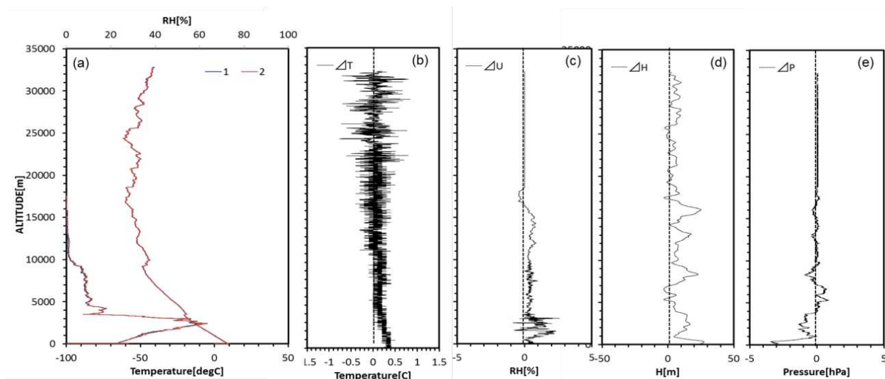
Figure 6.5: (a) Vertical profiles of temperature and RH obtained from a daytime multiple-payload sounding of two RS-11G radiosondes with a single balloon launched at Moriya (35.94°N, 140.00°E), Japan at 14:30 LT on 22 December 2014. Note the two curves are mostly overlapping for both temperature and RH. The profiles of differences in (b) temperature, (c) RH, (d) geopotential height, and (e) pressure.
