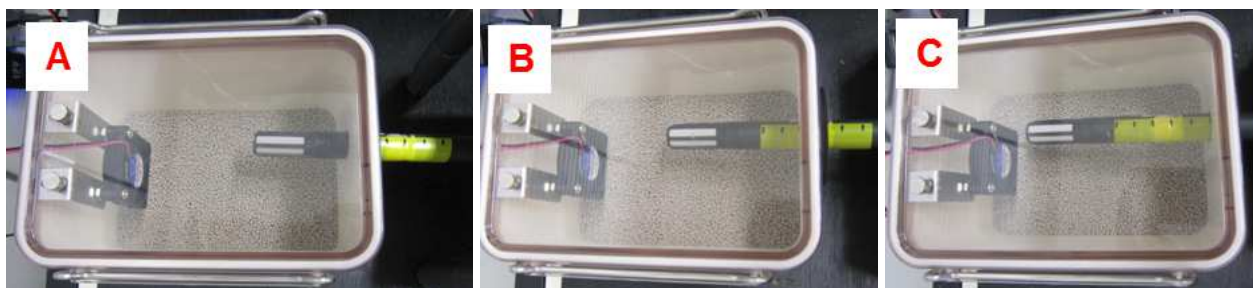
Figure F.11: The three different positions of the reference HC2 sensor in the SHC chamber. (A) The sensor top is located closer to the sensor insertion opening. (B) The sensor top is located around the center of the chamber. (C) The sensor top is located closer to the fan.
