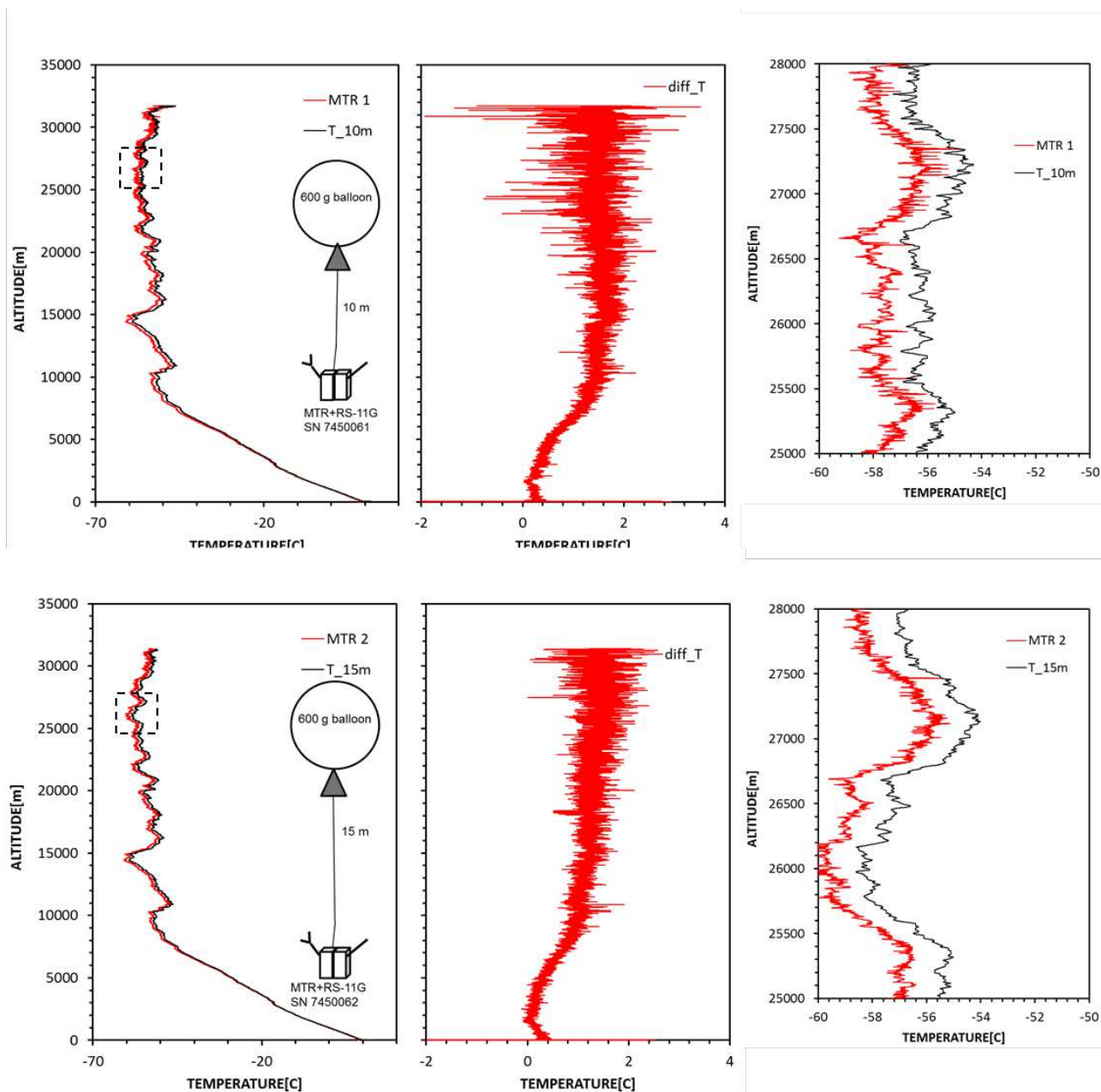
Figure 3.5: Temperature profiles obtained from two sets of MTR and RS-11G multiple payloads simultaneously launched at Tateno at 14:30 LT on 6 February 2014. One MTR-RS-11G payload is connected to a 600 g balloon with a 10 m string (top), and the other is with a 15 m string (bottom). (Left panels) Black lines indicate the RS-11G raw temperature profiles, and red lines indicate the MTR temperature. Note that the RS-11G temperature data is raw meaning that the heat spike filter and the solar radiation correction are not applied. (Center panels) Temperature difference of the RS-11G results with respect to the MTR results. (Right panels) A closer look at the region between 25 km and 28 km.
