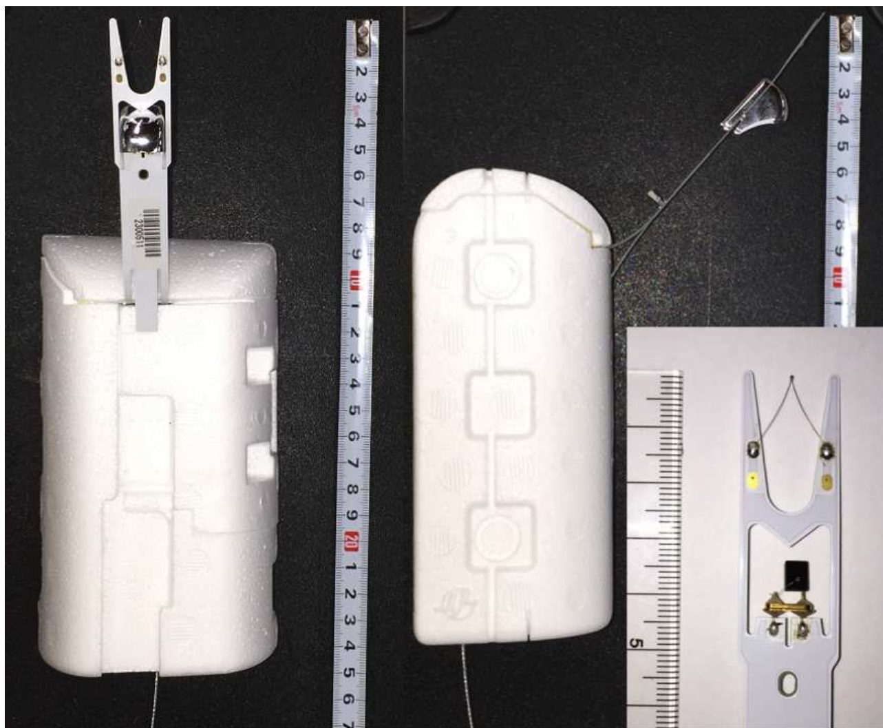
Figure 2.2: Photographs of the RS-11G radiosonde. The inset in lower right shows a magnified photograph of the sensor boom including the thermistor sensor and thin-film capacitive relative humidity sensor. The unit of the scales is cm.
