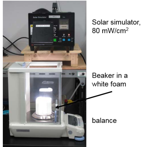
Fig. 8. Photograph of the measurement setup when the solar simulator is on.
