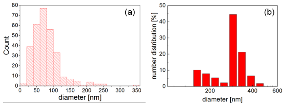
Fig. 6. (a) Size distribution of the silicon nanoparticles measured from the TEM images showing 300 particles in total. (b) Histogram of the silicon nanoparticle diameter in water by DLS measurement.
