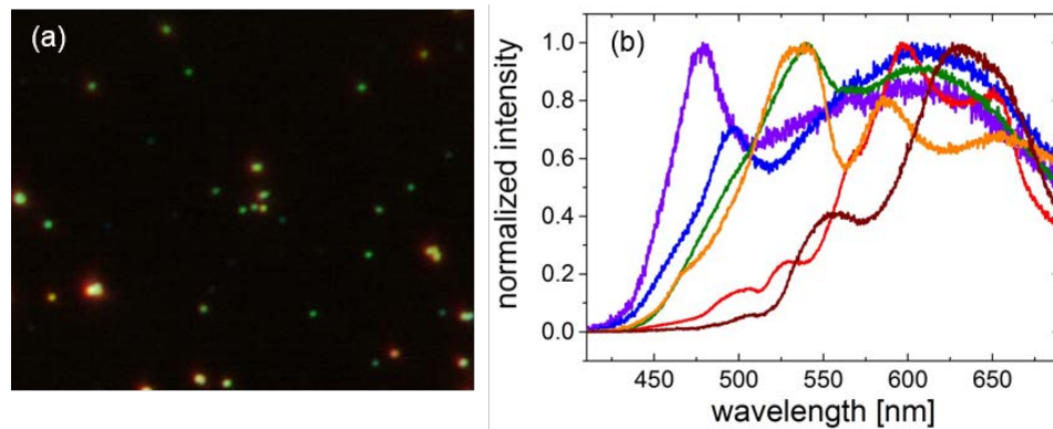
Fig. 7. (a) Dark field microscope image of the silicon nanoparticles on a cover glass. Different colors correspond to different sizes of the silicon nanoparticles. (b) Selected spectra of the backward scattering from the silicon nanoparticles on a cover glass. Each spectrum is normalized to its maximum.
