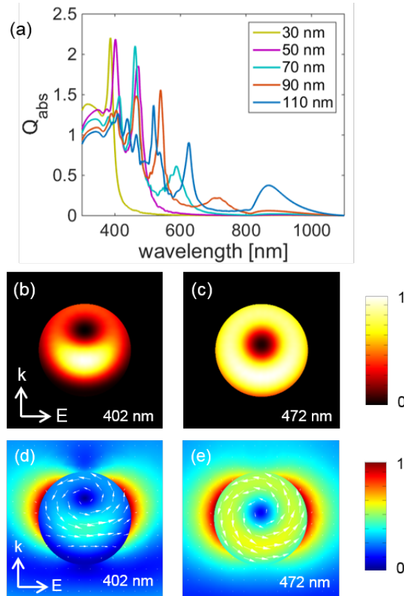
Fig. 1. (a) Absorption efficiencies of silicon nanospheres in water having different radii. (b-e) Cross sections of the simulated normalized absorption (b, c) and normalized electric field amplitude (d, e) in false color map for a 50-nm radius silicon nanosphere in water. Panels (b, d) and (c, e) are at 402 nm (second resonance) and 472 nm (first resonance), respectively. In the simulations, the incident light propagates from the bottom to the top and the electric field is polarized in horizontal direction.
