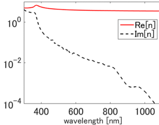
Fig. 4. Complex refractive index of silicon [27].
