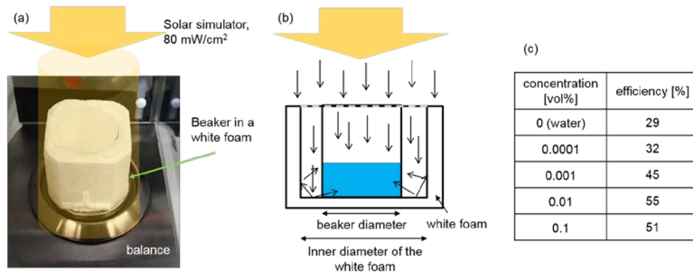
Fig. 9. (a) Photo of the experimental setup and (b) schematic drawing of the cross section of the setup. The thermos-coupler was removed when taking the photo. The beam size of the solar simulator was larger than the cross section of the white foam. Since the surface of the white foam is rough, scattered light can illuminate the nanofluid from the side. (c) Efficiencies of the silicon nanofluids.
