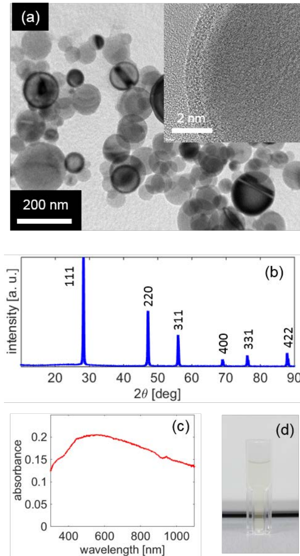
Fig. 2. (a) Bright field TEM image of the silicon nanoparticles. Inset shows the high-resolution TEM image. (b) Power XRD pattern of the silicon nanoparticles. (c) Extinction spectrum of the 0.001 vol% silicon nanoparticles in water in a 1-cm thick cell. The spectrum is normalized to pure water. (d) Photograph of silicon nanofluid at 0.001 vol%. The thickness of the plastic cell perpendicular direction to the photo is 1 cm.
