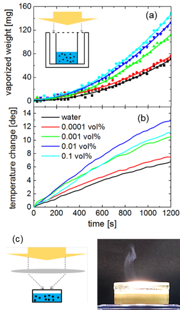
Fig. 3. Weight changes (a) and temperature changes (b) of the silicon nanofluids upon irradiation by a solar simulator. The legends for panel (a) is identical to panel (b). In panel (a), the measured data are represented by symbols and the solid lines are the fitted lines. The inset figure in panel (a) is a schematic of the setup and identical legends are used for panels (a) and (b). (c) Schematic of the setup with a focusing lens (left) and the photo of 0.1 vol% silicon nanofluid at the irradiation of \sim 800 mW/cm 2 from the solar simulator (right).
