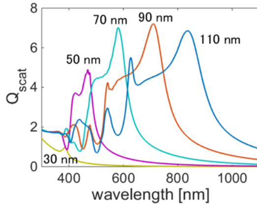
Fig. 5. Scattering efficiencies ( Q_{\text{scat}} ) of silicon nanospheres in water having different radii. The refractive index of silicon is taken from ref [27].
