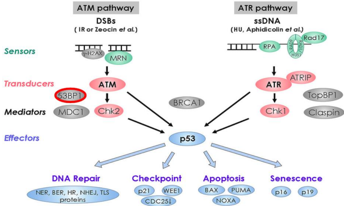
Figure 4. DNA damage response pathways in mammals (Yoshiyama et al. 2013).
