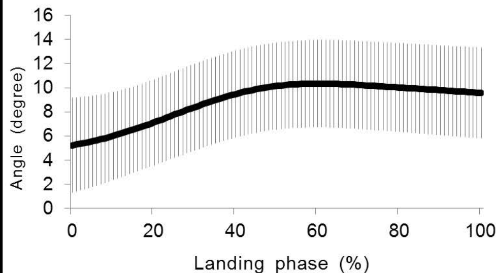
Rearfoot EVE(+)/INV(-)
