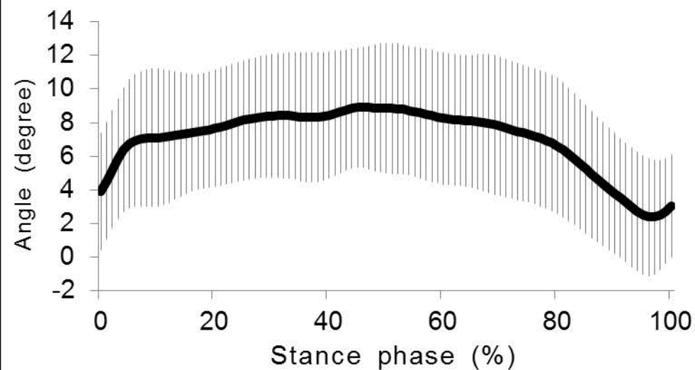
Rearfoot EVE(+)/INV(-)
