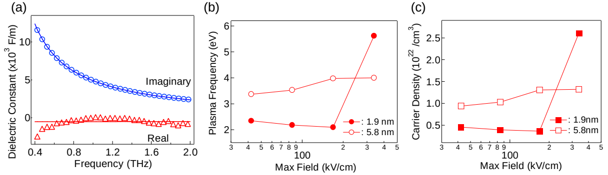
Fig. 3 (a) Complex dielectric constant of gold film with the thickness of 1.9 nm. Solid curves indicate the best-fit to the experimental data obtained by Drude analysis. (b) The estimated plasma frequencies and (c) the carrier densities of the Au films with the thicknesses of 1.9 and 5.8 nm as a function of maximum terahertz electric field.
