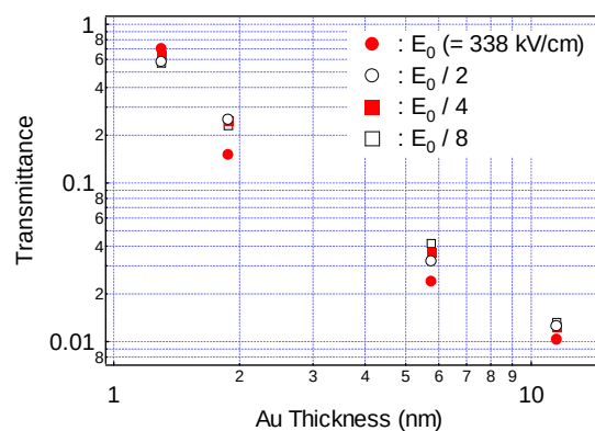
Fig. 2 Transmittance of terahertz waves as a function of the Au film thickness with several terahertz intensities.
