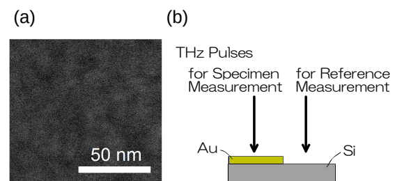
Fig. 1 (a) SEM image of Au thin film surface with 1.9 nm thickness. (b) Side view of the specimen for measuring terahertz transmittance of the reference and signal.
