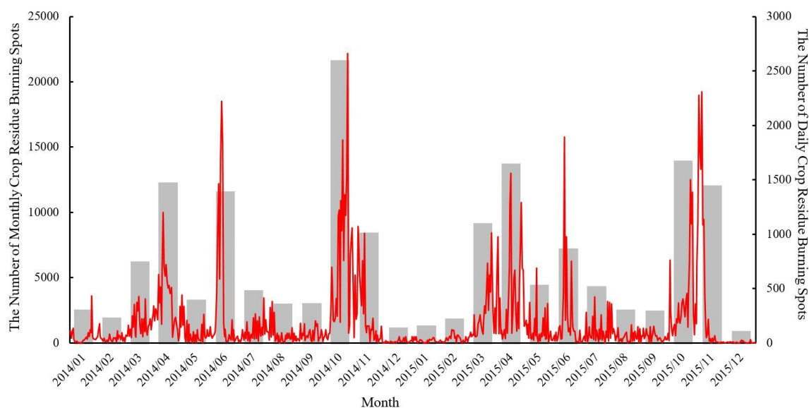
Fig. 2. The daily (red line) and monthly (gray column) number of crop residue burning spots in China.
