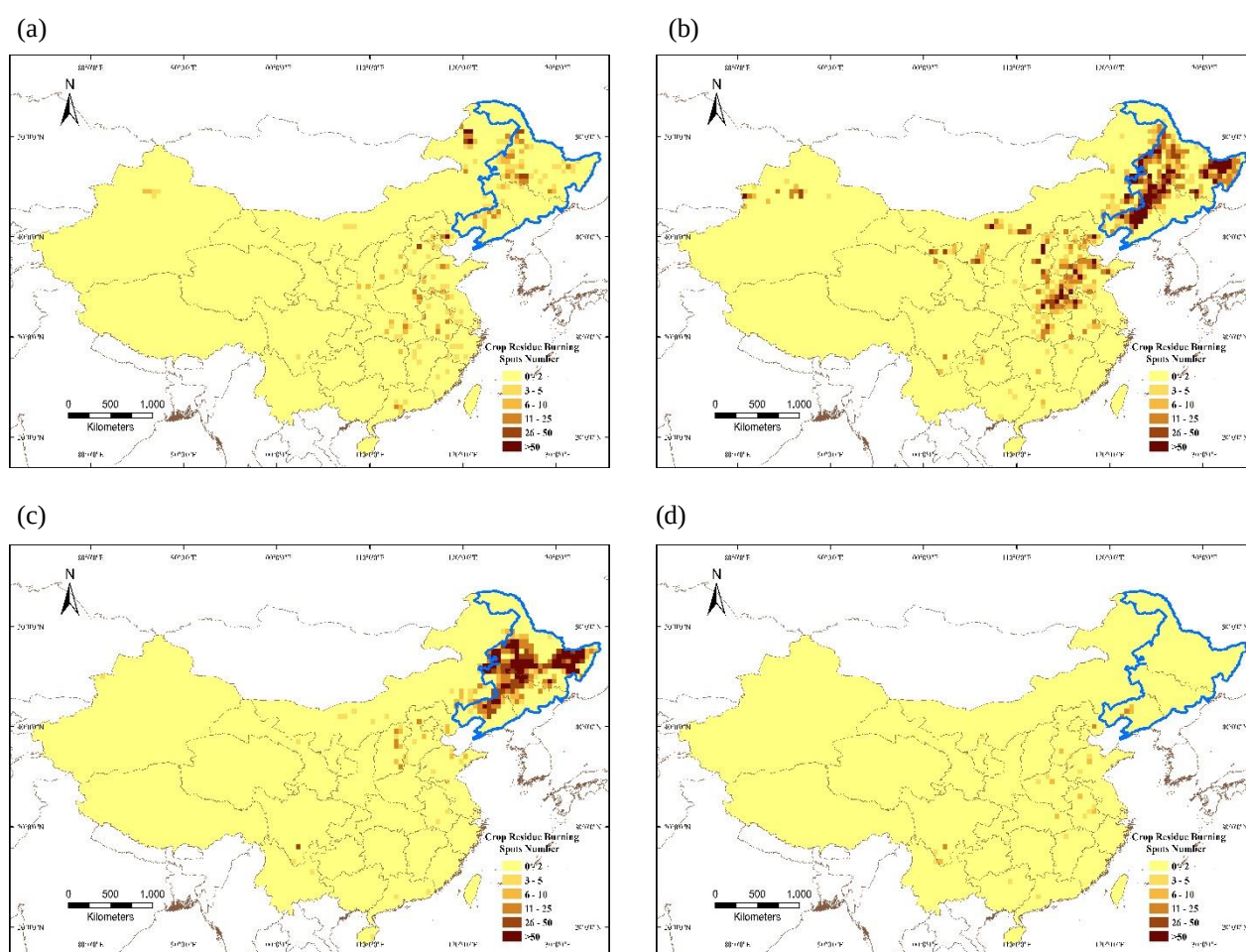
Fig. 9. Spatial distribution of crop residue burning from September to December in 2015: September (a); October (b); November (c); December (d) (blue line is the boundary of the 3 provinces in China's northeast).
