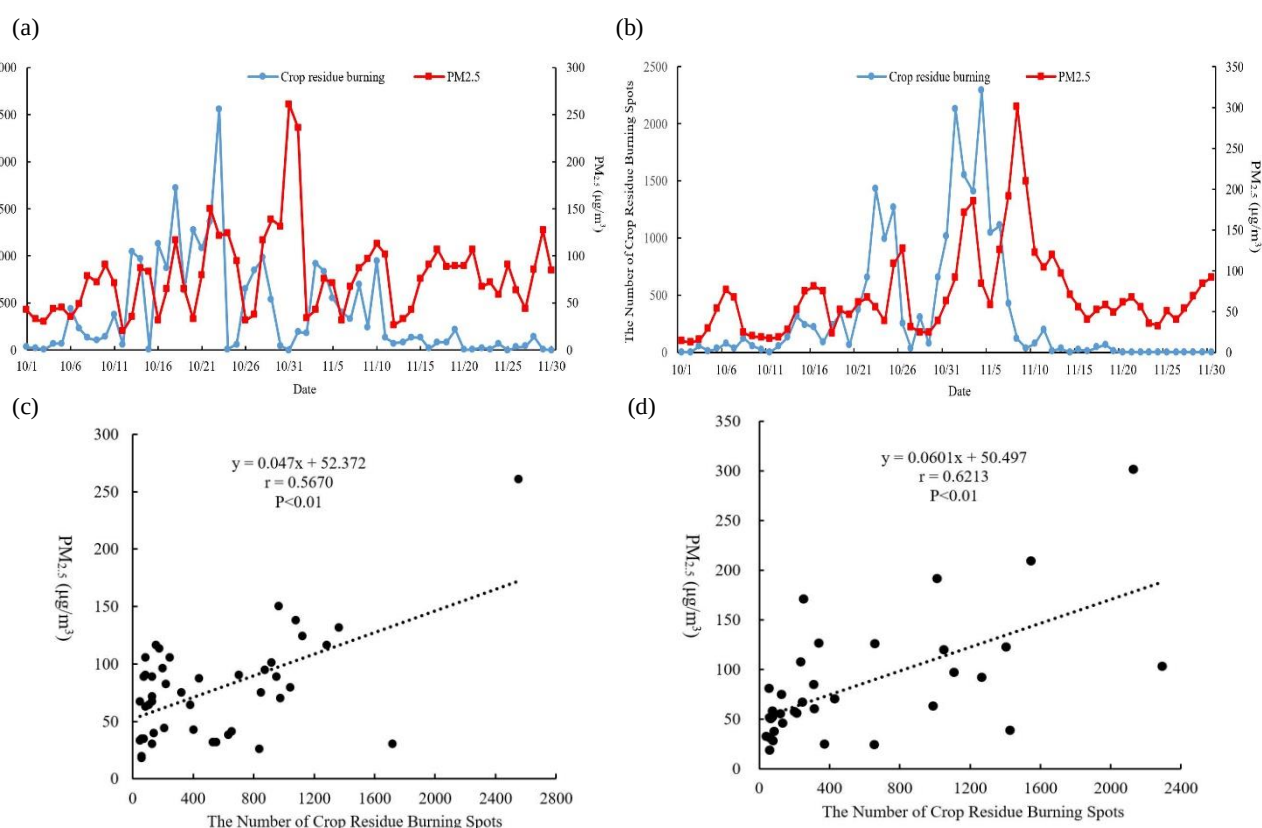
Fig. 7. The number of crop residue burning spots and PM 2.5 in China's northeast in October and November: 2014(a); 2015(b). And the correlation in China's northeast between the number of autumn crop residue burning spots and PM 2.5 from 8 days later in October and November 2014(c) and 7 days later in October and November 2015(d).
