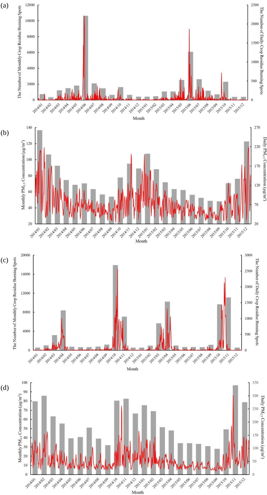
Fig. 3. The daily (red line) and monthly (gray column) data of crop residue burning spots in China's middle-east (a) and China's northeast (c) and PM 2.5 concentration in China's middle-east (b) and China's northeast (d).
