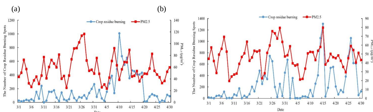
Fig. 4. The number of crop residue burning spots and PM_{2.5} of China's northeast in March and April: 2014(a); 2015(b).
