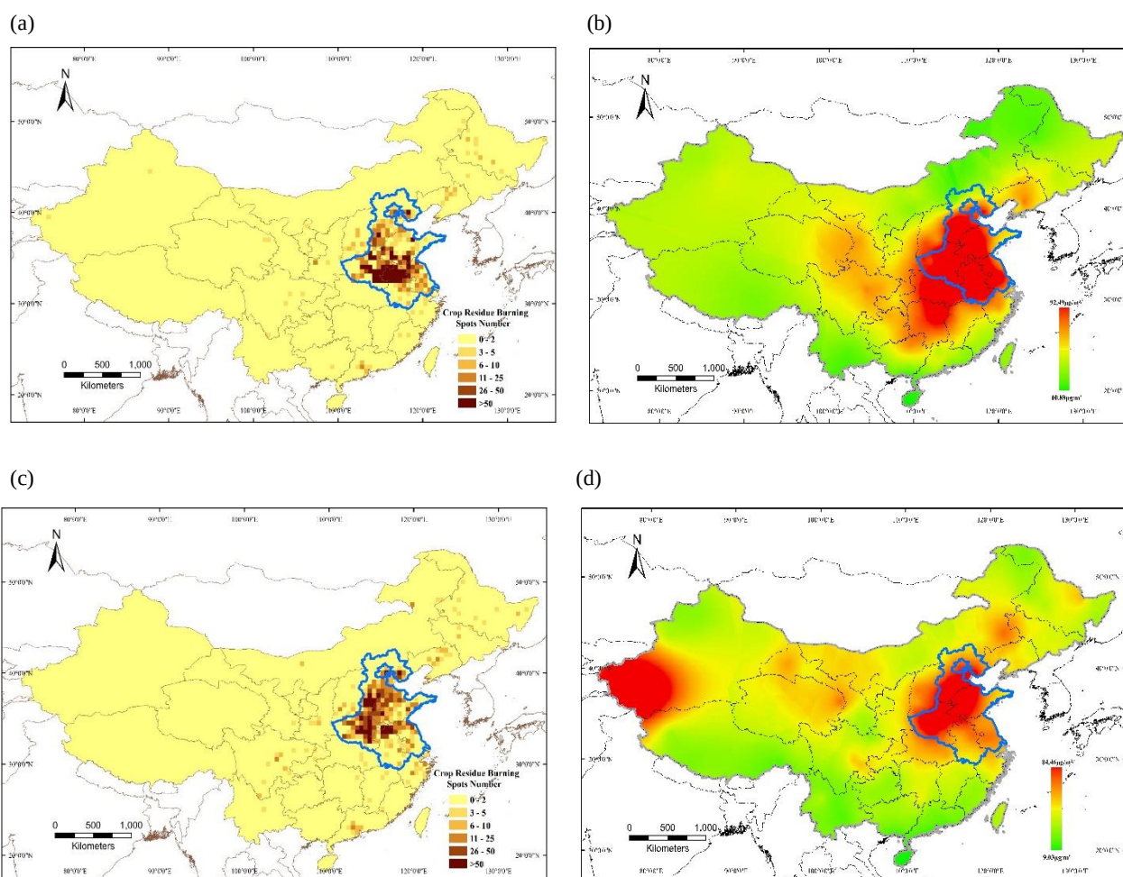
Fig. 6. Spatial distribution of crop residue burning and PM_{2.5} in China in June (blue line is the boundary of the five provinces in China's middle-east): crop residue burning in June 2014(a); crop residue burning in June 2015(c); PM_{2.5} distribution in June 2014(b); PM_{2.5} distribution in June 2015(d).
