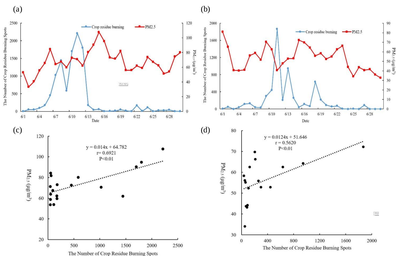
Fig. 5. The number of crop residue burning spots and PM 2.5 of China's middle-east in June: 2014(a); 2015(b). And the correlation between the number of crop residue burning spots and PM 2.5 measured 4 days later: June 2014(c); June 2015(d).
