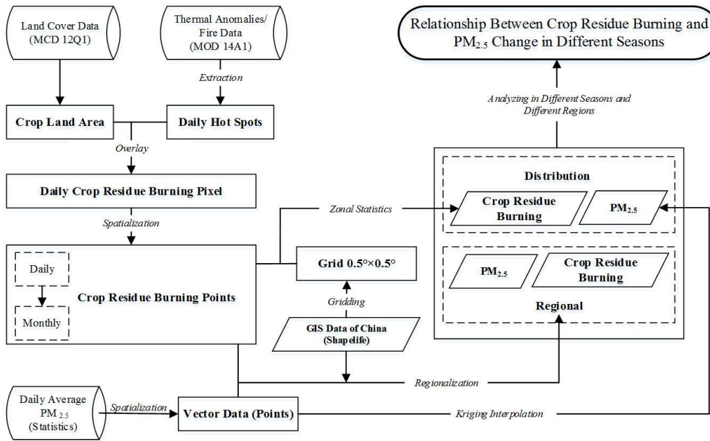
Fig. 1. Flow chart of obtaining crop residue burning data and PM 2.5 data.
