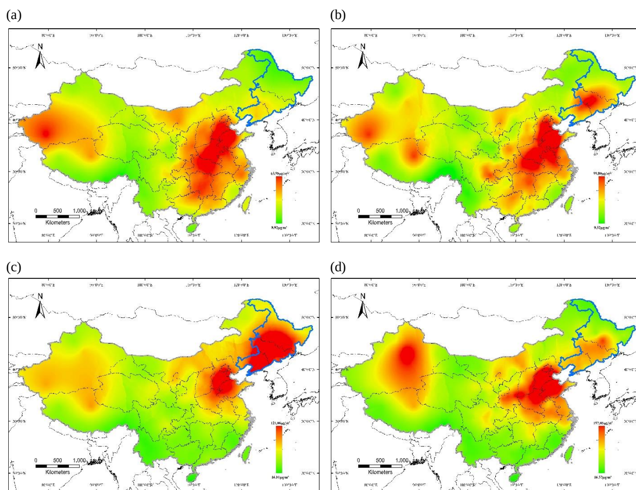
Fig. 8. Spatial distribution of PM_{2.5} from September to December in 2015: September (a); October (b); November (c); December (d) (blue line is the boundary of the 3 provinces in China's northeast).
