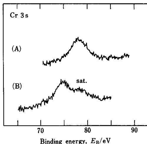
Fig. 2 X-Ray photoelectron spectra of Cr 3s for (A) LaCrO 4 and (B) LaCrO 3 . Sat. indicates a multiplet satellite.
