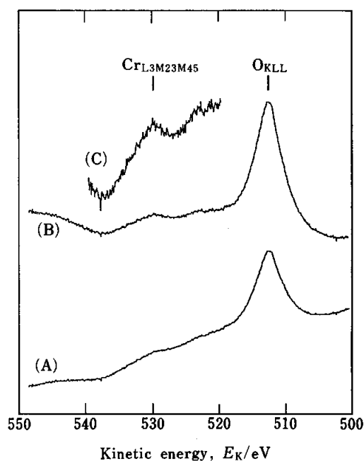
Fig. 3 X-Ray photoelectron spectra of Cr LMM and O KLL region for LaCrO 4 . (A) original spectrum, (B) (A) after linear background subtraction, and (C) enlarged Cr LMM region of (B).
