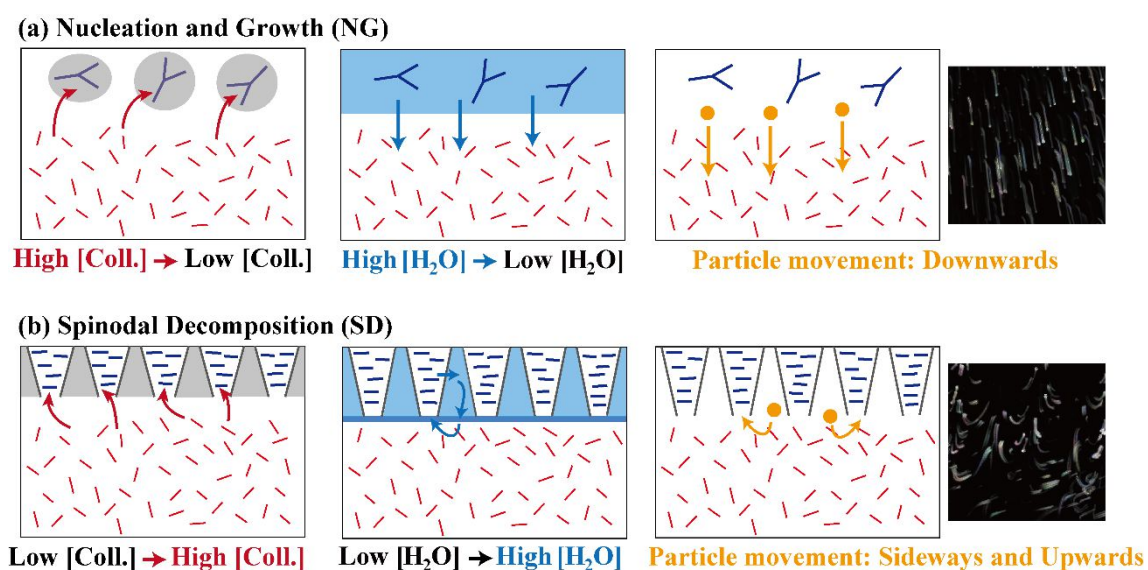
Figure 6.2 The movement of collagen, water, and particles during phase separation. (a) In nucleation and growth (NG) phase separation, molecules move from high concentration regions to low concentration regions. In a collagen solution, collagen molecules move towards the nuclei, whereas water molecules move away from the nuclei. (b) In spinodal decomposition (SD) phase separation, molecules move from low concentration regions to high concentration regions. In a collagen solution, collagen molecules move towards the collagen matrix region and not the channel region. On the other hand, the movement of water is in a convective movement from the matrix to the channel, then back up towards the matrix. The movement of the particles appear to coincide with those of the water molecules, and not with those of the collagen molecules, thus suggesting that the movement of the particles are driven by that of water during phase separation.
