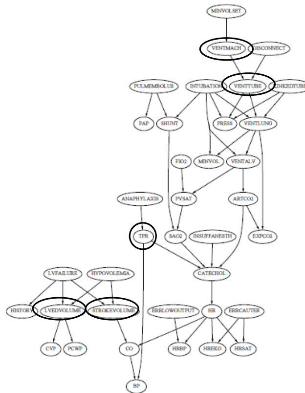
Figure 5.3 Example of ALARM
