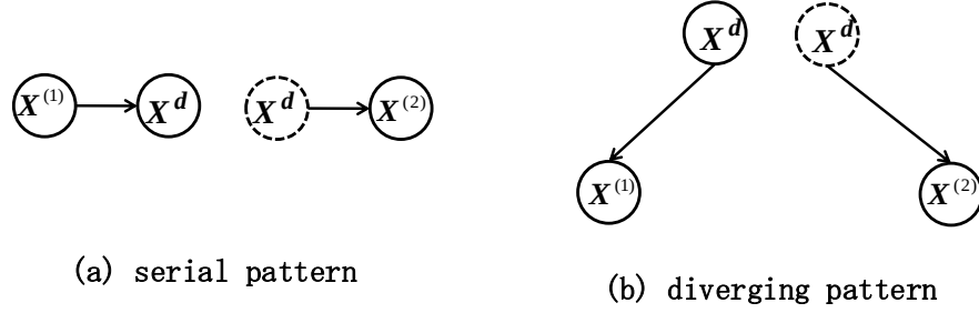
Figure 5.1 Partitioning with d -separations.
