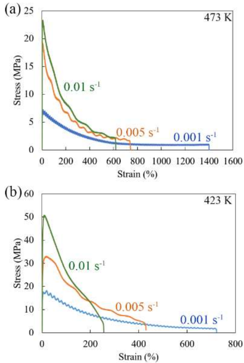
Fig. 6.4 Engineering stress-strain curves of the ERES specimens tested in tension at 0.001, 0.005 and 0.01 s -1 at (a) 473 K and (b) 423 K
