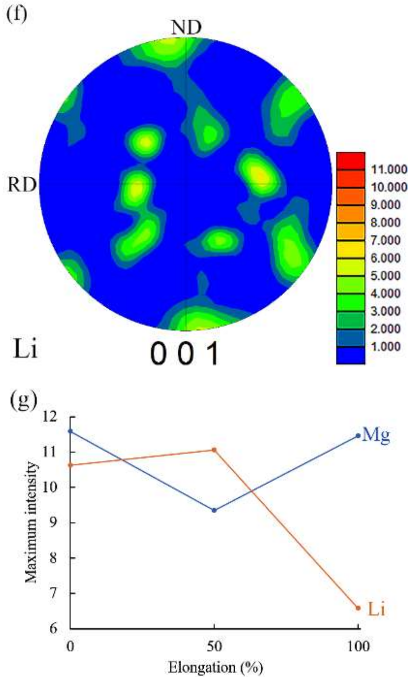
Fig. 6.13 The (0 0 0 1) pole figures of \alpha phase in the ERED specimens after tensile elongations of (a) 0%, (b) 50% and (c) 100% at 473 K at 0.001 \text{ s}^{-1} ; the (0 0 1) pole figures of \beta phase in the ERED specimens after tensile elongations of (d) 0%, (e) 50% and (f) 100% at 473 K at 0.001 \text{ s}^{-1} ; and (g) the change of the maximum intensity of the pole figures.
