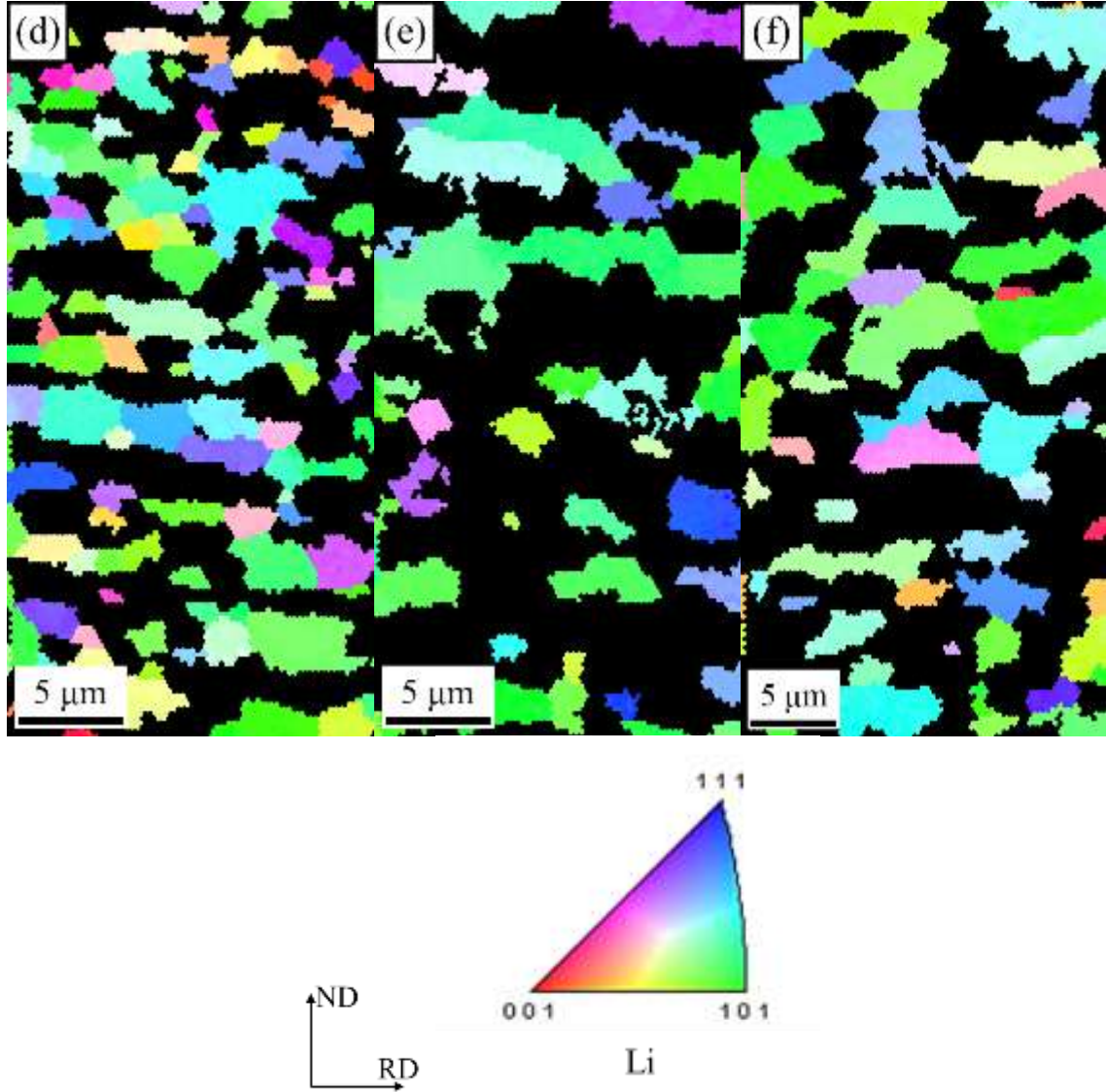
Fig. 6.10 IPF maps of the \alpha phase in the ERES specimens after different levels of tensile elongation of (a) 0%, (b) 50% and (c) 100% at 473 K at 0.001 \text{ s}^{-1} , and IPF maps of the \beta phase in the ERES specimens after different levels of tensile elongation of (d) 0%, (e) 50% and (f) 100% at 473 K at 0.001 \text{ s}^{-1} .
