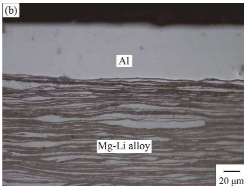
Fig. 3.3 (a) Longitudinal section of the as-rolled Al-coated Mg-Li alloy sheet, and (b) interface between Al coating and Mg-Li alloy substrate in the longitudinal section. The rolling direction corresponds to the traverse direction of the figures.
