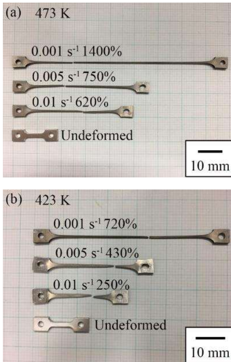
Fig. 6.5 Appearances of ERER specimens after tensile tests at 0.001, 0.005 and 0.01 s -1 at (a) 473 K and (b) 423 K.
