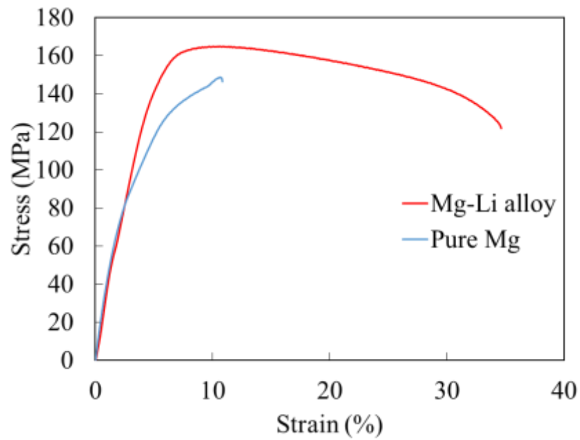
Fig. 4.2 Nominal stress-strain curves of Mg-Li alloy and pure Mg sheets at room temperature at 0.001 \text{ s}^{-1} .
